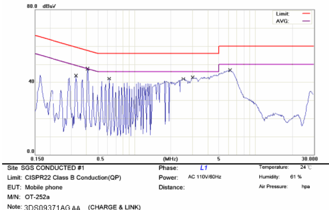
Conducted Emission Measurement
