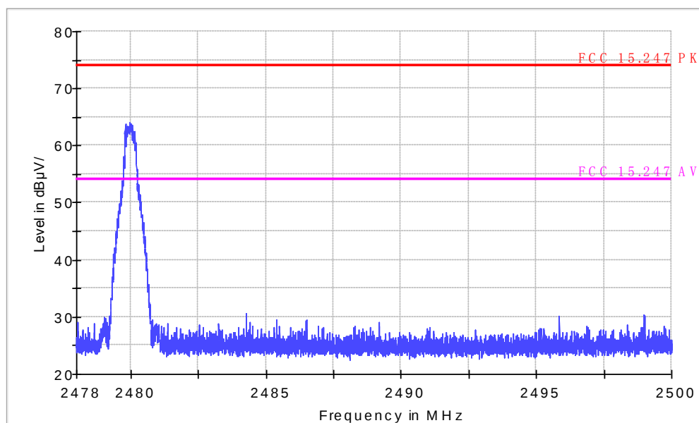
FCC Electric Field Strength 2.4GHz Bandedge-PK
