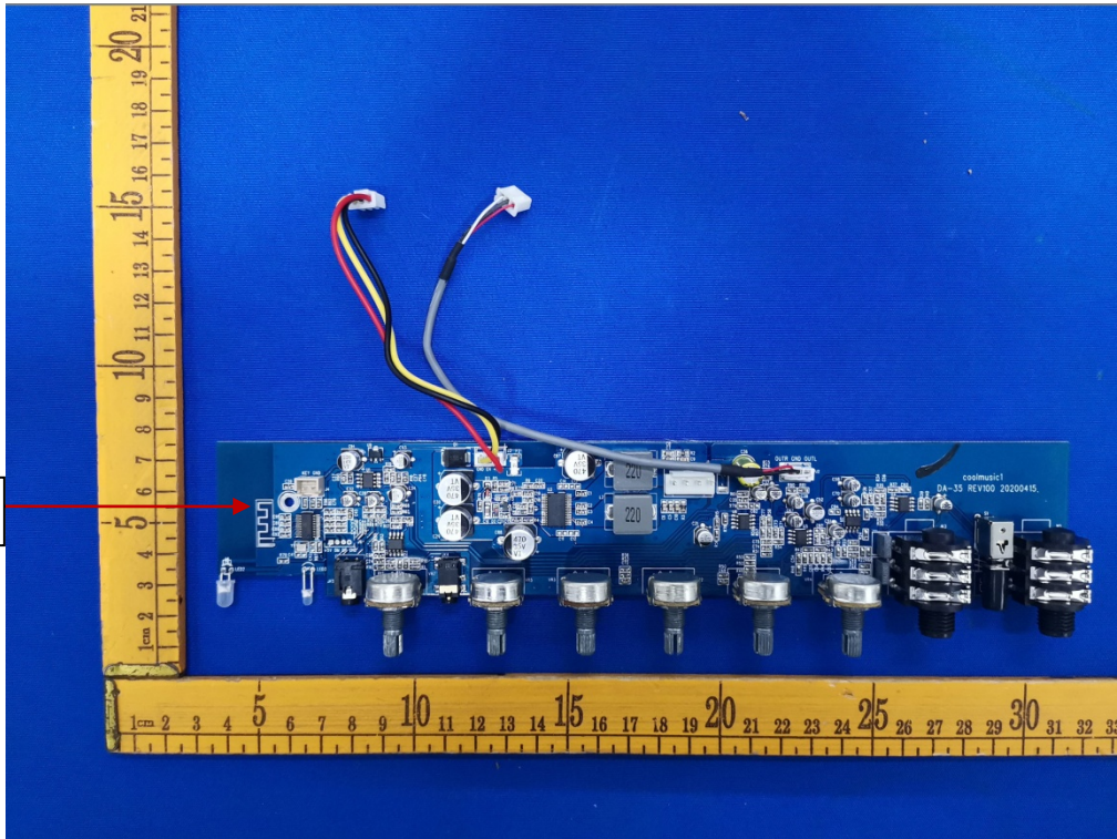
BT Antenna
