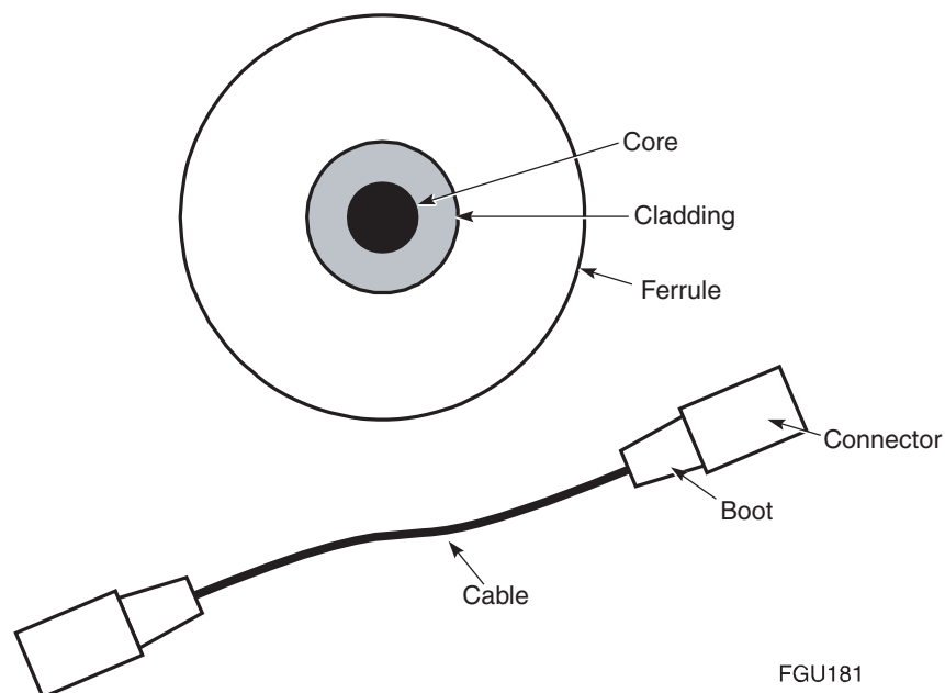
Figure 18 Parts of a fiber optic cable
