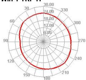
Wifi 1 TRP H
