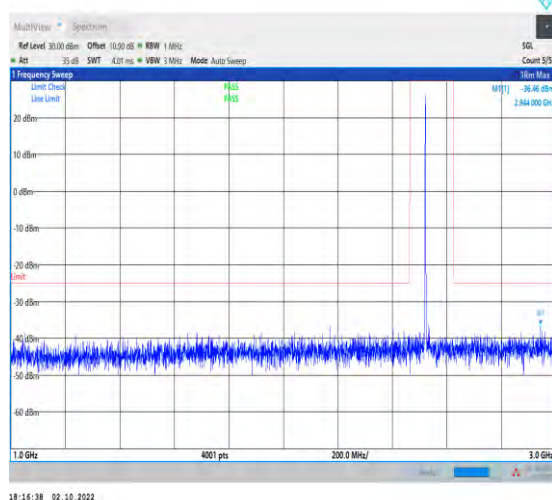
1-N7--15-50-H-1-DFT-PI2BPSK-Inner_1RB_Left-1@ 1-1000-3000-Ant1-2944.00--36.46--25-PASS
