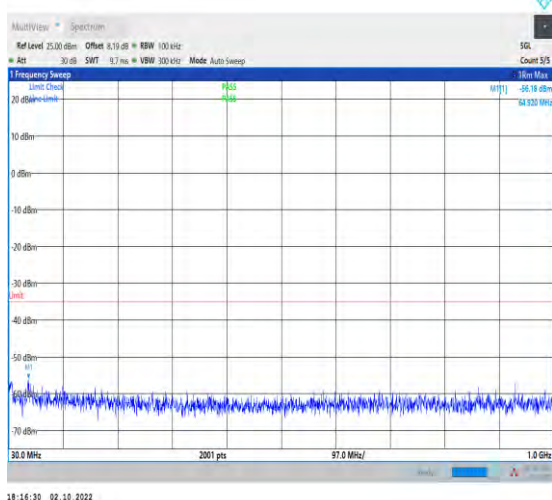
1-N7--15-50-H-1-DFT-PI2BPSK-Inner_1RB_Left-1 @ 1-30-1000-Ant1-64.92--56.18--35-PASS
