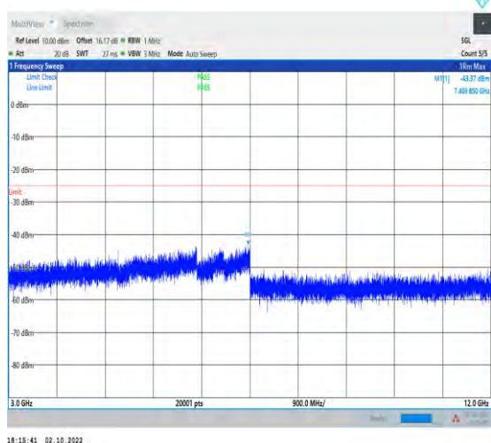
1-N7--15-50-M-1-DFT-PI2BPSK-Inner_1RB_Left-1 @ 1-3000-12000-Ant1-7469.85--43.37--25-PASS
