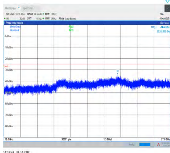
1-N7--15-50-M-1-DFT-PI2BPSK-Inner_1RB_Left-1@ 1-12000-27000-Ant1-22242.50--34.40--25-PASS
