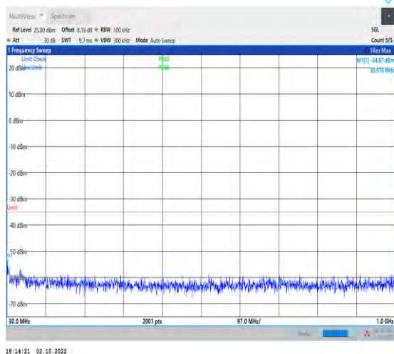
1-N7--15-50-L-1-DFT-PI2BPSK-Inner_1RB_Left-1@ 1-30-1000-Ant1-30.97--54.87--35-PASS
