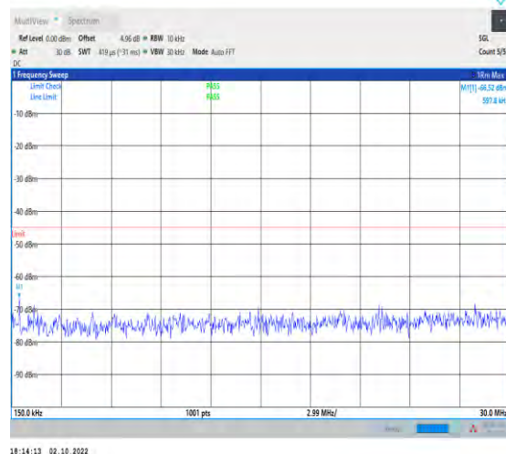
1-N7--15-50-L-1-DFT-PI2BPSK-Inner_1RB_Left-1@1 -0.15-30-Ant1-0.60--66.52--45-PASS
