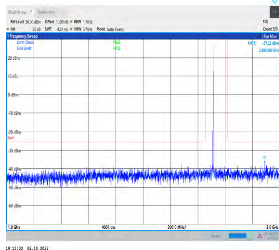
1-N7--15-50-M-1-DFT-PI2BPSK-Inner_1RB_Left-1@ 1-1000-3000-Ant1-2890.50--37.22--25-PASS
