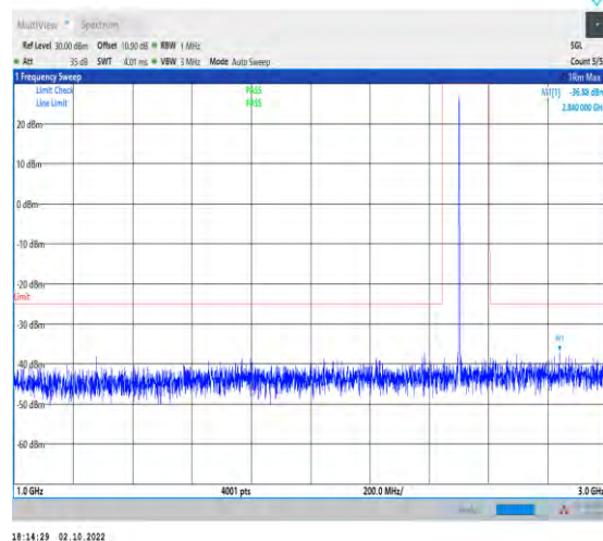
1-N7--15-50-L-1-DFT-PI2BPSK-Inner_1RB_Left-1@1 -1000-3000-Ant1-2840.00--36.88--25-PASS
