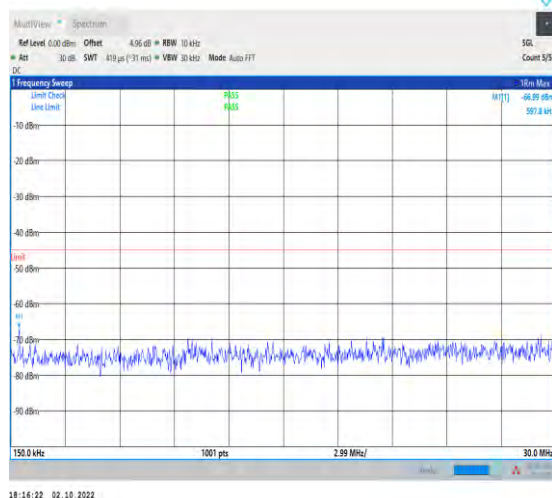
1-N7--15-50-H-1-DFT-PI2BPSK-Inner_1RB_Left-1@ 1-0.15-30-Ant1-0.60--66.99--45-PASS
