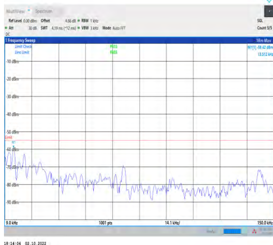
1-N7--15-50-L-1-DFT-PI2BPSK-Inner_1RB_Left-1@ 1-0.009-0.15-Ant1-0.01--59.42--55-PASS
