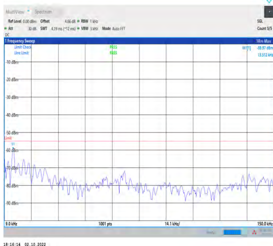
1-N7--15-50-H-1-DFT-PI2BPSK-Inner_1RB_Left-1 @ 1-0.009-0.15-Ant1-0.01--59.97--55-PASS
