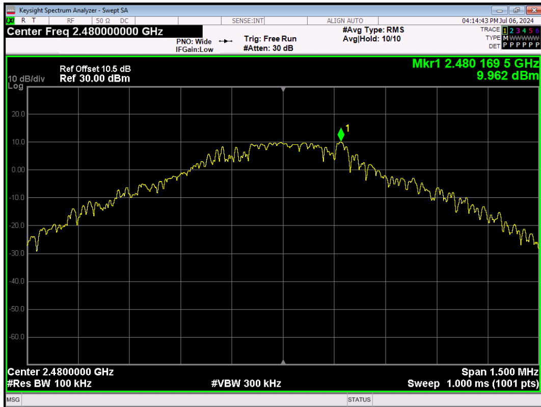
DH5-Ant1-2480-0~Reference-PASS
