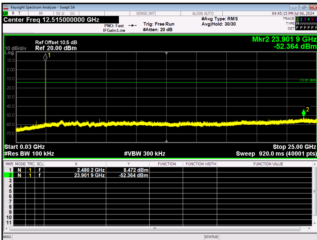
3DH5-Ant1-2480-30~25000-PASS
