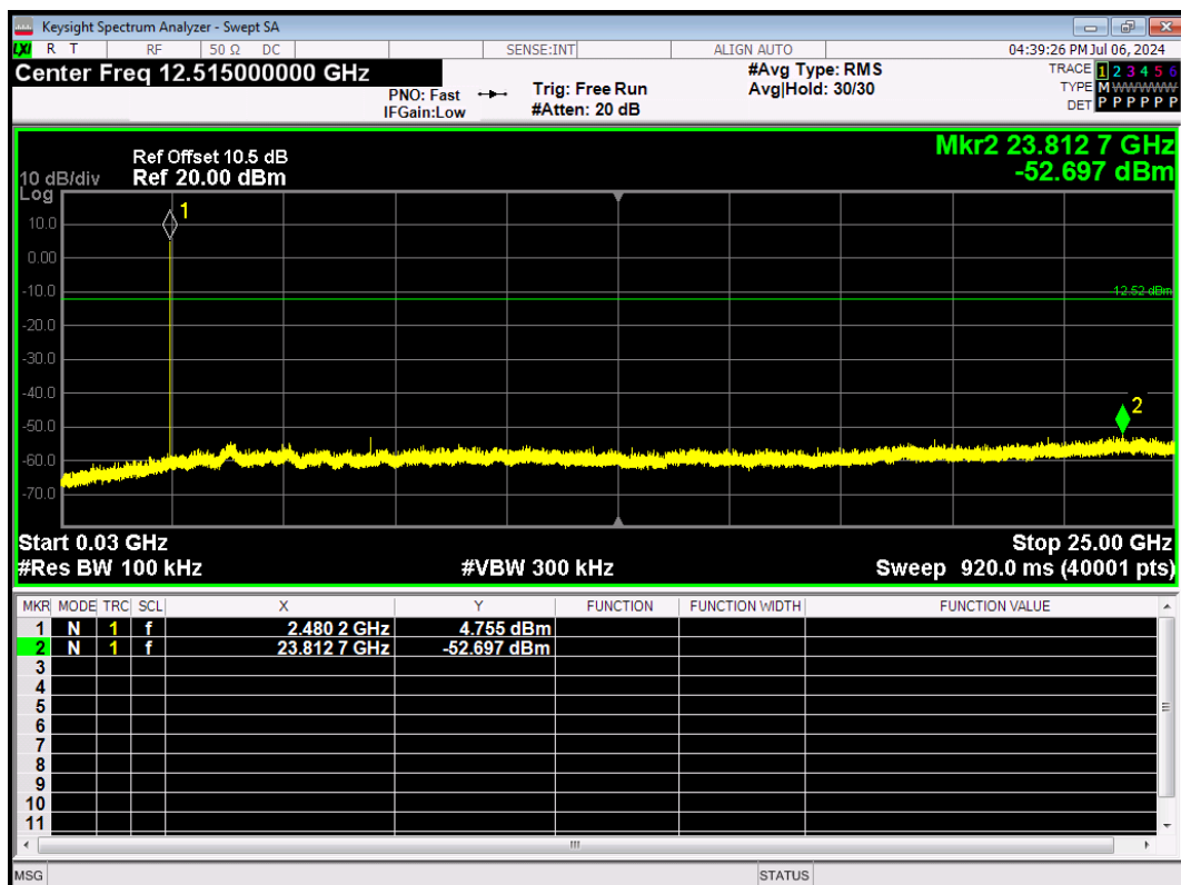
2DH5-Ant1-2480-30~25000-PASS
