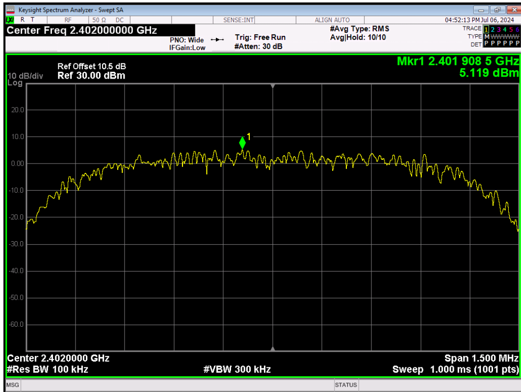
3DH5-Ant1-2402-0~Reference-PASS
