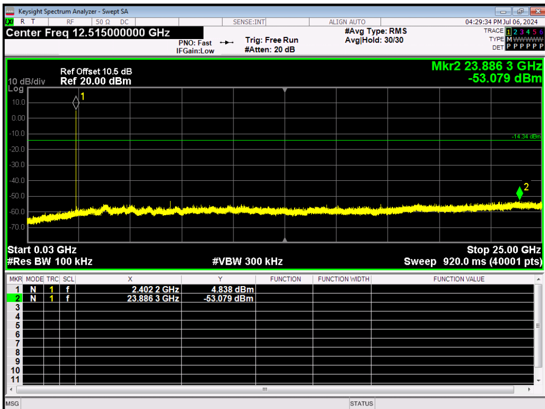
2DH5-Ant1-2402-30~25000-PASS
