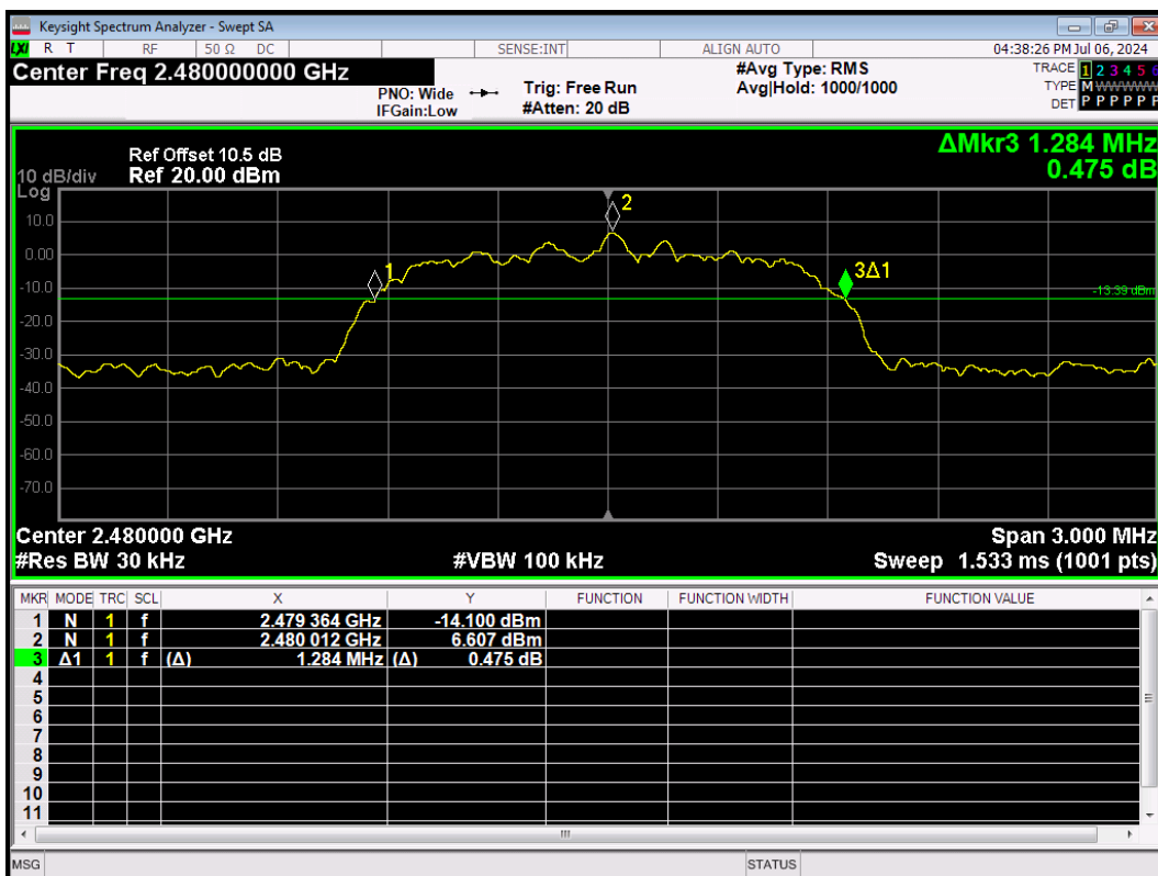
2DH5-Ant1-2480
