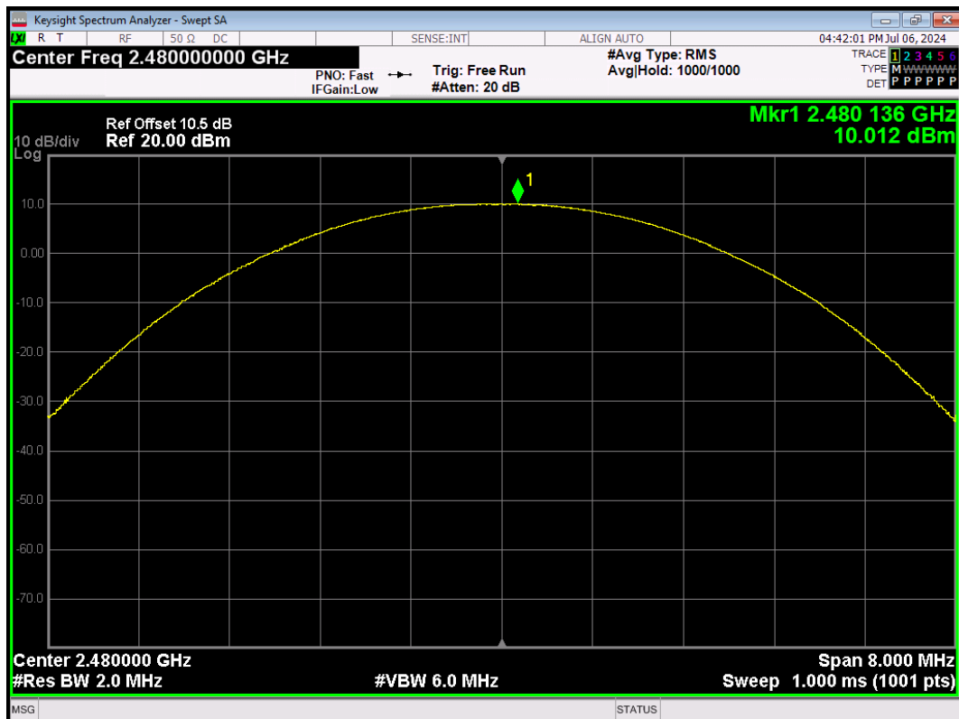
2DH5-Ant1-2480-PASS
