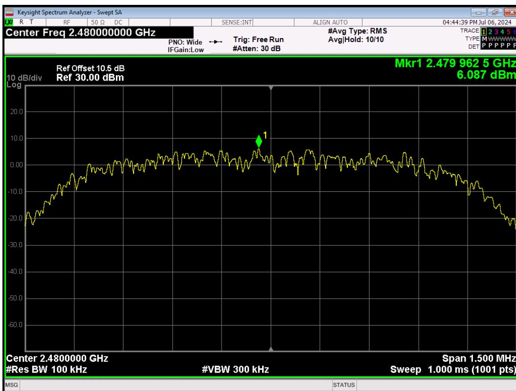
3DH5-Ant1-2480-0~Reference-PASS
