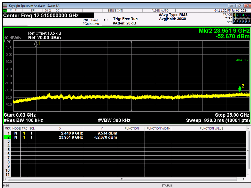
DH5-Ant1-2441-30~25000-PASS
