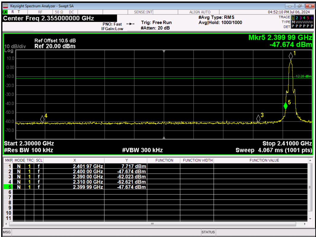
3DH5-Ant1-2402-PASS
