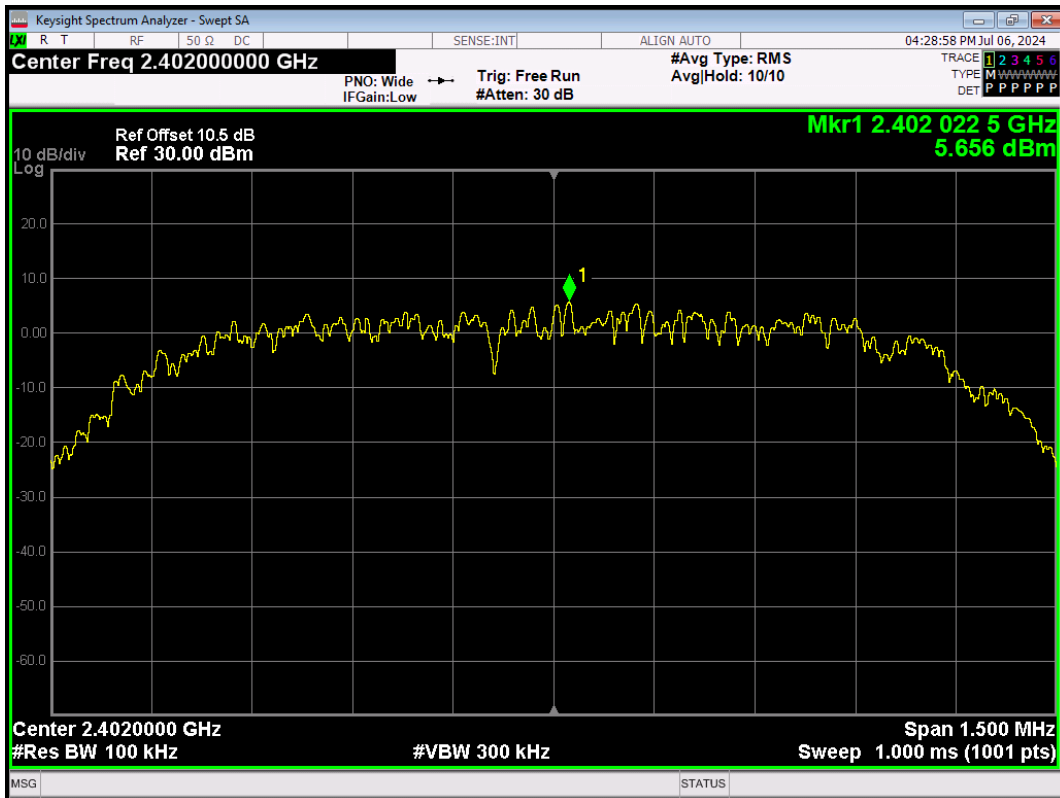
2DH5-Ant1-2402-0~Reference-PASS
