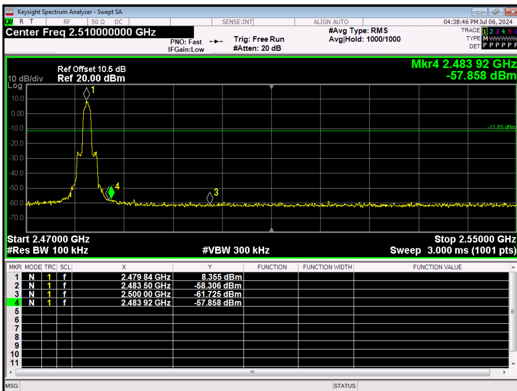
2DH5-Ant1-2480-PASS
