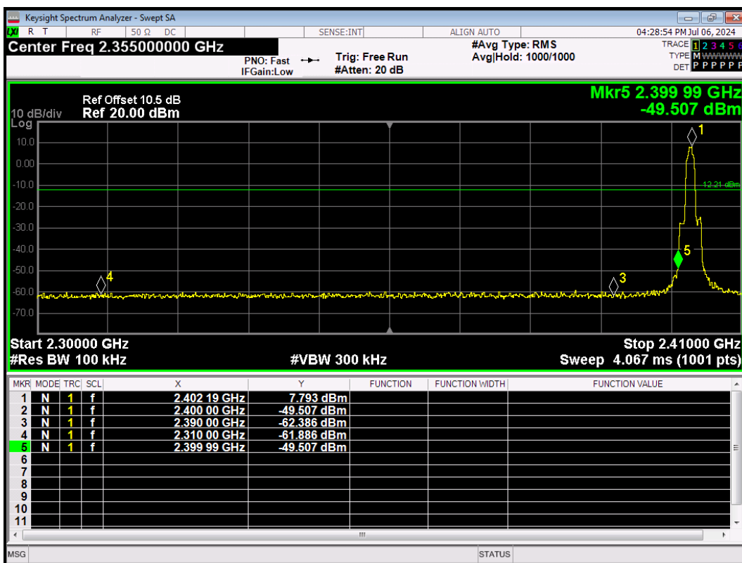
2DH5-Ant1-2402-PASS
