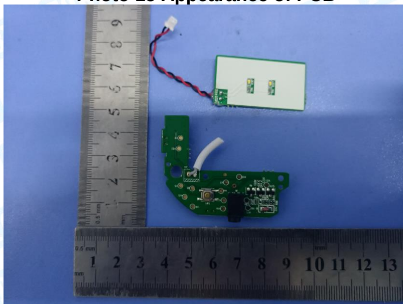
Photo 15 Appearance of PCB
