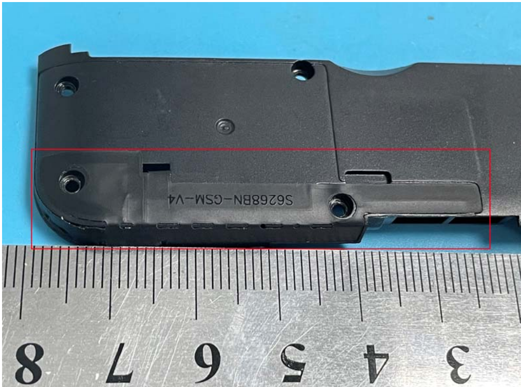
Main antenna
