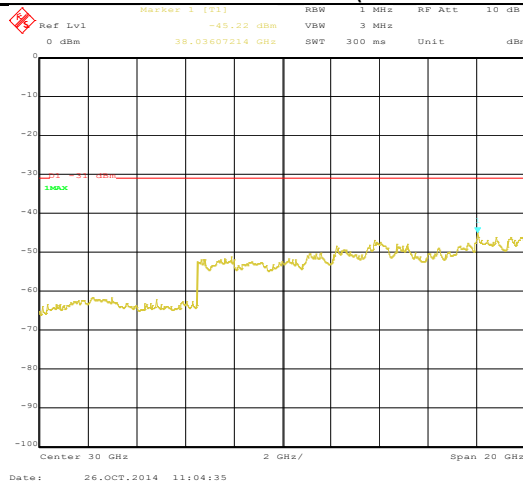
Chain 4 CSE - Mid CH 4965MHz (20GHz-40GHz)
