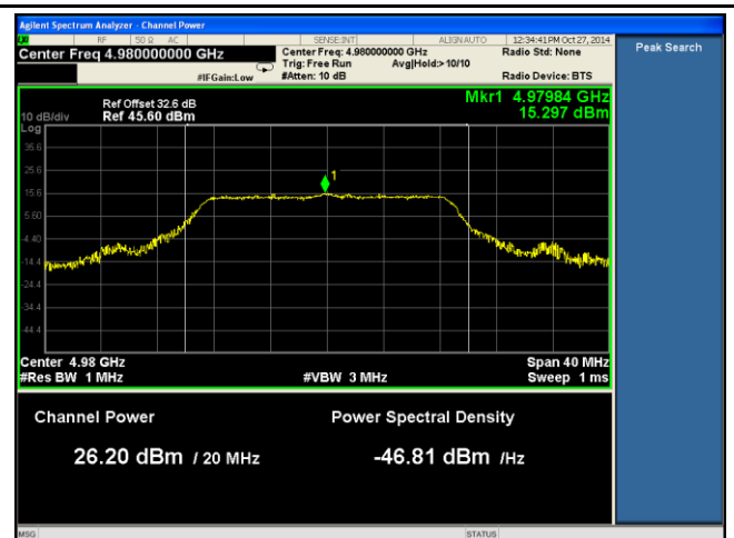
Chain 2 PSD (0dBi Antenna) - 4980MHz
