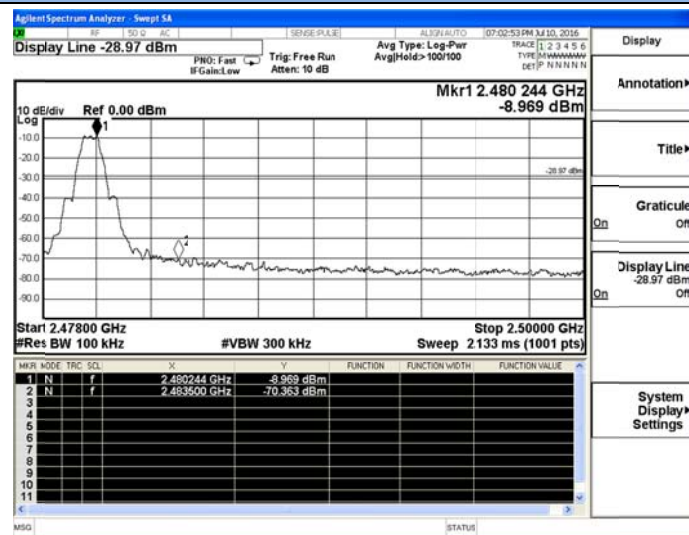
BT LE-High Channel, 2480MHz
