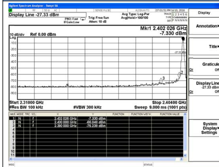
BT LE-Low Channel, 2402MHz
