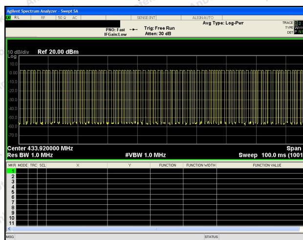
T period
