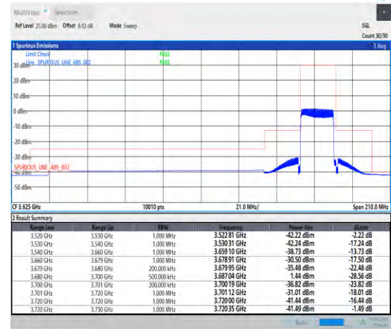
1-N48-PC3-30-20-H-3-DFT-PI2BPSK-Outer_Full-50@0-Ant3-1--PASS-see graph
