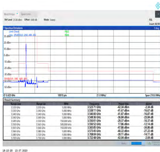
1-N48-PC3-30-15-L-1-DFT-PI2BPSK-Edge_1RB_Left-1@0-Ant3-1--PASS-see graph
