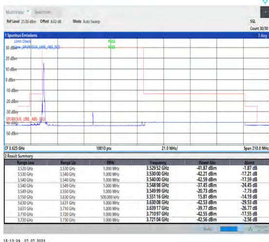
1-N48-PC3-30-80-L-4-CP-QPSK-Edge_1RB_Left-1@0-Ant3-1--PASS-see graph
