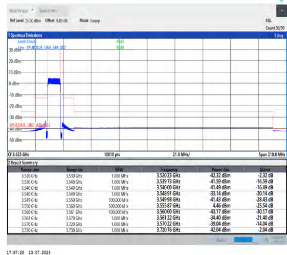
1-N48-PC3-30-10-L-6-CP-QPSK-Outer_Full-24@0-Ant3-1--PASS-see graph
