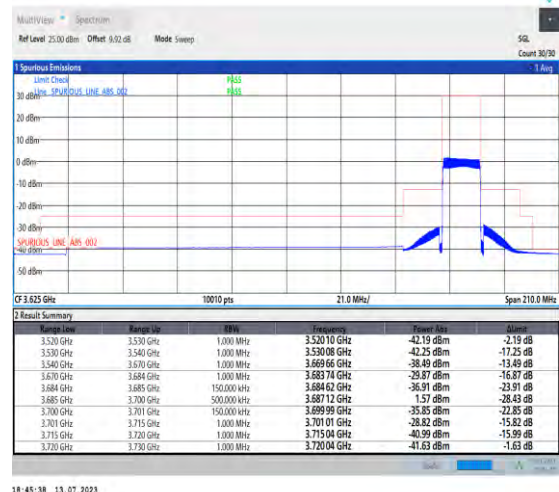
1-N48-PC3-30-15-H-6-CP-QPSK-Outer_Full-38@0Ant3-1--PASS-see graph
