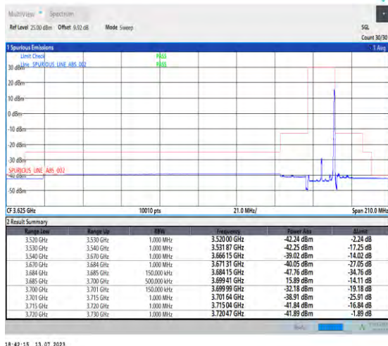
1-N48-PC3-30-15-H-5-CP-QPSK-Edge_1RB_Right-1@37-Ant3-1--PASS-see graph
