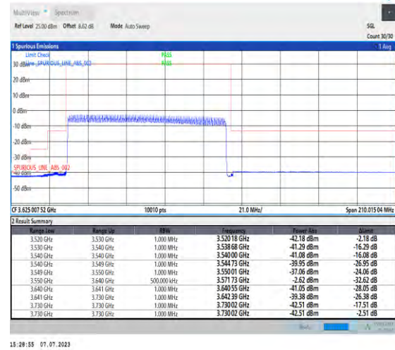
1-N48-PC3-30-90-L-3-DFT-PI2BPSK-Outer_Full-240@0-Ant3-1--PASS-see graph
