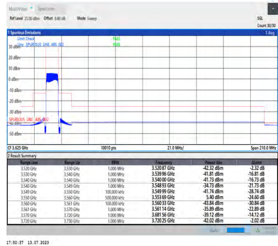
1-N48-PC3-30-10-L-3-DFT-PI2BPSK-Outer_Full-24@0-Ant3-1--PASS-see graph
