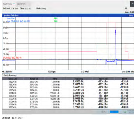
1-N48-PC3-30-15-H-2-DFT-PI2BPSK-Edge_1RB_Right-1@37-Ant3-1--PASS-see graph
