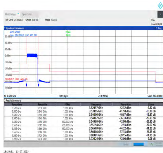
1-N48-PC3-30-15-L-3-DFT-PI2BPSK-Outer_Full-36@0Ant3-1--PASS-see graph
