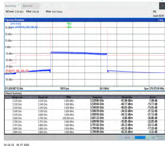
1-N48-PC3-30-100-H-6-CP-QPSK-Outer_Full-273 @0-Ant3-1--PASS-see graph
