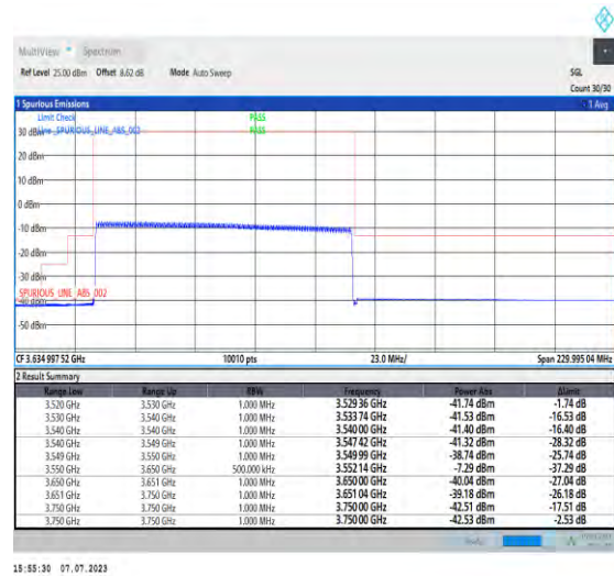
1-N48-PC3-30-100-L-6-CP-QPSK-Outer_Full-273 @0-Ant3-1--PASS-see graph
