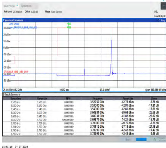
1-N48-PC3-30-90-H-5-CP-QPSK-Edge_1RB_Right-1@244-Ant3-1--PASS-see graph
