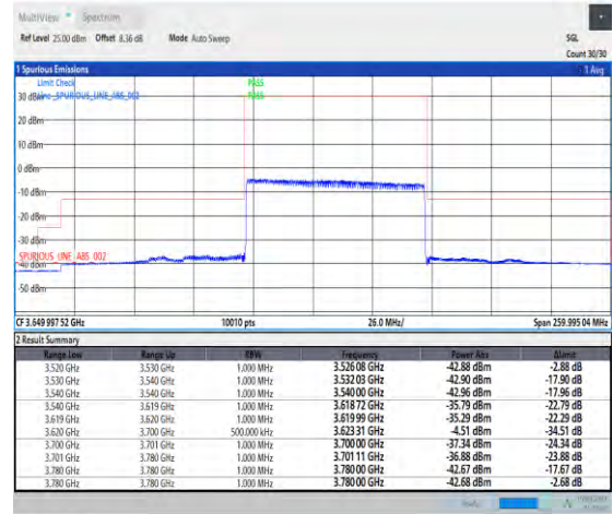
1-N48-PC3-30-80-H-3-DFT-PI2BPSK-Outer_Full-100@0-Ant3-1--PASS-see graph
