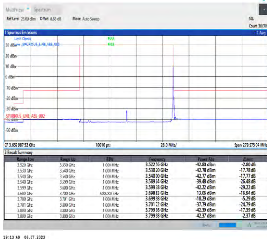
1-N48-PC3-30-100-H-5-CP-QPSK-Edge_1RB_Right-1 @272-Ant3-1--PASS-see graph
