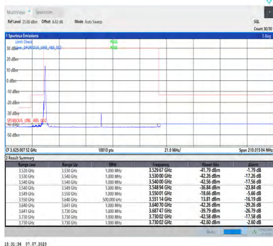
1-N48-PC3-30-90-L-4-CP-QPSK-Edge_1RB_Left-1@0-Ant3-1--PASS-see graph
