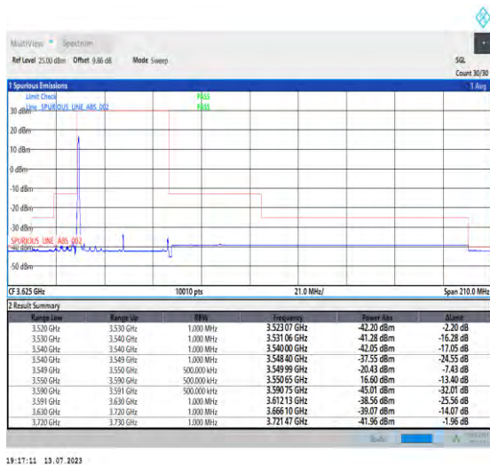
1-N48-PC3-30-40-L-1-DFT-PI2BPSK-Edge_1RB_Left -1@0-Ant3-1--PASS-see graph
