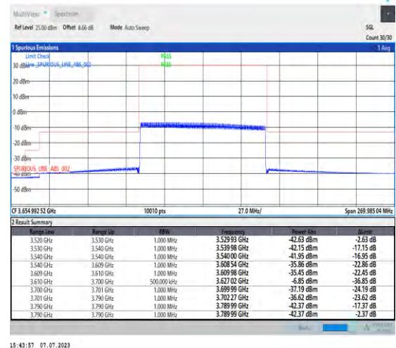
1-N48-PC3-30-90-H-6-CP-QPSK-Outer_Full-245@0-Ant3-1--PASS-see graph
