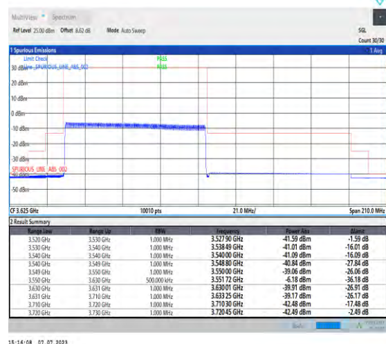
1-N48-PC3-30-80-L-6-CP-QPSK-Outer_Full-217@0-Ant3-1--PASS-see graph
