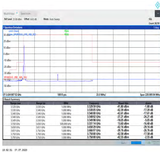
1-N48-PC3-30-100-L-4-CP-QPSK-Edge_1RB_Left-1 @0-Ant3-1--PASS-see graph
