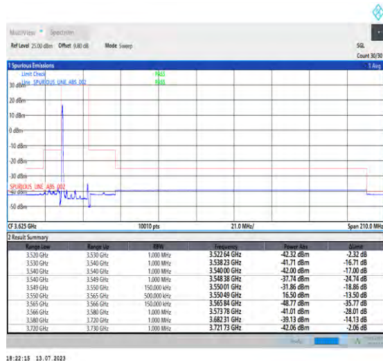
1-N48-PC3-30-15-L-4-CP-QPSK-Edge_1RB_Left-1@0-Ant3-1--PASS-see graph
