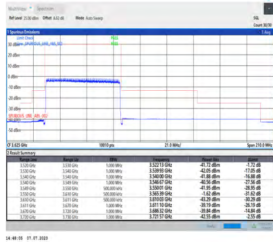
1-N48-PC3-30-60-L-3-DFT-PI2BPSK-Outer_Full-16 2@0-Ant3-1--PASS-see graph
