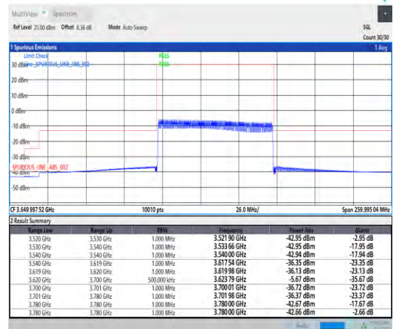
1-N48-PC3-30-80-H-6-CP-QPSK-Outer_Full-217@0-Ant3-1--PASS-see graph
