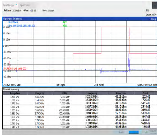
1-N48-PC3-30-40-H-2-DFT-PI2BPSK-Edge_1RB_Right-t-1@105-Ant3-1--PASS-see graph
