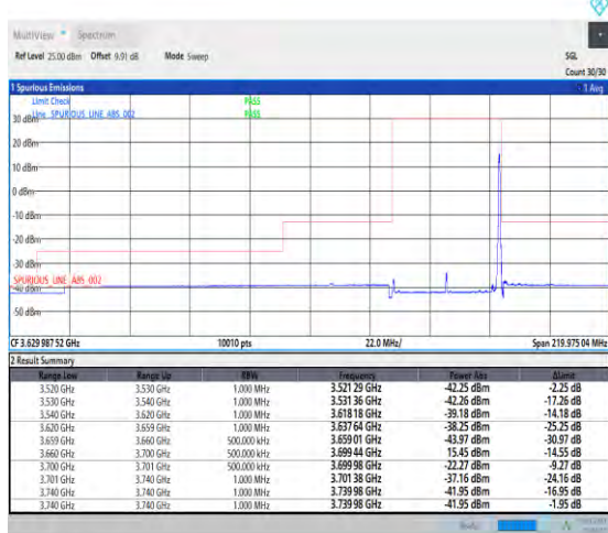
1-N48-PC3-30-40-H-5-CP-QPSK-Edge_1RB_Right-1@105-Ant3-1--PASS-see graph
