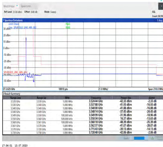
1-N48-PC3-30-10-L-4-CP-QPSK-Edge_1RB_Left-1@0-Ant3-1--PASS-see graph
