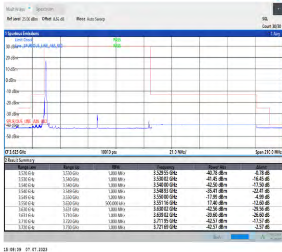
1-N48-PC3-30-80-L-1-DFT-PI2BPSK-Edge_1RB_Left-1@0-Ant3-1--PASS-see graph
