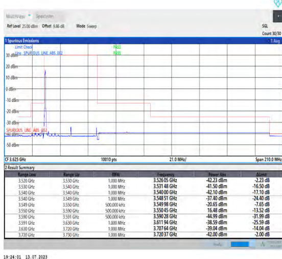
1-N48-PC3-30-40-L-4-CP-QPSK-Edge_1RB_Left-1@ 0-Ant3-1--PASS-see graph
