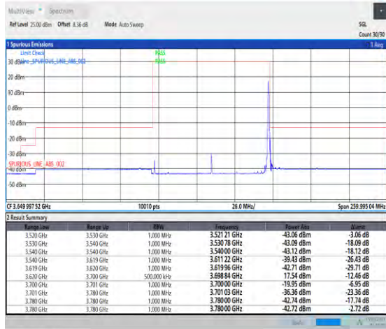
1-N48-PC3-30-80-H-2-DFT-PI2BPSK-Edge_1RB_Right-t-1@216-Ant3-1--PASS-see graph
