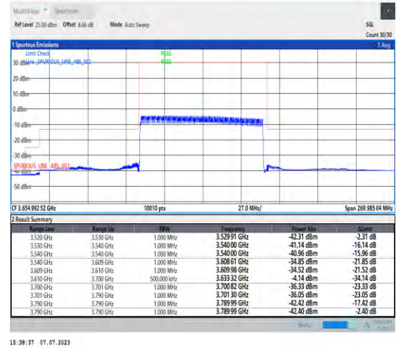
1-N48-PC3-30-90-H-3-DFT-PI2BPSK-Outer_Full-240@0-Ant3-1--PASS-see graph
