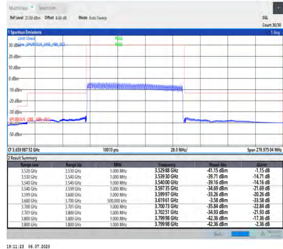
1-N48-PC3-30-100-H-3-DFT-PI2BPSK-Outer_Full -51@0-Ant3-1--PASS-see graph
