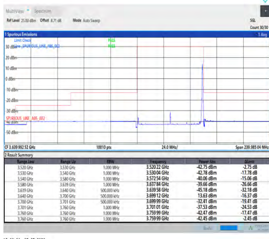
1-N48-PC3-30-60-H-5-CP-QPSK-Edge_1RB_Right-1@161-Ant3-1--PASS-see graph
