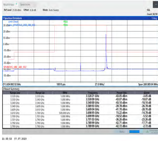
1-N48-PC3-30-90-H-2-DFT-PI2BPSK-Edge_1RB_Right-t-1@244-Ant3-1--PASS-see graph
