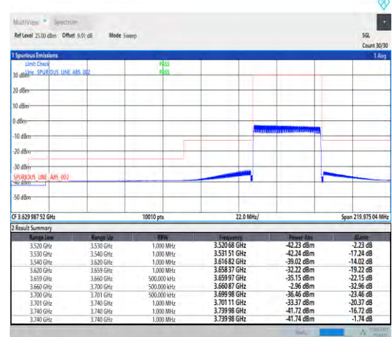
1-N48-PC3-30-40-H-6-CP-QPSK-Outer_Full-106@0-Ant3-1--PASS-see graph
