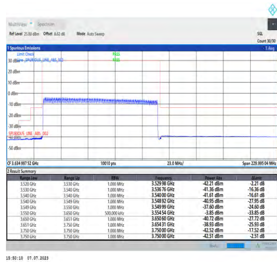
1-N48-PC3-30-100-L-3-DFT-PI2BPSK-Outer_Full-5 1@0-Ant3-1--PASS-see graph
