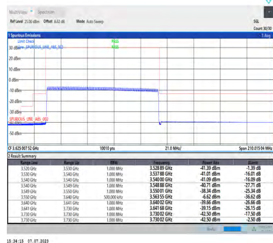
1-N48-PC3-30-90-L-6-CP-QPSK-Outer_Full-245@0-Ant3-1--PASS-see graph
