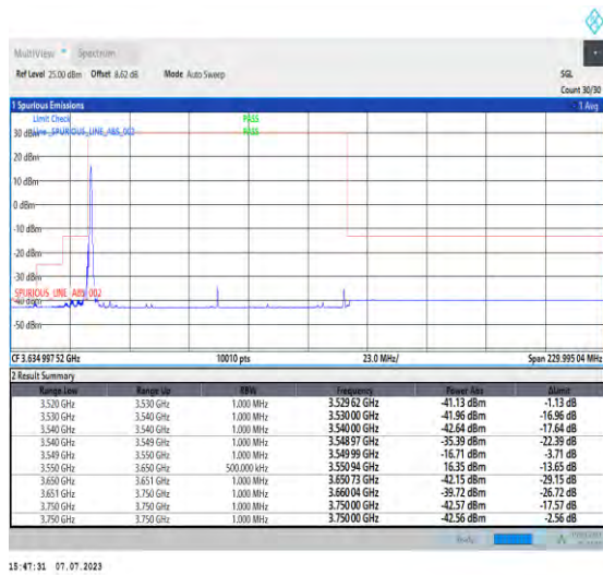
1-N48-PC3-30-100-L-1-DFT-PI2BPSK-Edge_1RB_Lef t-1@0-Ant3-1--PASS-see graph
