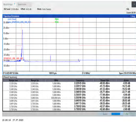
1-N48-PC3-30-90-L-1-DFT-PI2BPSK-Edge_1RB_Left-1@0-Ant3-1--PASS-see graph
