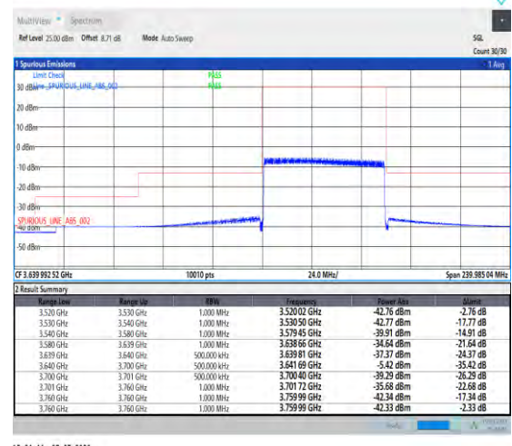
1-N48-PC3-30-60-H-6-CP-QPSK-Outer_Full-162@0-Ant3-1--PASS-see graph
