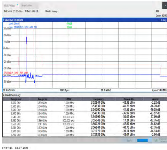
1-N48-PC3-30-10-L-1-DFT-PI2BPSK-Edge_1RB_Left-1@0-Ant3-1--PASS-see graph
