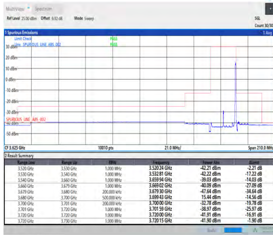
1-N48-PC3-30-20-H-2-DFT-PI2BPSK-Edge_1RB_Right-t-1@50-Ant3-1--PASS-see graph
