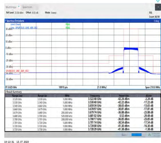
1-N48-PC3-30-20-H-6-CP-QPSK-Outer_Full-51@0-Ant3-1--PASS-see graph
