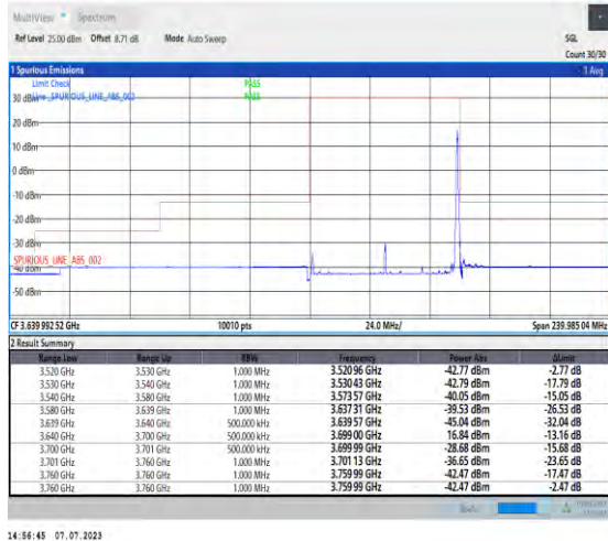
1-N48-PC3-30-60-H-2-DFT-PI2BPSK-Edge_1RB_Right-t-1@161-Ant3-1--PASS-see graph
