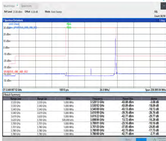
1-N48-PC3-30-80-H-5-CP-QPSK-Edge_1RB_Right-1@216-Ant3-1--PASS-see graph
