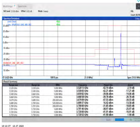
1-N48-PC3-30-20-H-5-CP-QPSK-Edge_1RB_Right-1@50-Ant3-1--PASS-see graph
