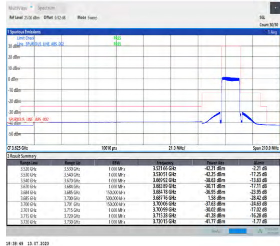
1-N48-PC3-30-15-H-3-DFT-PI2BPSK-Outer_Full-36@0Ant3-1--PASS-see graph
