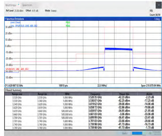
1-N48-PC3-30-40-H-3-DFT-PI2BPSK-Outer_Full-100@0-Ant3-1--PASS-see graph
