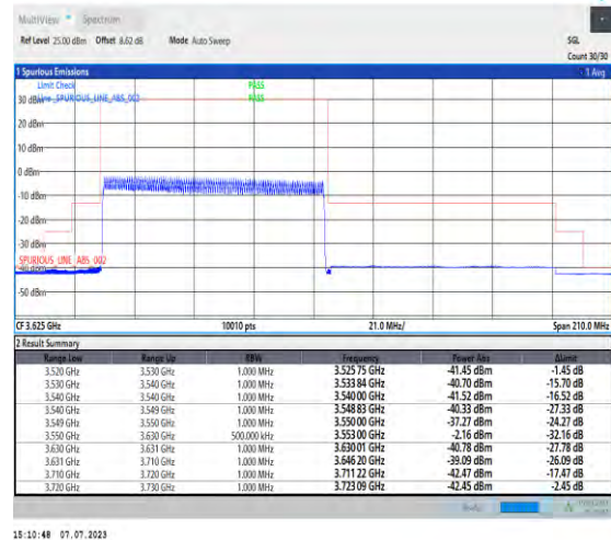
1-N48-PC3-30-80-L-3-DFT-PI2BPSK-Outer_Full-10 0@0-Ant3-1--PASS-see graph
