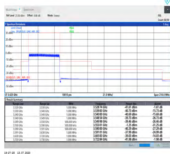
1-N48-PC3-30-40-L-6-CP-QPSK-Outer_Full-106@0 -Ant3-1--PASS-see graph
