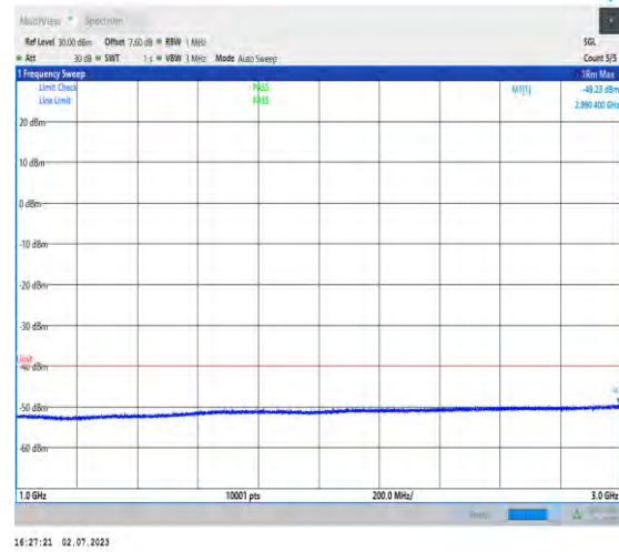
1-N48-PC3-30-100-M-1-NS_01-DFT-PI2BPSK-Inner_1RB_Left-1@1-1000-3000-Ant3-2990.40--49.23--40- PASS
