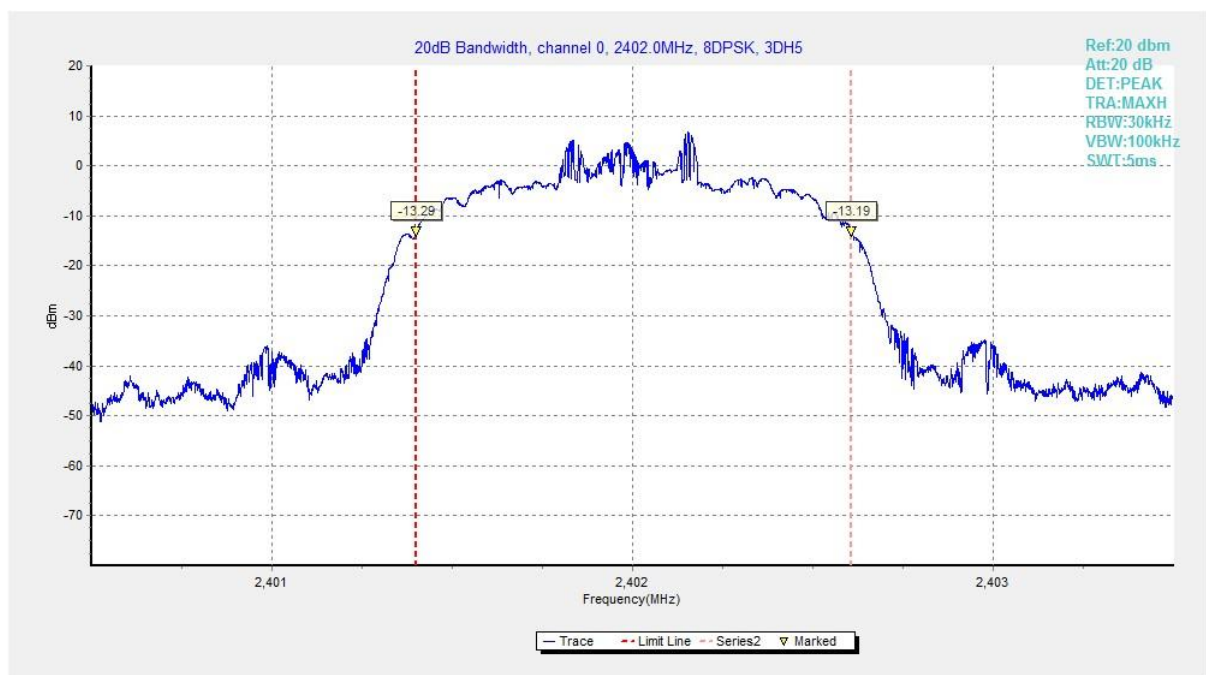
Fig. 67 20dB Bandwidth (8DPSK, Ch 0)
