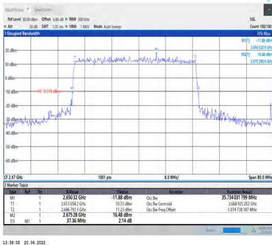
1-N41-PC2-30-40-H-3-DFT-16QAM-Outet_Full-100@ 0-Ant1-35.734-37.360-≤40-PASS
