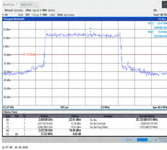
1-N41-PC2-30-40-H-1-DFT-QPSK-Outet_Full-100@ 0-Ant1-35.725-37.520-≤40-PASS
