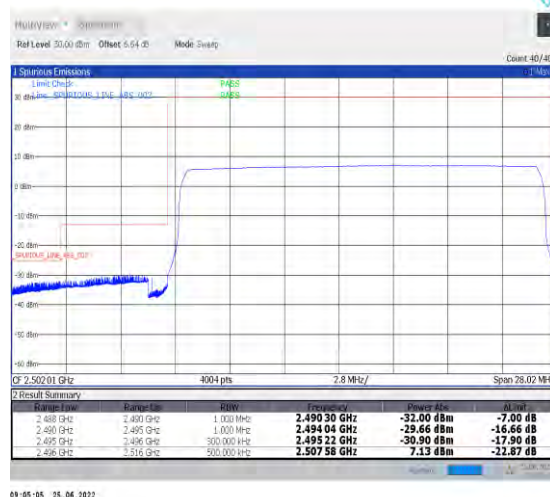
1-N41-PC2-30-20-L-6-CP-QPSK-Outer_Full-51@0-Ant1-PASS-see graph
