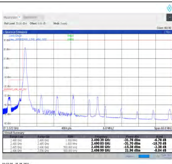
1-N41-PC2-30-60-L-1-DFT-PI2BPSK-Edge_1RB_Left-1@0-Ant1-PASS-see graph
