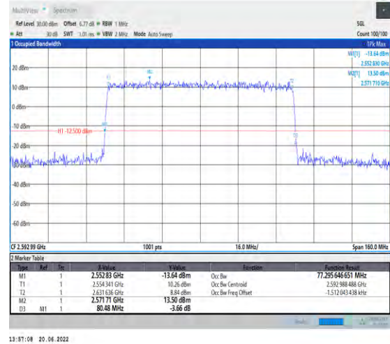
1-N41-PC2-30-80-M-6-CP-QPSK-Outer_Full-217@0 -Ant1-77.296-80.480-≤80-PASS
