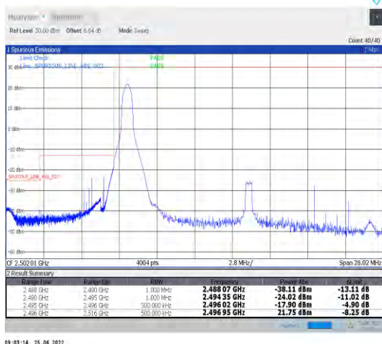
1-N41-PC2-30-20-L-4-CP-QPSK-Edge_1RB_Left-1@0-Ant1-PASS-see graph
