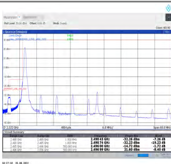
1-N41-PC2-30-60-L-4-CP-QPSK-Edge_1RB_Left-1@0-Ant1-PASS-see graph
