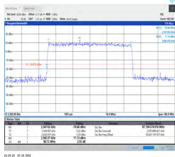
1-N41-PC2-30-90-M-9-CP-256QAM-Outer_Full-245@0-Ant1-87.195-90.720-≤90-PASS
