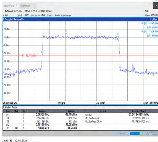
1-N41-PC2-30-60-M-4-DFT-64QAM-Outer_Full-162 @0-Ant1-57.542-59.880-≤60-PASS
