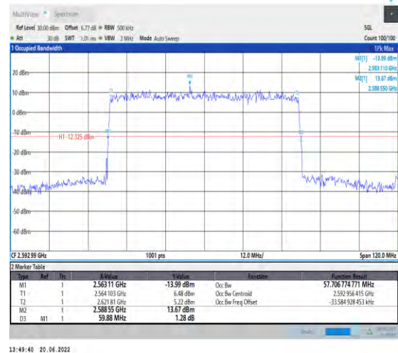
1-N41-PC2-30-60-M-5-DFT-256QAM-Outer_Full-162 @0-Ant1-57.707-59.880-≤60-PASS
