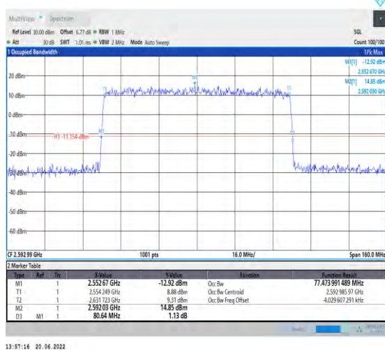
1-N41-PC2-30-80-M-7-CP-16QAM-Outer_Full-217@ 0-Ant1-77.474-80.640-≤80-PASS
