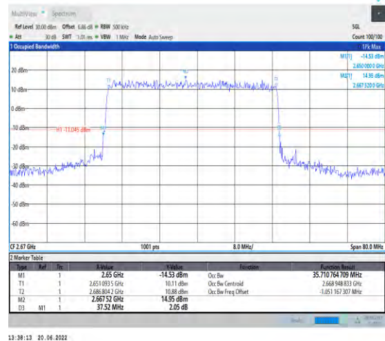
1-N41-PC2-30-40-H-4-DFT-64QAM-Outet_Full-100@ 0-Ant1-35.711-37.520-≤40-PASS
