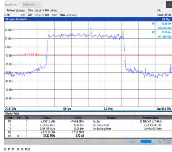
1-N41-PC2-30-40-H-2-DFT-PI2BPSK-Outet_Full-100@ 0-Ant1-35.697-37.520-≤40-PASS
