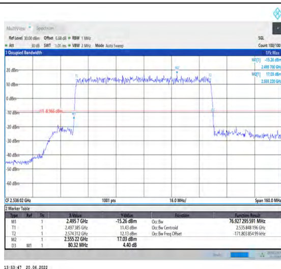
1-N41-PC2-30-80-L-2-DFT-PI2BPSK-Outer_Full-216 @0-Ant1-76.927-80.320-≤80-PASS
