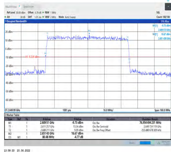
1-N41-PC2-30-80-H-3-DFT-16QAM-Outer_Full-216 @0-Ant1-76.954-80.480-≤80-PASS
