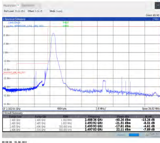
1-N41-PC2-30-20-L-1-DFT-PI2BPSK-Edge_1RB_Left-1@0-Ant1-PASS-see graph
