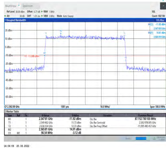
1-N41-PC2-30-90-M-7-CP-16QAM-Outer_Full-245@0-Ant1-87.153-90.540-≤90-PASS
