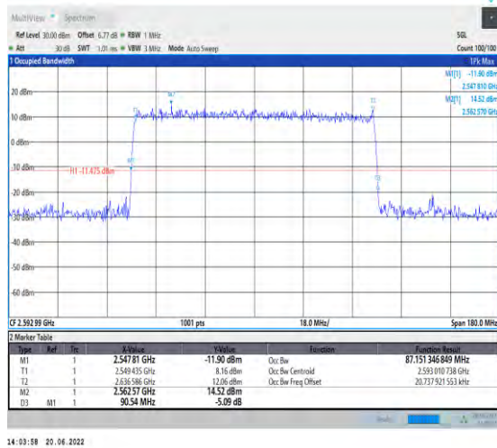
1-N41-PC2-30-90-M-6-CP-QPSK-Outer_Full-245@0 -Ant1-87.151-90.540-≤90-PASS
