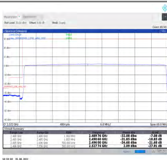
1-N41-PC2-30-60-L-6-CP-QPSK-Outer_Full-162@0-Ant1-PASS-see graph
