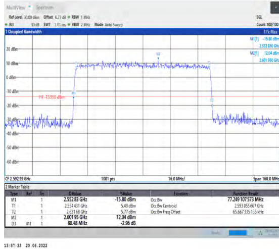
1-N41-PC2-30-80-M-9-CP-256QAM-Outer_Full-217 @0-Ant1-77.249-80.480-≤80-PASS
