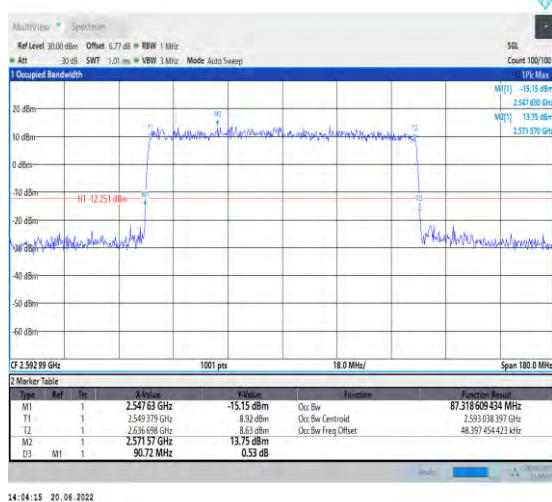
1-N41-PC2-30-90-M-8-CP-64QAM-Outer_Full-245@0-Ant1-87.319-90.720-≤90-PASS
