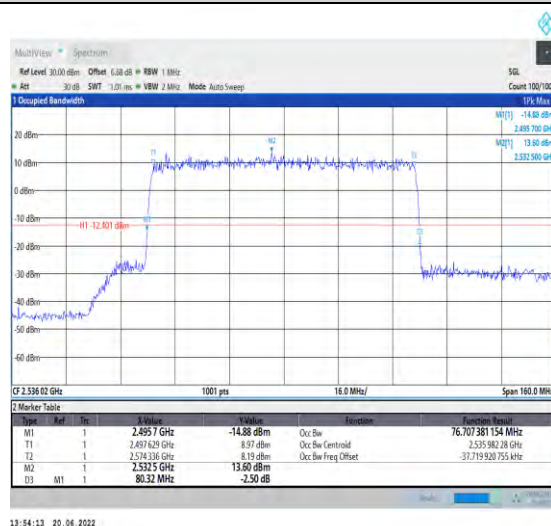
1-N41-PC2-30-80-L-5-DFT-256QAM-Outer_Full-216 @0-Ant1-76.707-80.320-≤80-PASS
