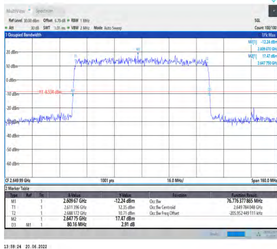
1-N41-PC2-30-80-H-2-DFT-PI2BPSK-Outer_Full-216 @0-Ant1-76.776-80.160-≤80-PASS
