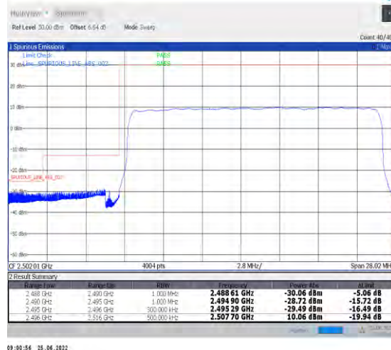
1-N41-PC2-30-20-L-3-DFT-PI2BPSK-Outer_Full-50@0-Ant1-PASS-see graph
