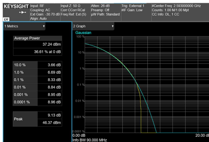
Channel: MIDDLE, Modulation: 64QAM, BW=90MHz, CCDF
