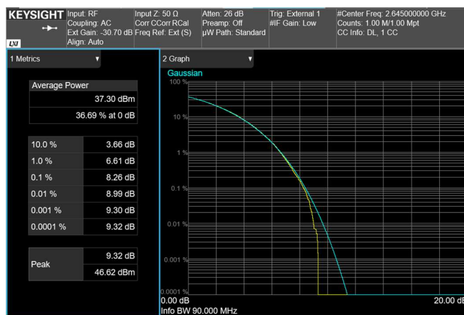
Channel: TOP, Modulation: 64QAM, BW=90MHz, CCDF
