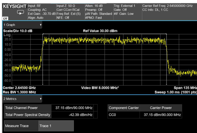
Channel: TOP, Modulation: 64QAM, BW=90MHz, Channel Power
