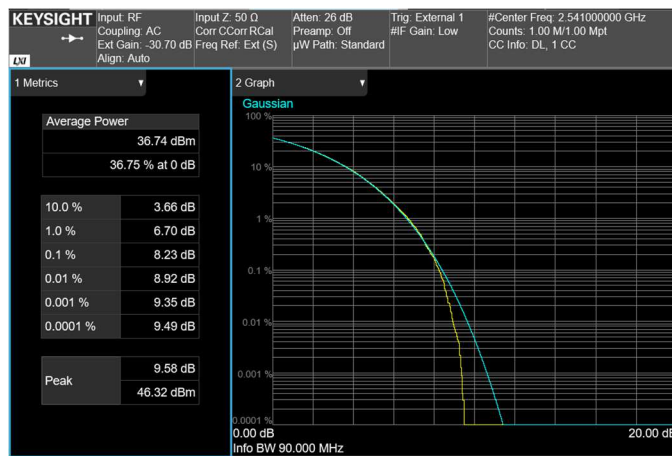
Channel: BOTTOM, Modulation: 64QAM, BW=90MHz, CCDF
