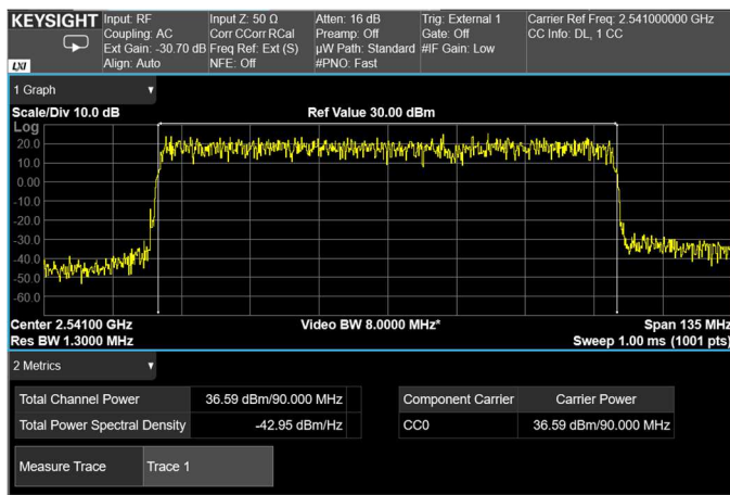
Channel: BOTTOM, Modulation: 64QAM, BW=90MHz, Channel Power
