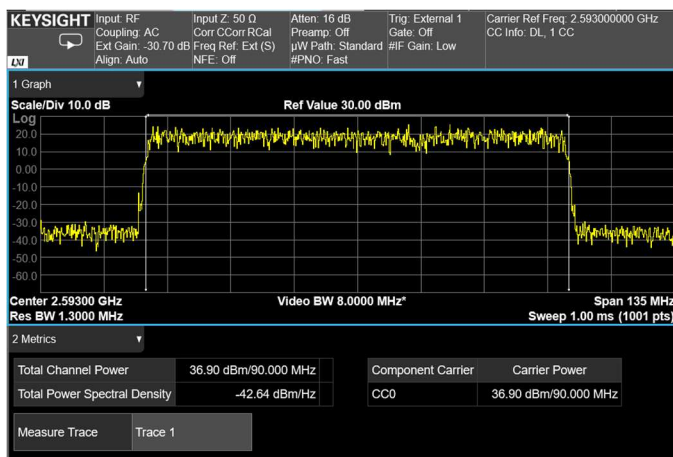
Channel: MIDDLE, Modulation: 64QAM, BW=90MHz, Channel Power
