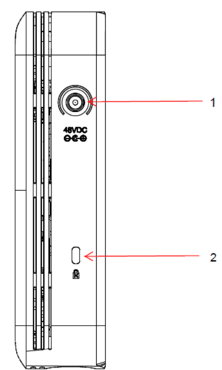
Figure 5 Access Point Ports and Connections on the Left of the AP
