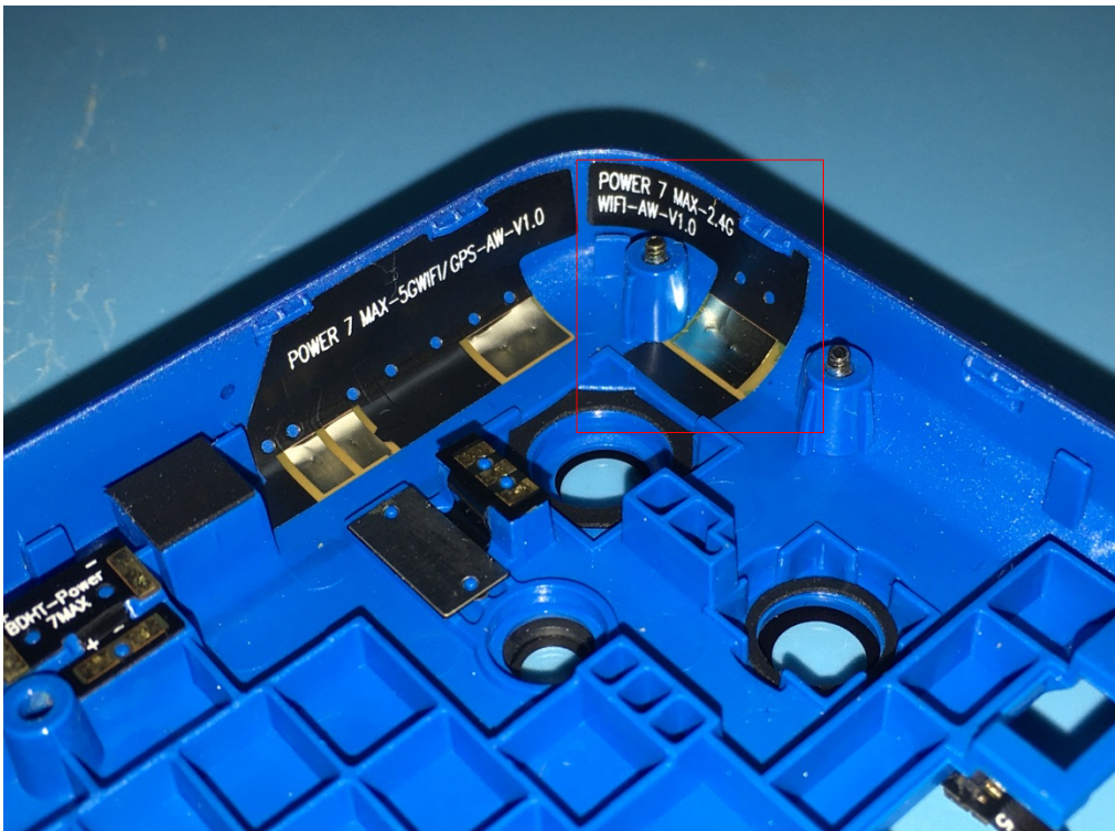
2.4G Wi-Fi/BT/BLE antenna
