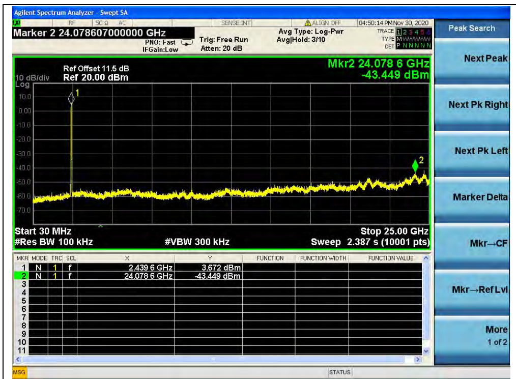
(30MHz to 25GHz, Channel 7, 802.11g)
