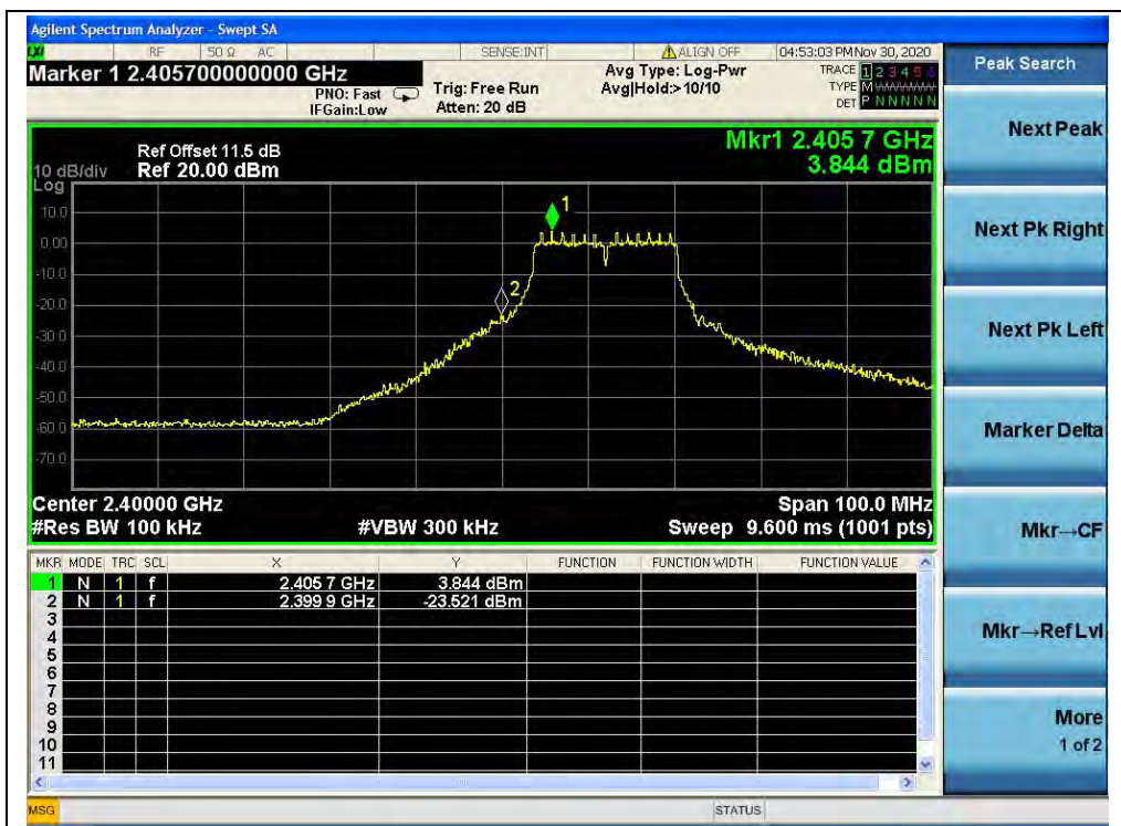
(Band Edge, Channel 1, 802.11g)
