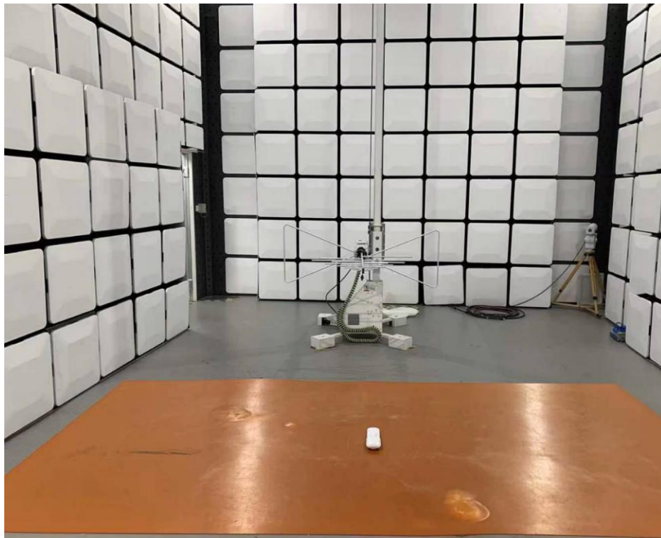
Radiated Measurement (Below 1GHz)
