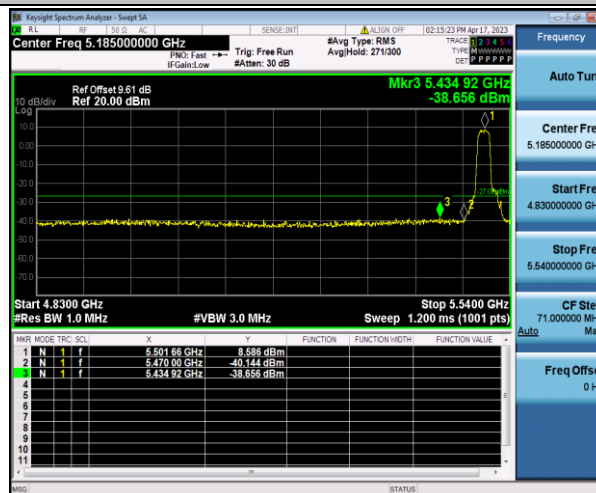
11N20SISO_Ant1_Low_5500
