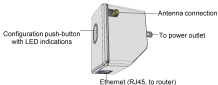
Figure 5: Wi-Fi Gateway interfaces
