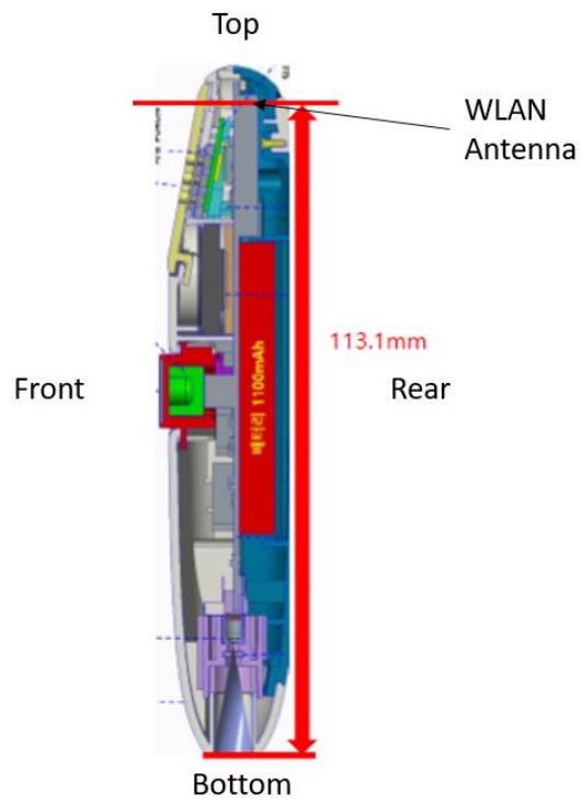
Figure E-1 Antenna Location_3
