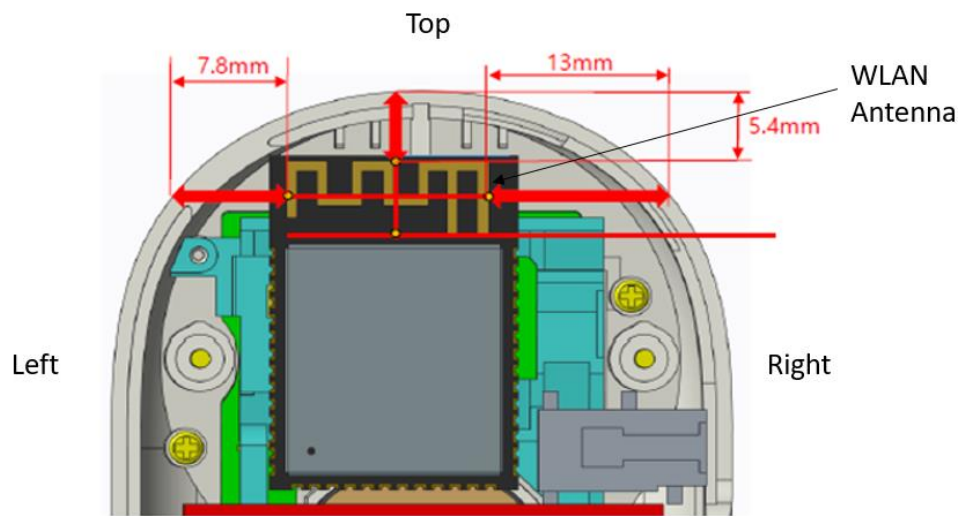
Figure E-1 Antenna Location_1
