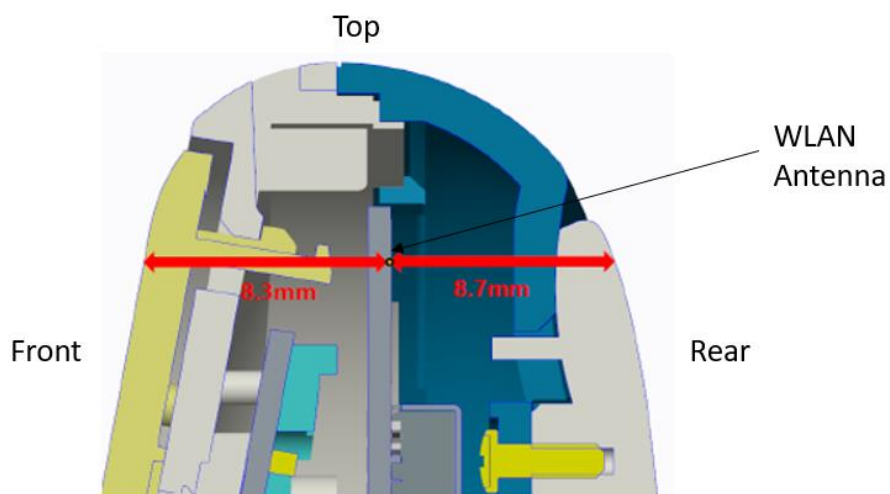
Figure E-1 Antenna Location_2
