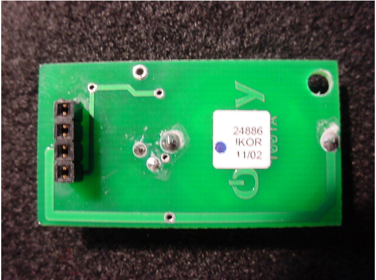
Figure 7: Oscillator Module – Bottom View
