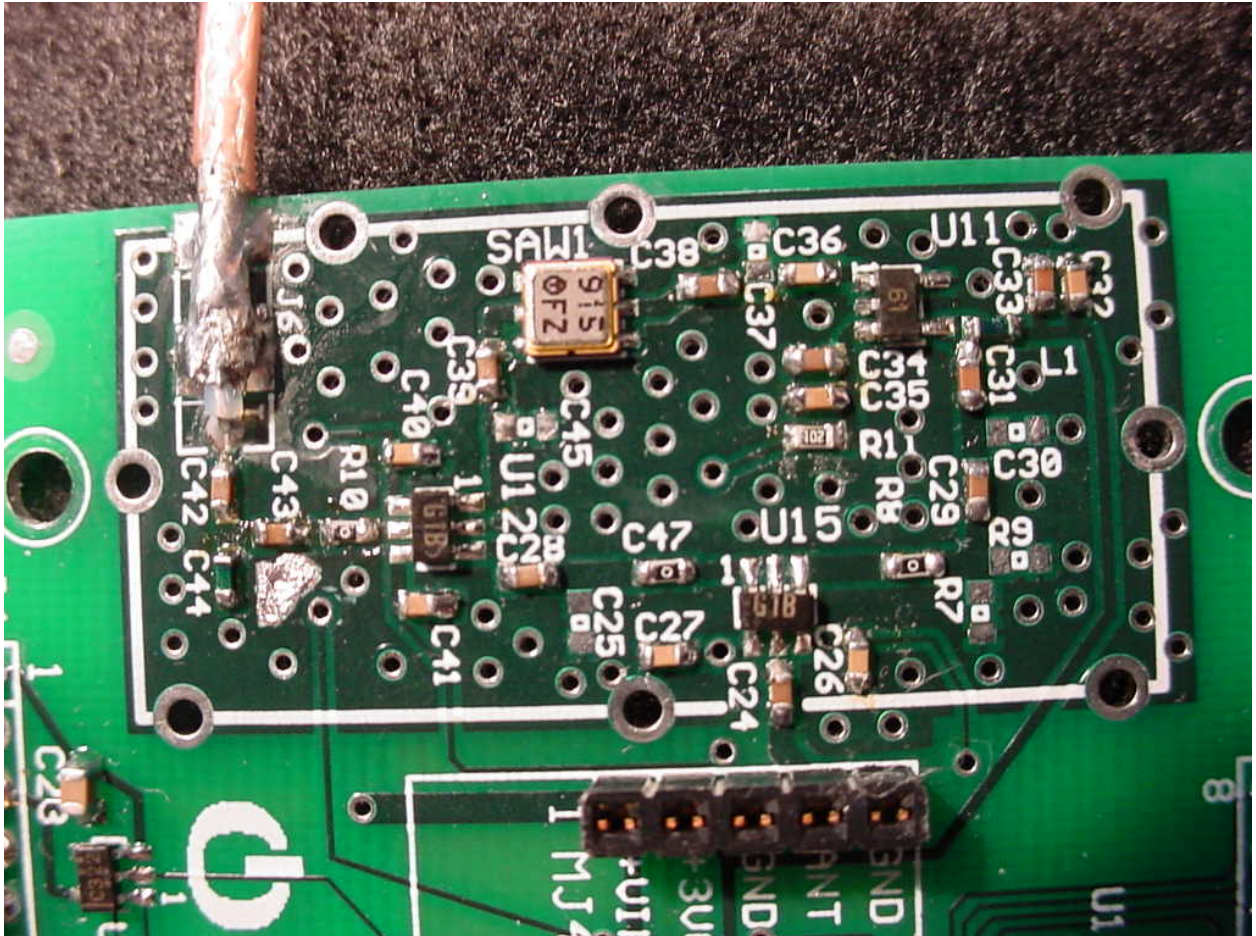
Figure 4: RF Output Circuitry – Top view
