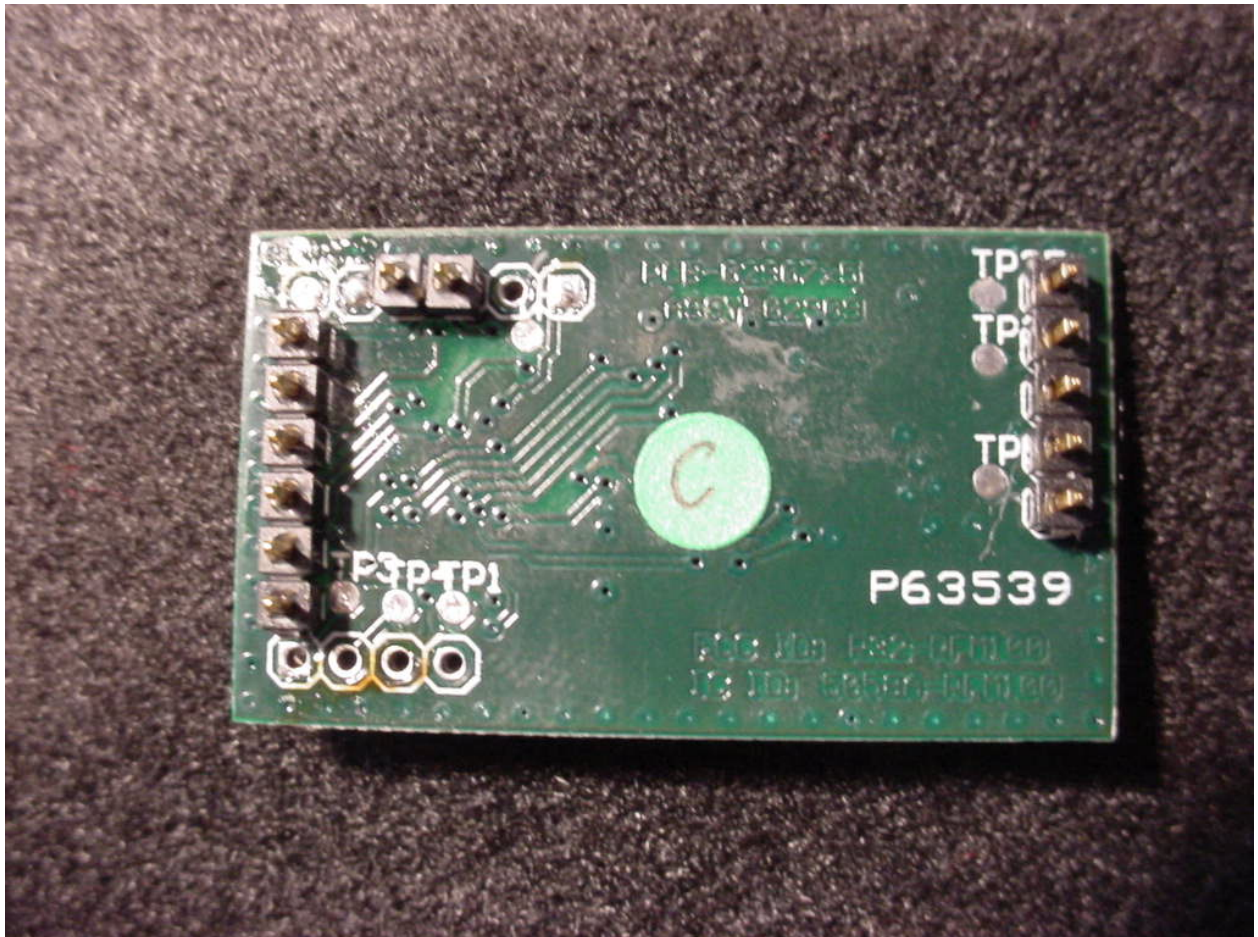
Figure 9: Transmitter Module – Bottom View
