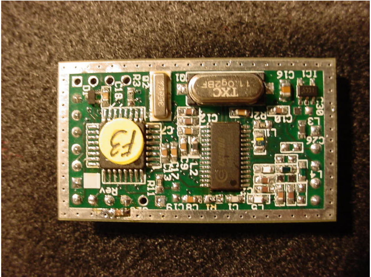
Figure 8: Transmitter Module – Top View
