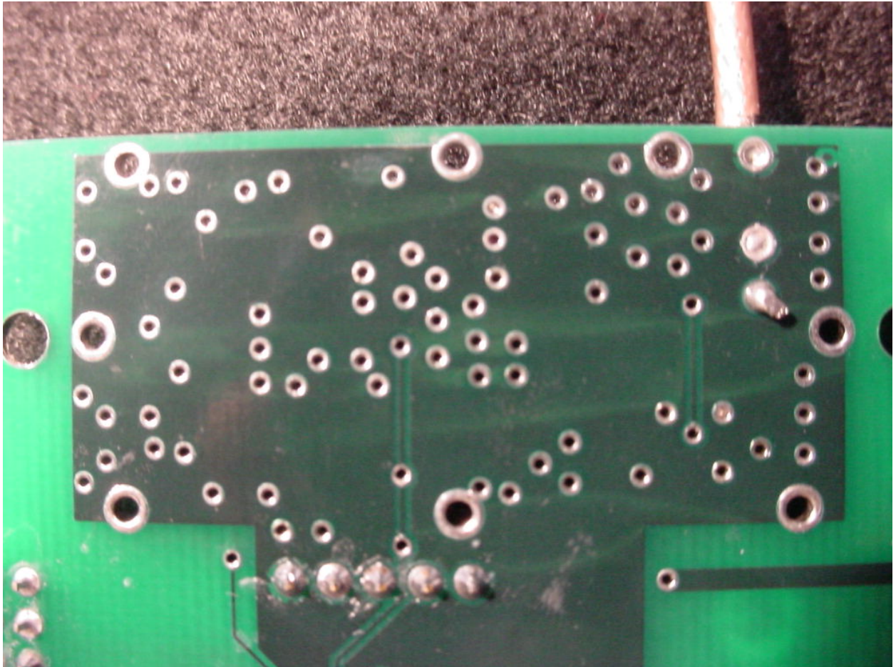
Figure 5: RF Output Circuitry – Bottom View
