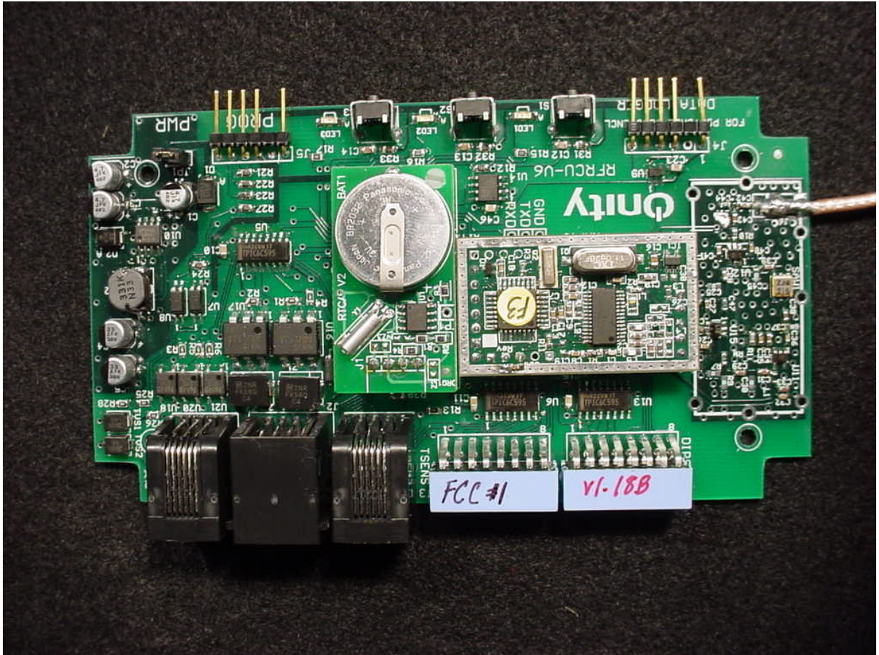
Figure 2: Main Board – Top View
