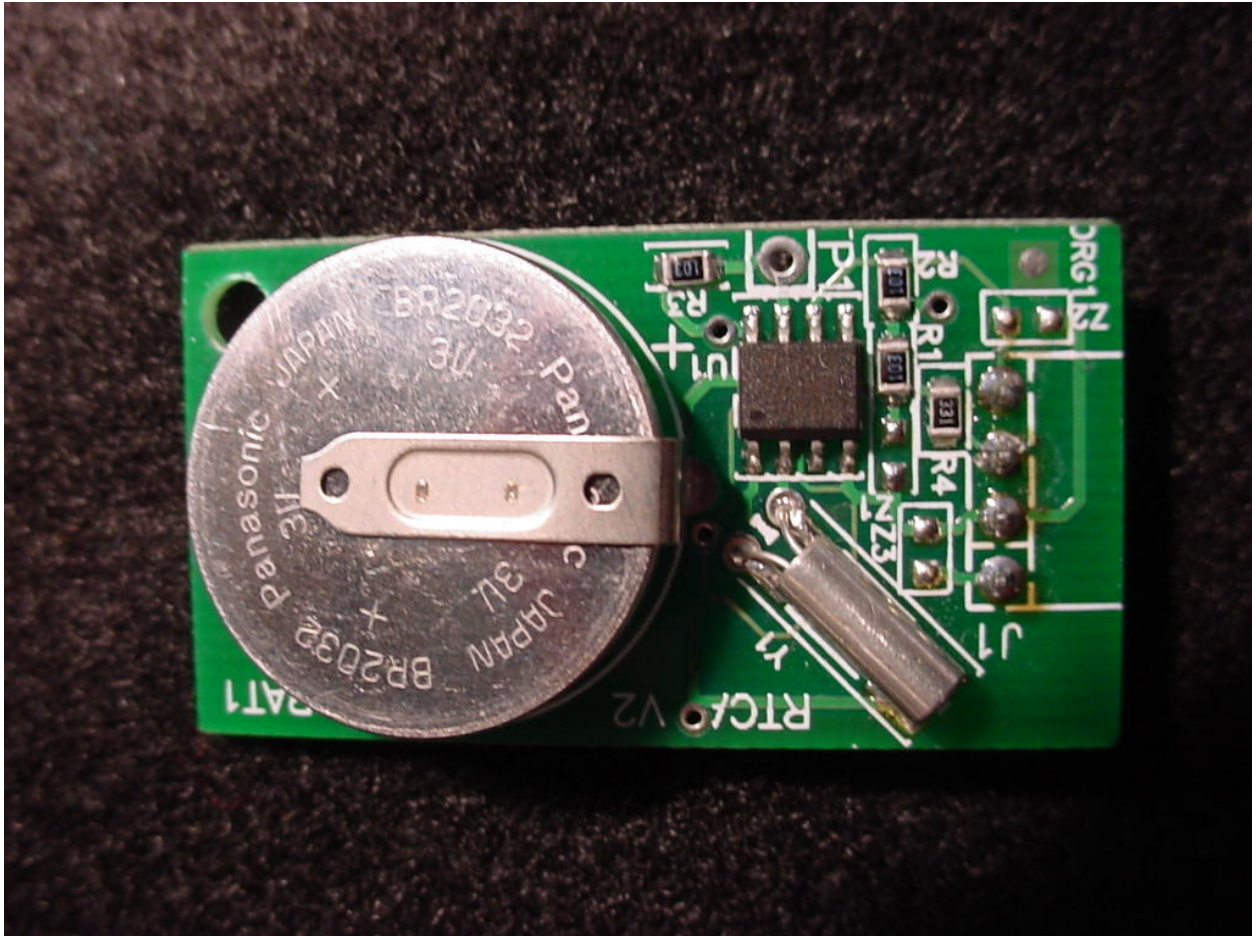
Figure 6: Oscillator Module – Top View
