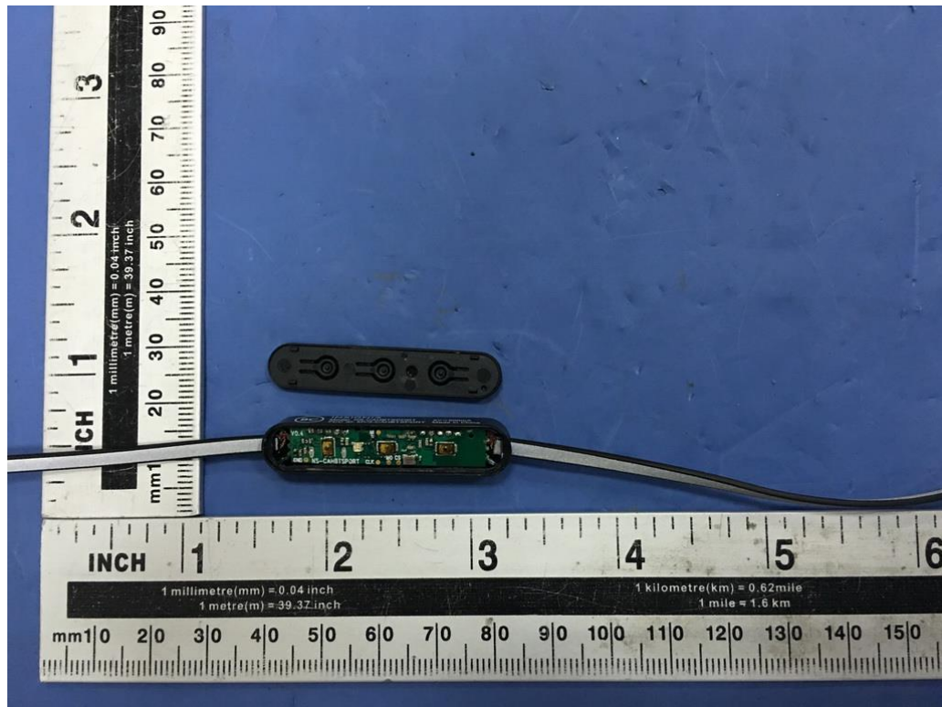
Fig. 1: Internal view
