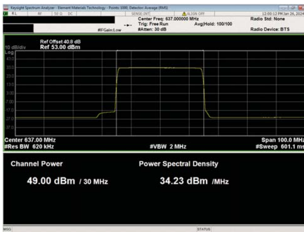
Port 1 NR 30 MHz Channel Bandwidth QPSK High Ch, 637.0 MHz
