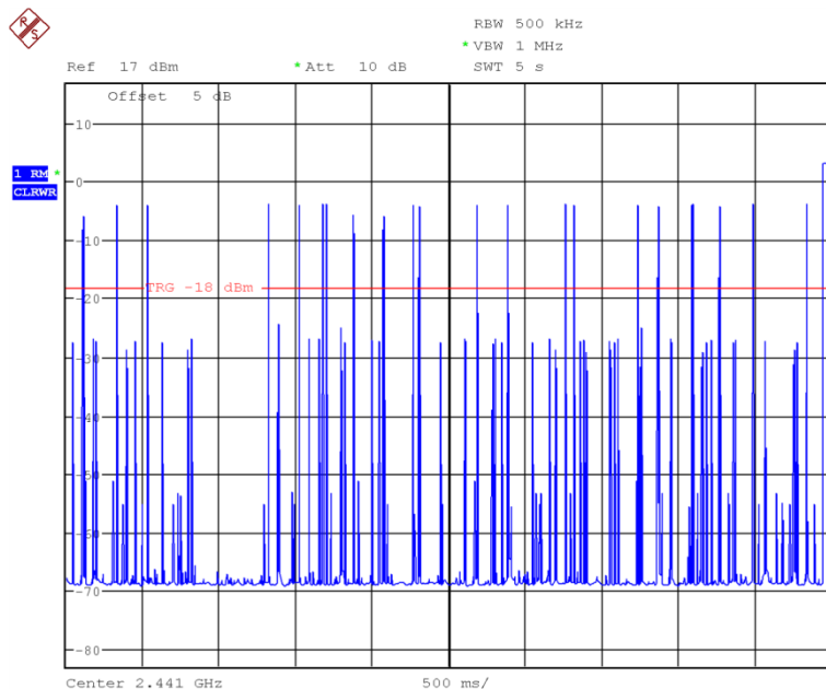
Fig.58 Number of Transmissions Measurement: Ch39, Packet DH3
