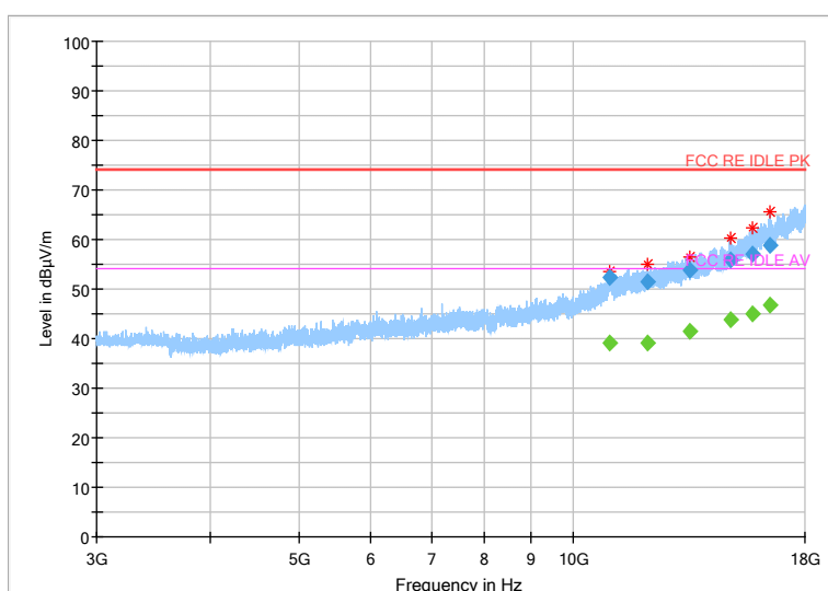
Fig 52 Radiated emission: 8DPSK, Ch0, 3GHz~18GHz
