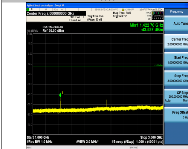
Band12_5MHz_16QAM_23155_1RB#0_1000~3000_1000~3000
