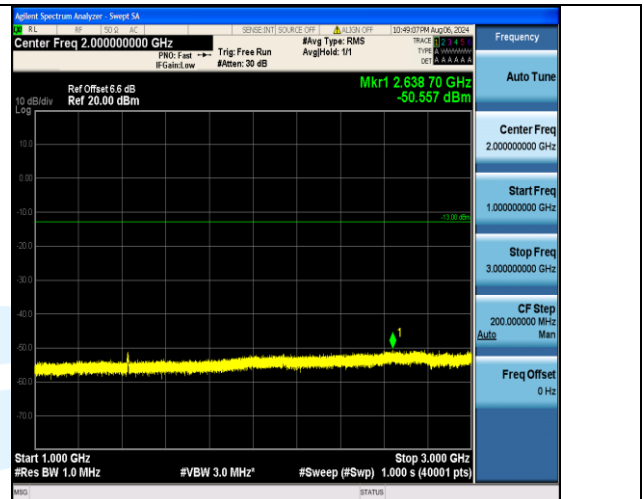
Band12_5MHz_QPSK_23155_25RB#0_1000~3000_1000~3000
