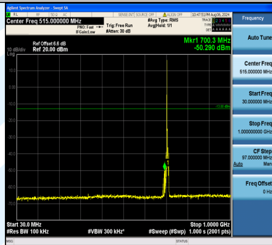
Band12_5MHz_16QAM_23155_1RB#0_30~1000_30~1000
