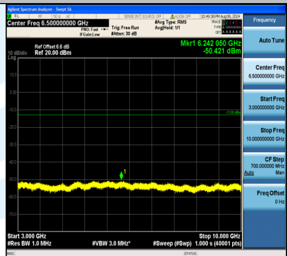
Band12_5MHz_16QAM_23155_25RB#0_3000~10000_3000~10000
