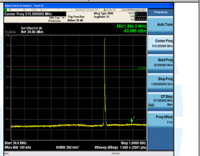
Band12_5MHz_16QAM_23035_1RB#0_30~1000_30~1000
