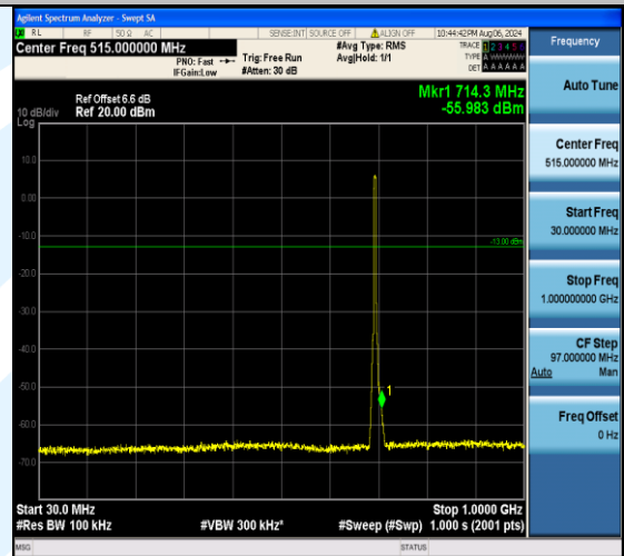
Band12_5MHz_16QAM_23035_25RB#0_30~1000_30~1000
