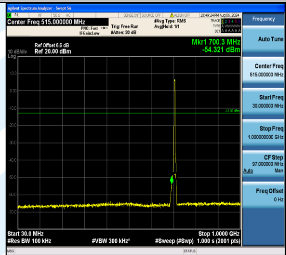
Band12_5MHz_16QAM_23155_25RB#0_30~1000_30~1000
