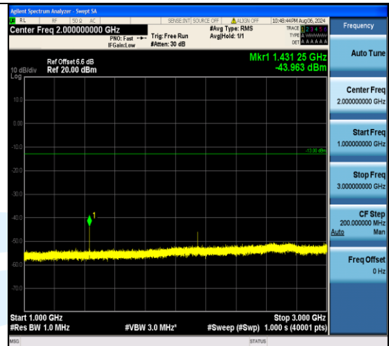
Band12_5MHz_16QAM_23155_1RB#24_1000~3000_1000~3000
