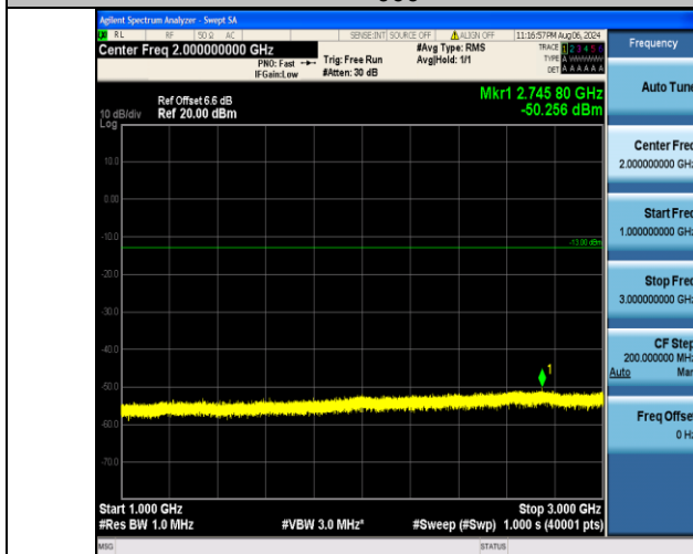
Band12_10MHz_QPSK_23060_1RB#49_1000~3000_1000~3000
