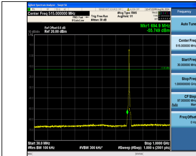
Band12_5MHz_16QAM_23095_25RB#0_30~1000_30~1000
