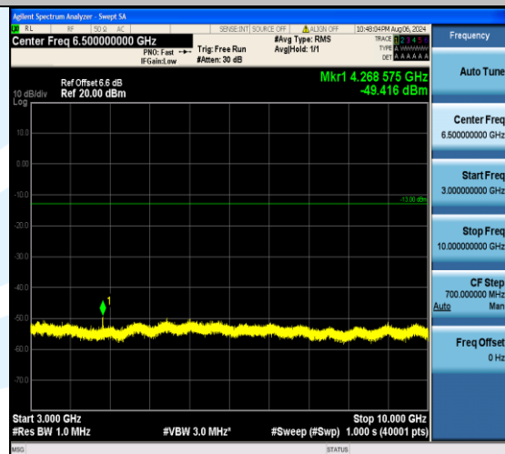
Band12_5MHz_16QAM_23155_1RB#0_3000~10000_3000~10000
