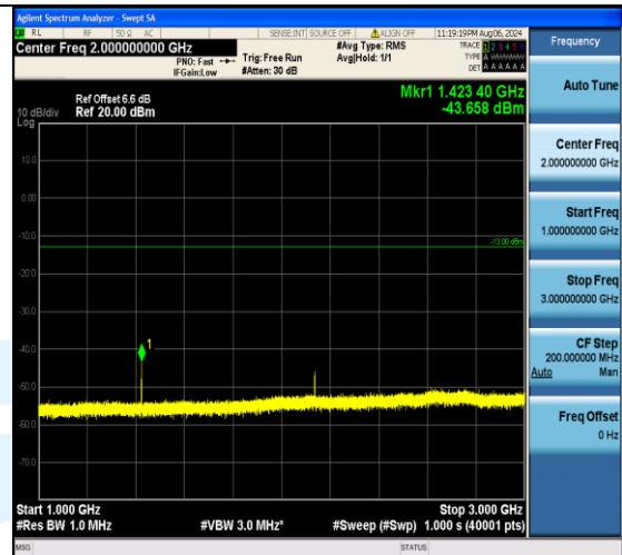
Band12_10MHz_QPSK_23095_1RB#49_1000~3000_1000~3000
