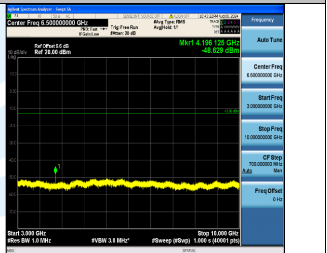
Band12_5MHz_16QAM_23035_1RB#0_3000~10000_3000~10000
