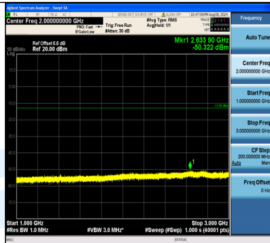
Band12_5MHz_16QAM_23095_25RB#0_1000~3000_1000~3000
