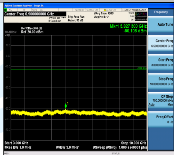
Band12_10MHz_QPSK_23095_50RB#0_3000~10000_3000~10000
