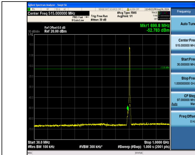
Band12_5MHz_QPSK_23155_25RB#0_30~1000_30~1000
