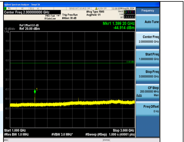
Band12_10MHz_QPSK_23060_1RB#0_1000~3000_1000~3000
