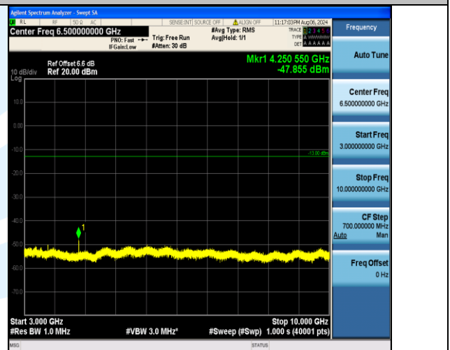
Band12_10MHz_QPSK_23060_1RB#49_3000~10000_3000~10000
