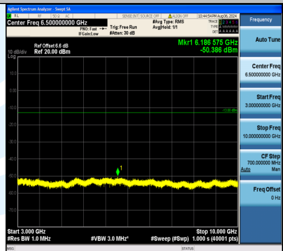
Band12_5MHz_16QAM_23035_25RB#0_3000~10000_3000~10000
