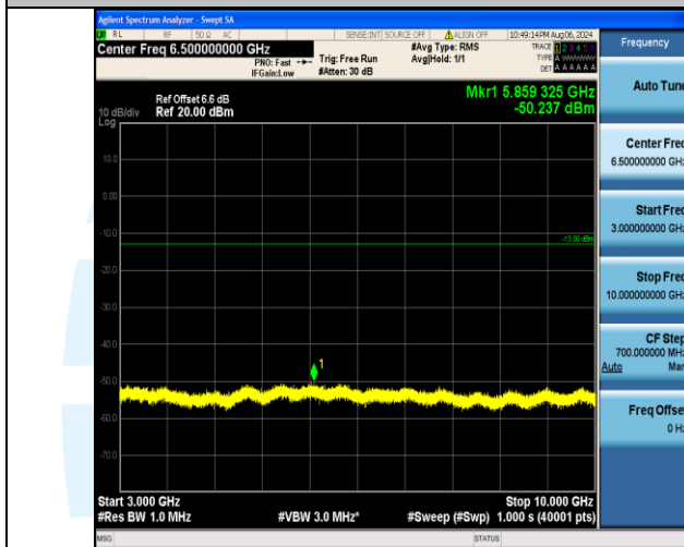
Band12_5MHz_QPSK_23155_25RB#0_3000~10000_3000~10000
