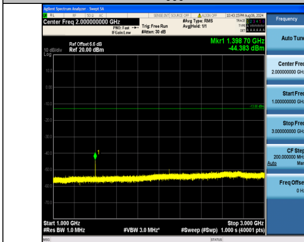
Band12_5MHz_16QAM_23035_1RB#0_1000~3000_1000~3000
