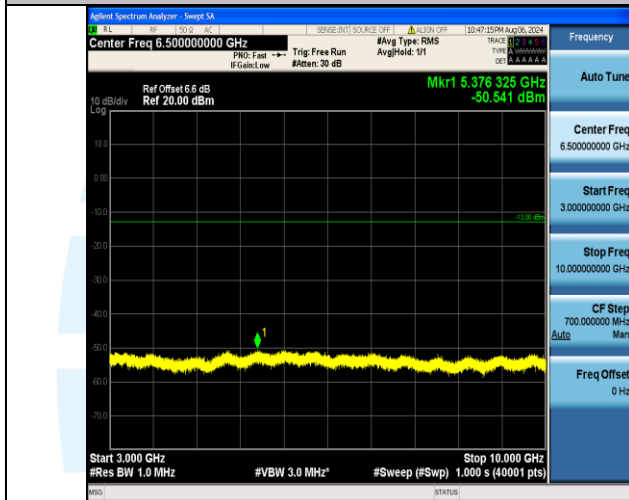
Band12_5MHz_16QAM_23095_25RB#0_3000~10000_3000~10000
