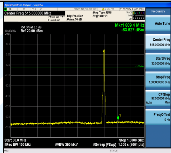
Band12_10MHz_QPSK_23095_50RB#0_30~1000_30~1000
