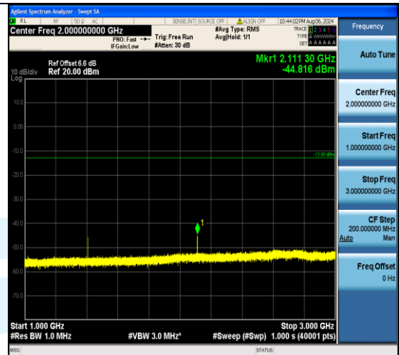
Band12_5MHz_16QAM_23035_1RB#24_1000~3000_1000~3000
