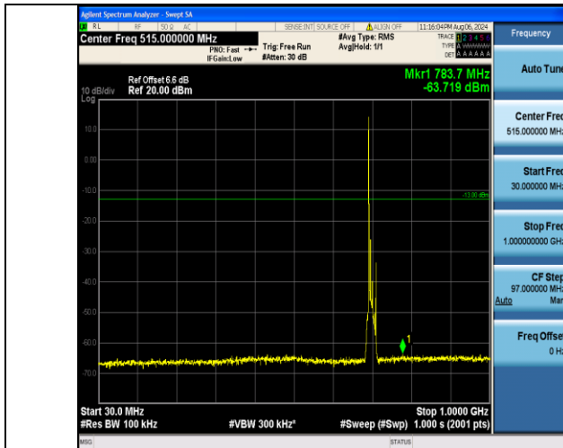
Band12_10MHz_QPSK_23060_1RB#0_30~1000_30~1000
