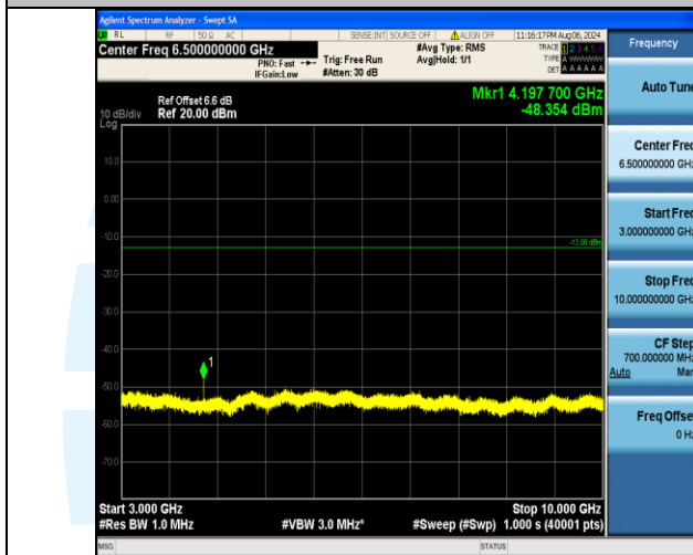
Band12_10MHz_QPSK_23060_1RB#0_3000~10000_3000~10000
