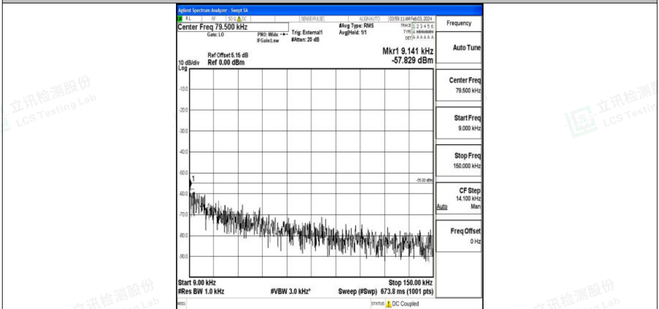
Band38_10MHz_16QAM_38200_1RB#0_0.009~0.15_0.009~0.15
