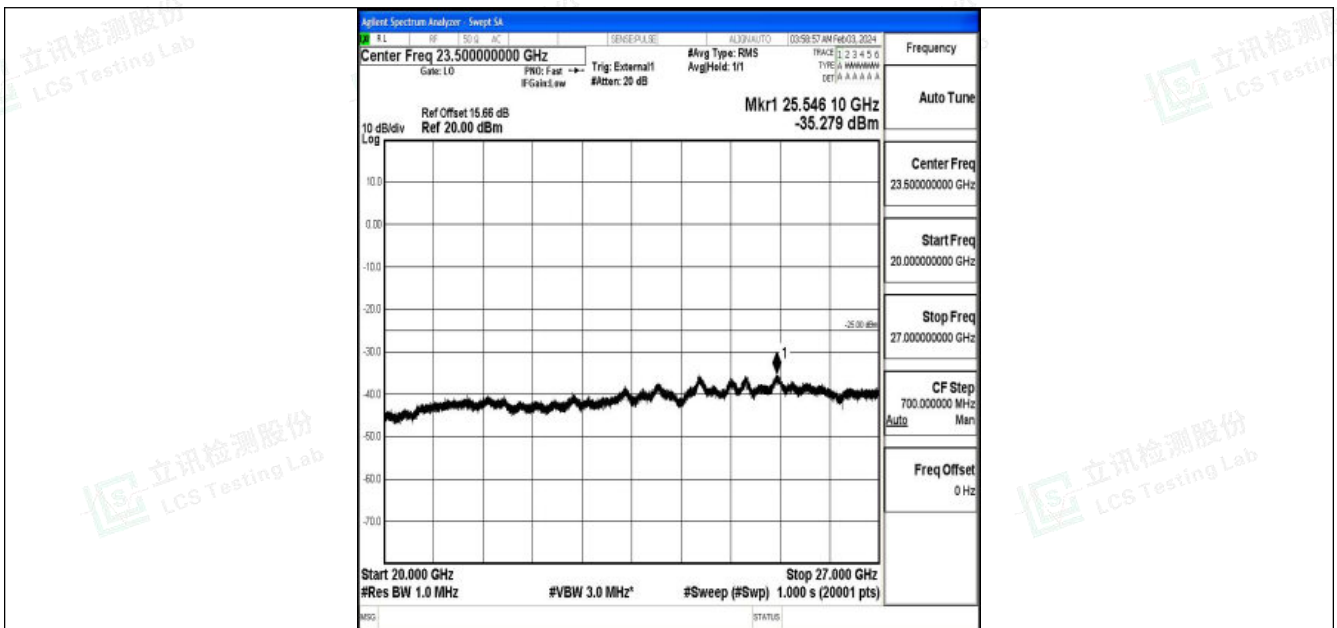
Band38_10MHz_QPSK_38200_1RB#0_20000~27000_20000~27000
