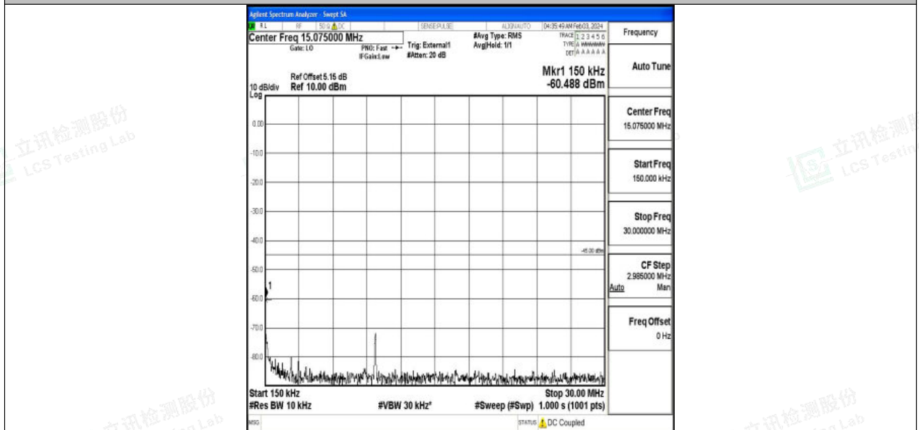
Band38_20MHz_QPSK_37850_1RB#0_0.15~30_0.15~30
