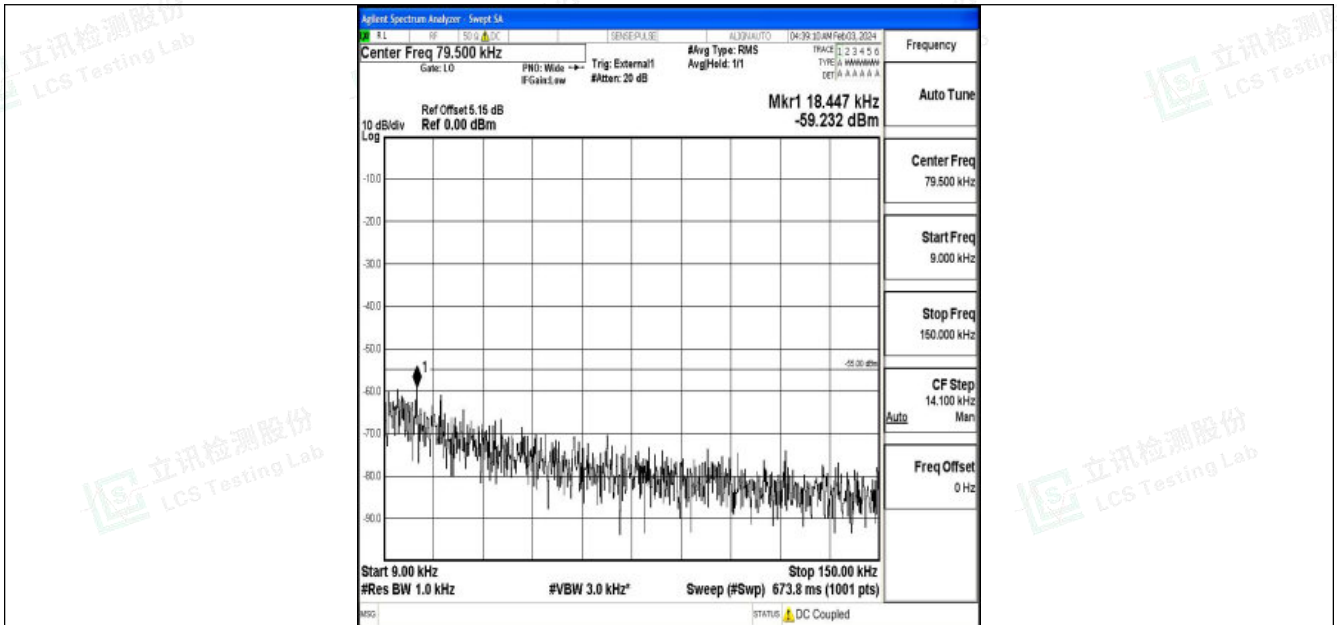
Band38_20MHz_QPSK_38000_1RB#0_0.009~0.15_0.009~0.15
