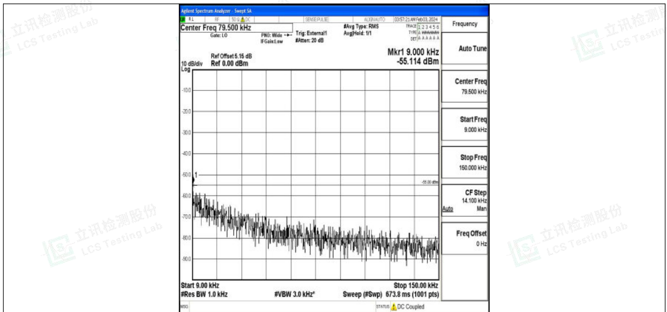
Band38_10MHz_QPSK_38200_1RB#0_0.009~0.15_0.009~0.15
