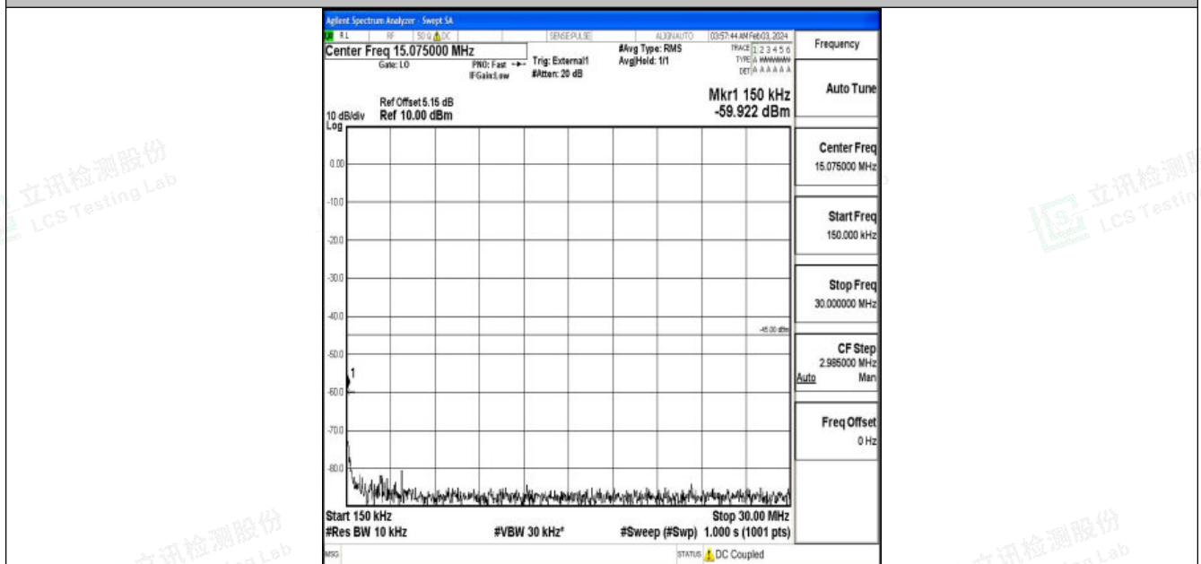
Band38_10MHz_QPSK_38200_1RB#0_0.15~30_0.15~30
