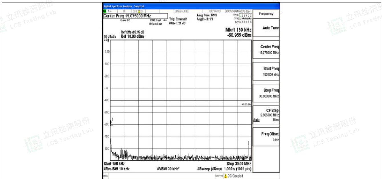
Band38_10MHz_16QAM_38000_1RB#0_0.15~30_0.15~30
