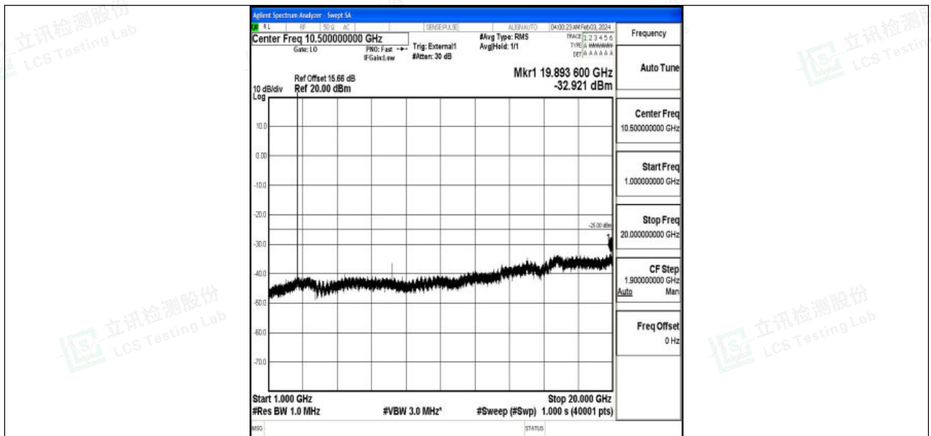
Band38_10MHz_16QAM_38200_1RB#0_1000~20000_1000~20000
