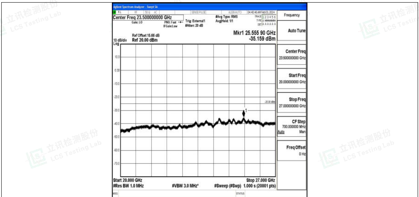
Band38_20MHz_QPSK_38000_1RB#0_20000~27000_20000~27000
