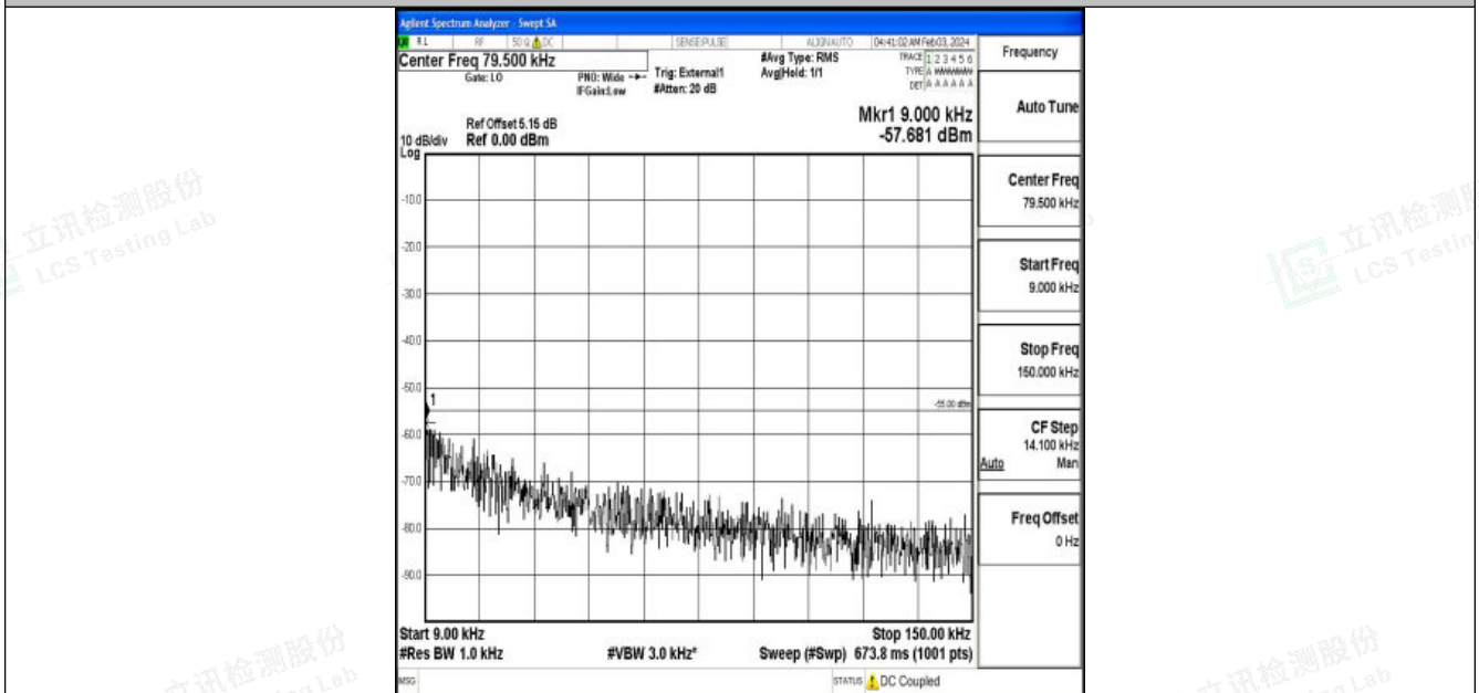
Band38_20MHz_16QAM_38000_1RB#0_0.009~0.15_0.009~0.15
