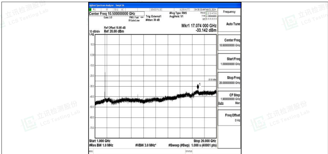
Band38_20MHz_16QAM_37850_1RB#0_1000~20000_1000~20000
