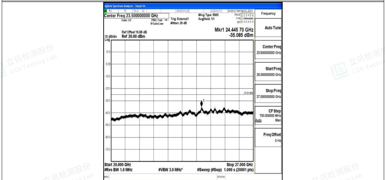
Band38_10MHz_16QAM_38200_1RB#0_20000~27000_20000~27000
