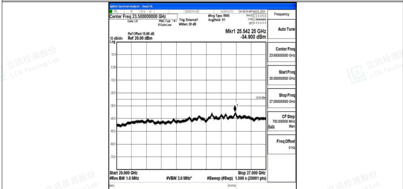
Band38_20MHz_16QAM_37850_1RB#0_20000~27000_20000~27000
