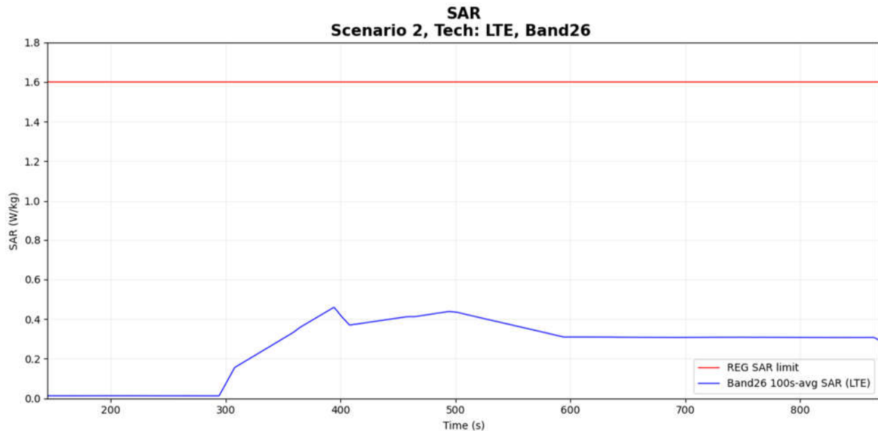
Figure 7-6 Time-averaged SAR
