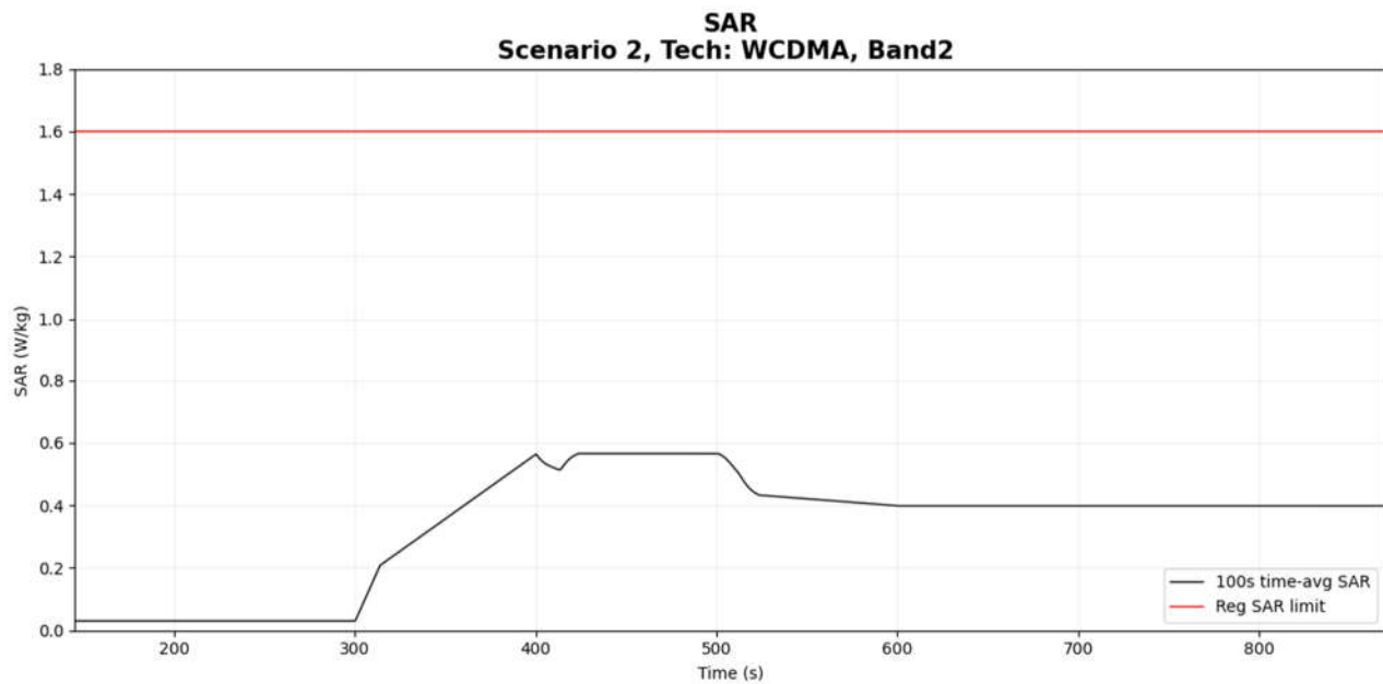
Figure 6- 7 Time-averaged SAR
