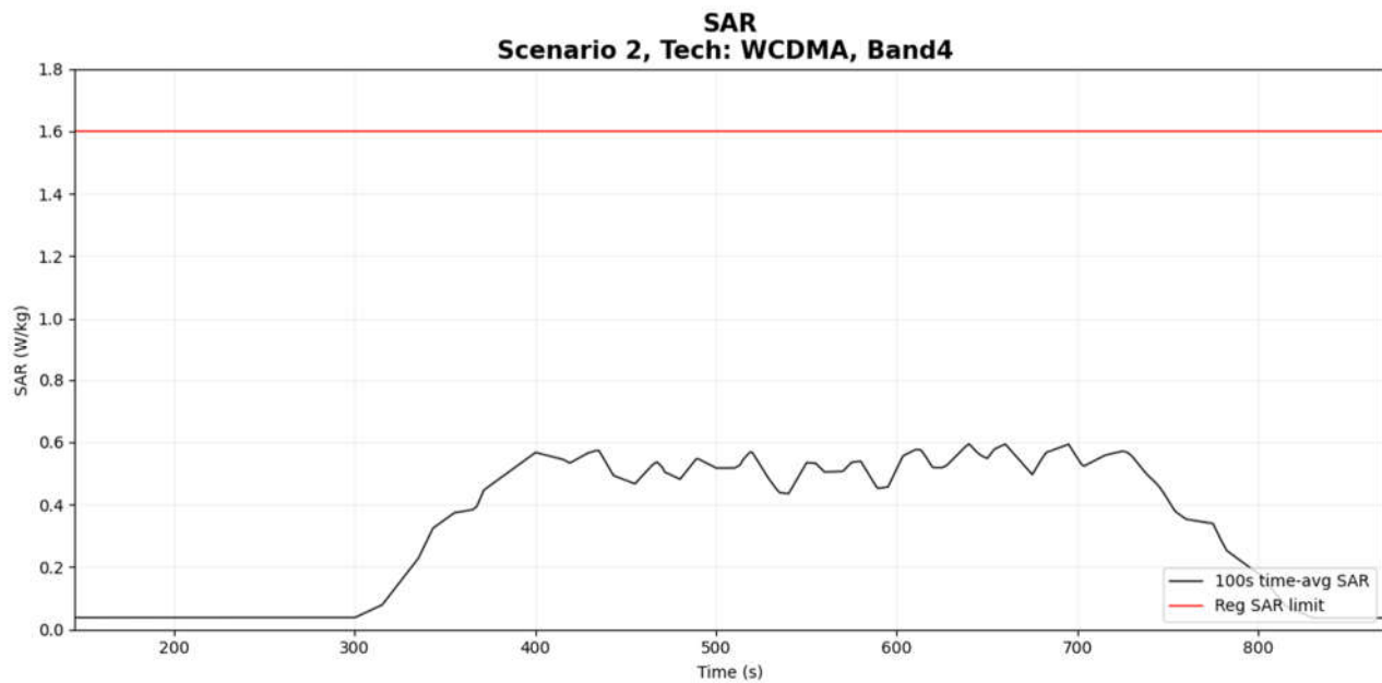
Figure 6- 6 Time-averaged SAR
