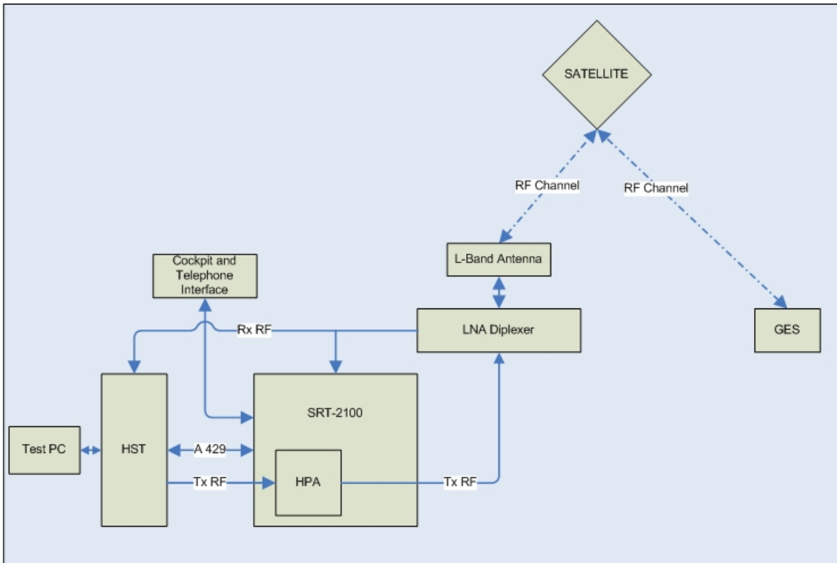
Figure 1 - RF Power Output Test Setup
