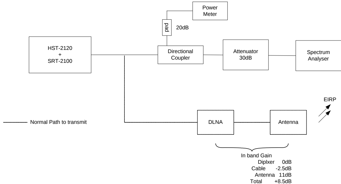
Figure 5 - Occupied Bandwidth Test Setup
