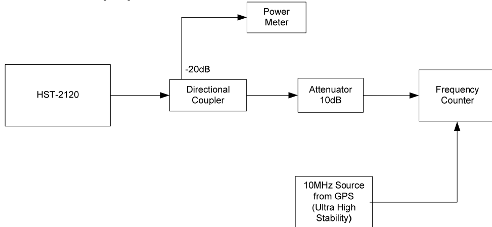
Figure 13 Frequency Stability Test Setup
