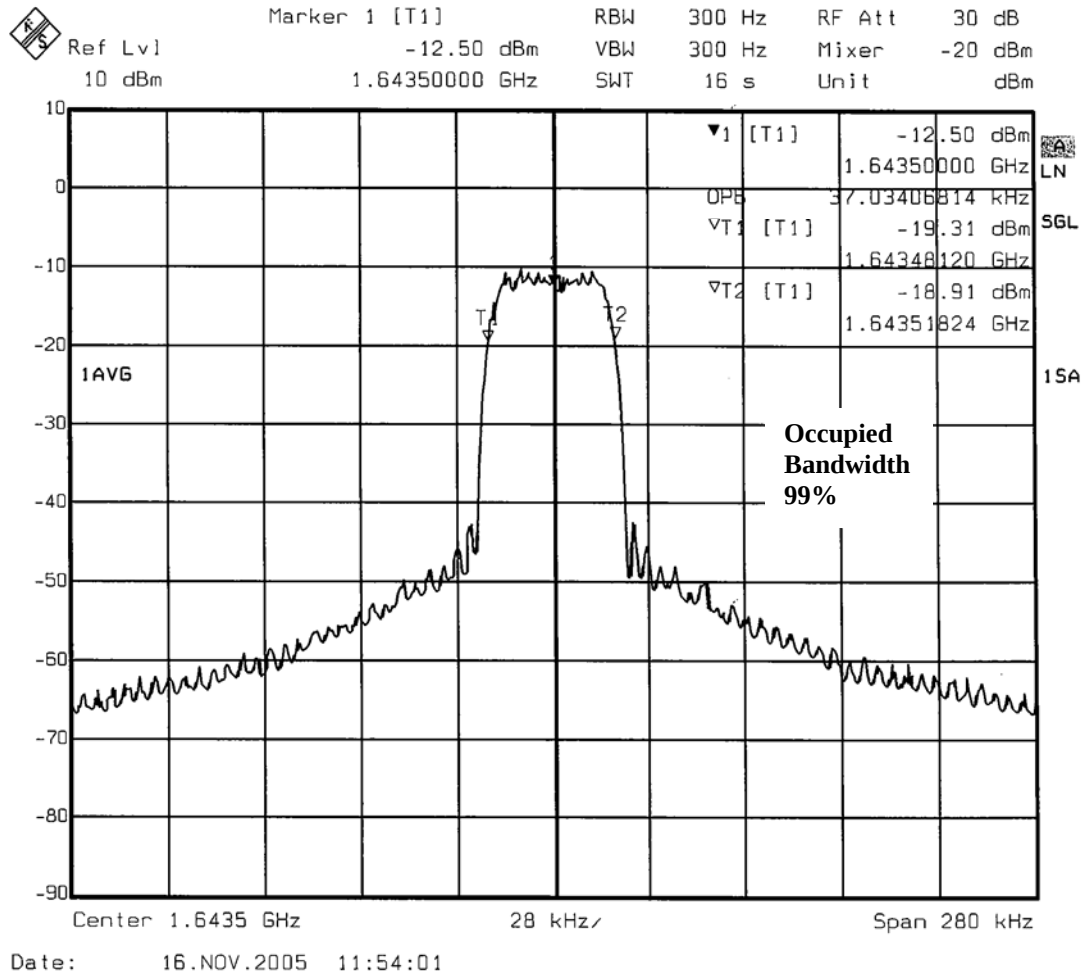
Figure 7 – Occupied Bandwidth 134400 bps
