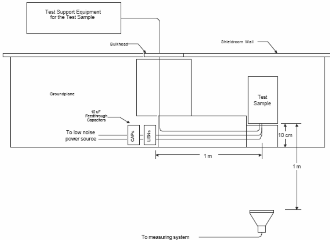
Figure 12 Field Strength Test Setup
