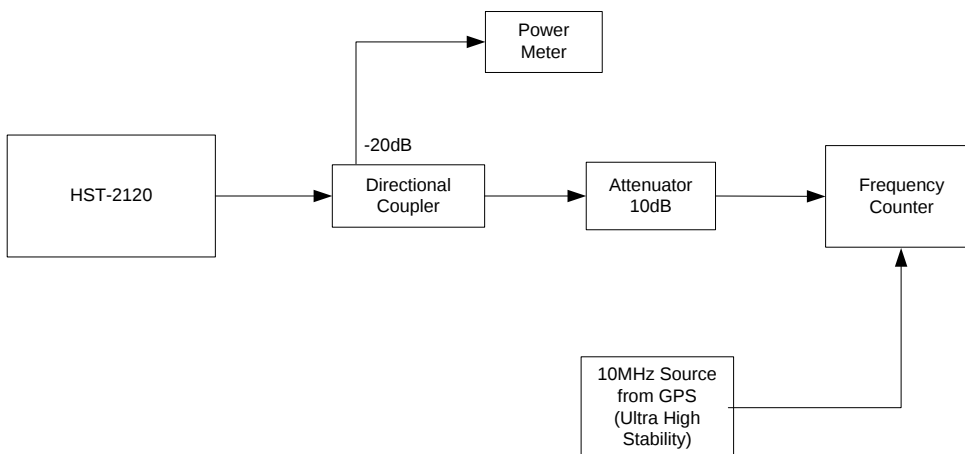
Figure 14 Frequency Stability Test Setup
