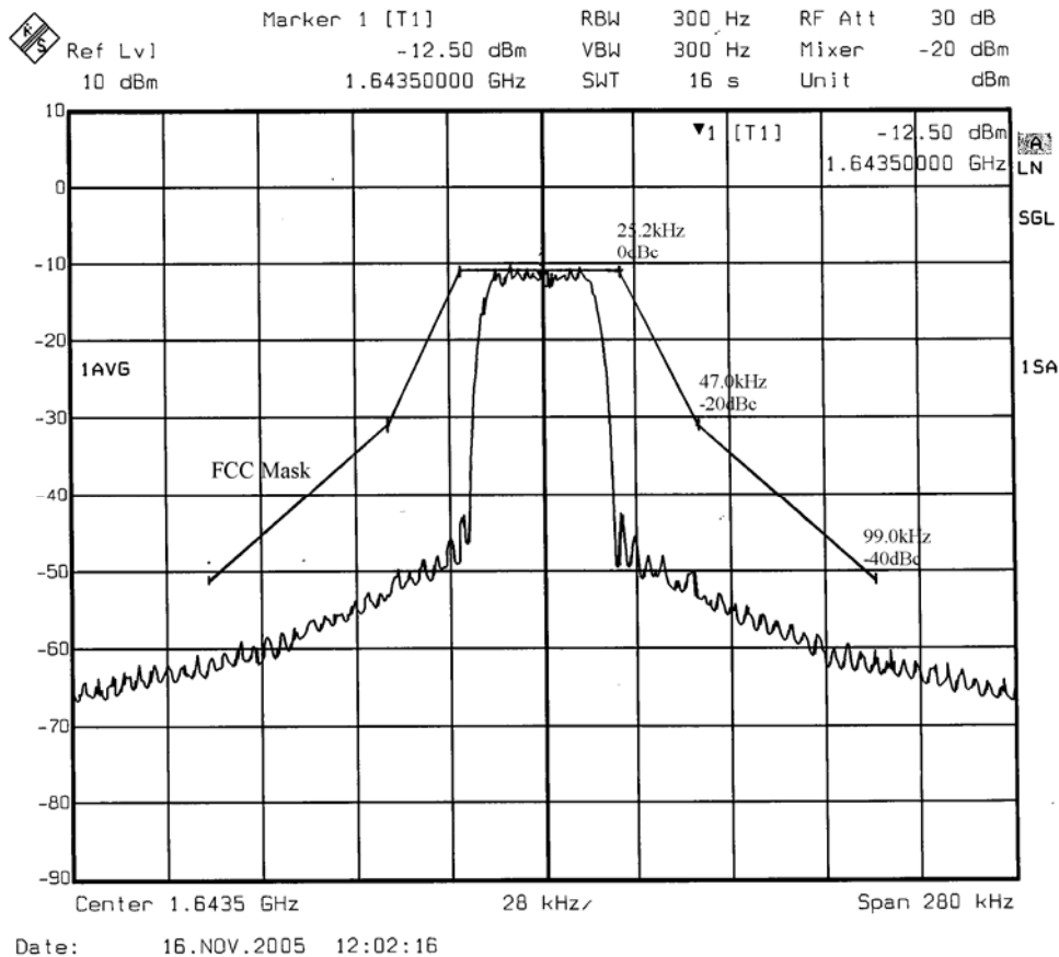
Figure 11 – 134400 bps 16-QAM Transmitter Spectrum
