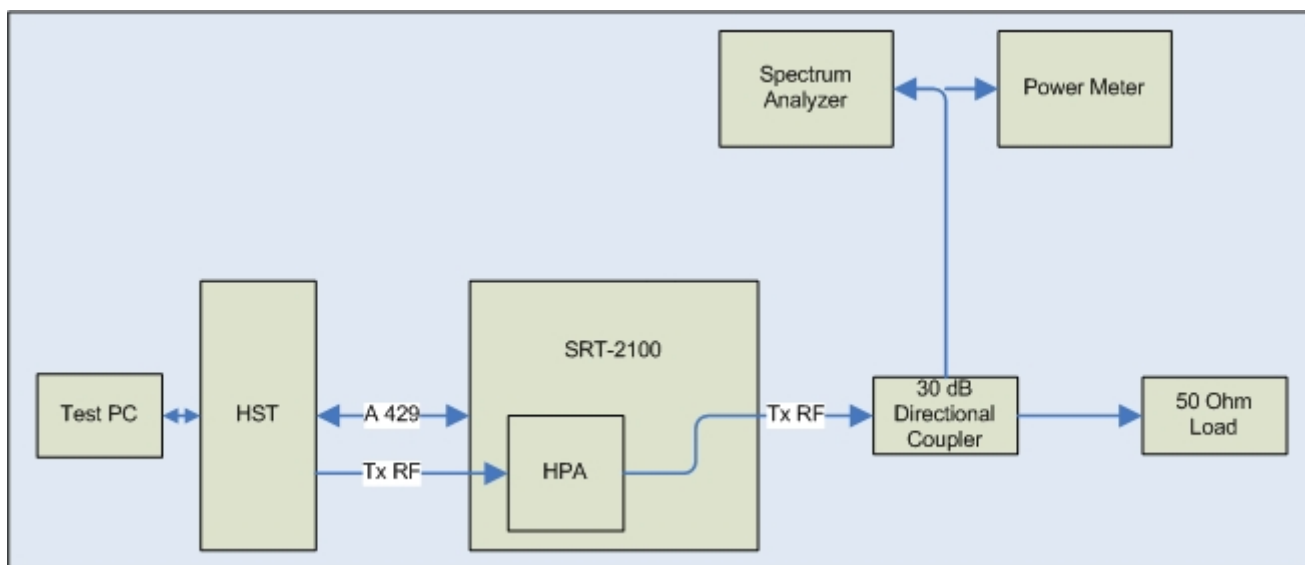
Figure 8 - Spurious Emissions Test Setup
