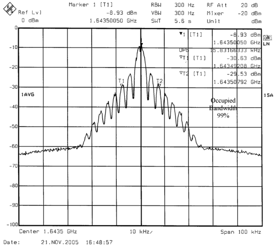
Figure 6 – Occupied Bandwidth 3000 bps
