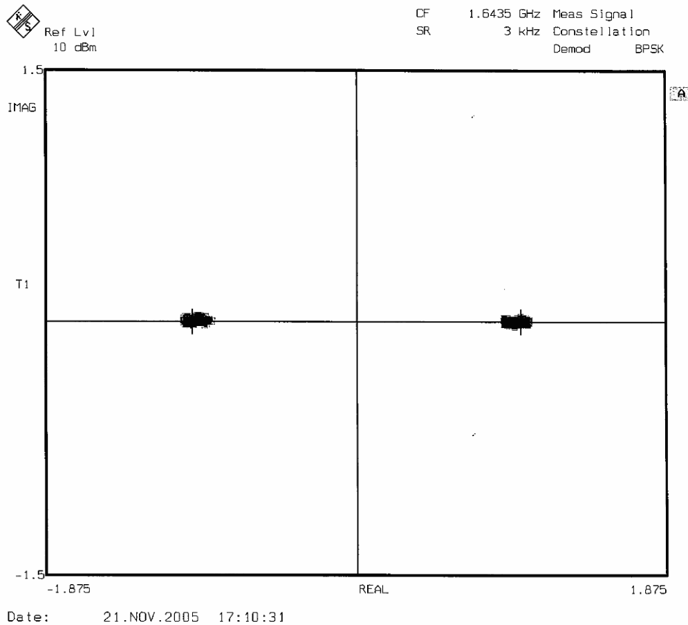
Figure 3 - 3000 bps BPSK I/Q Diagram
