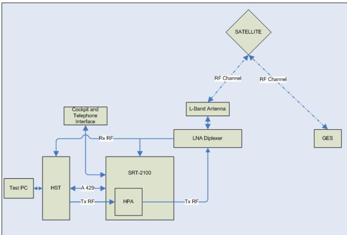
Figure 15 - Priority/Preemption Test Setup
