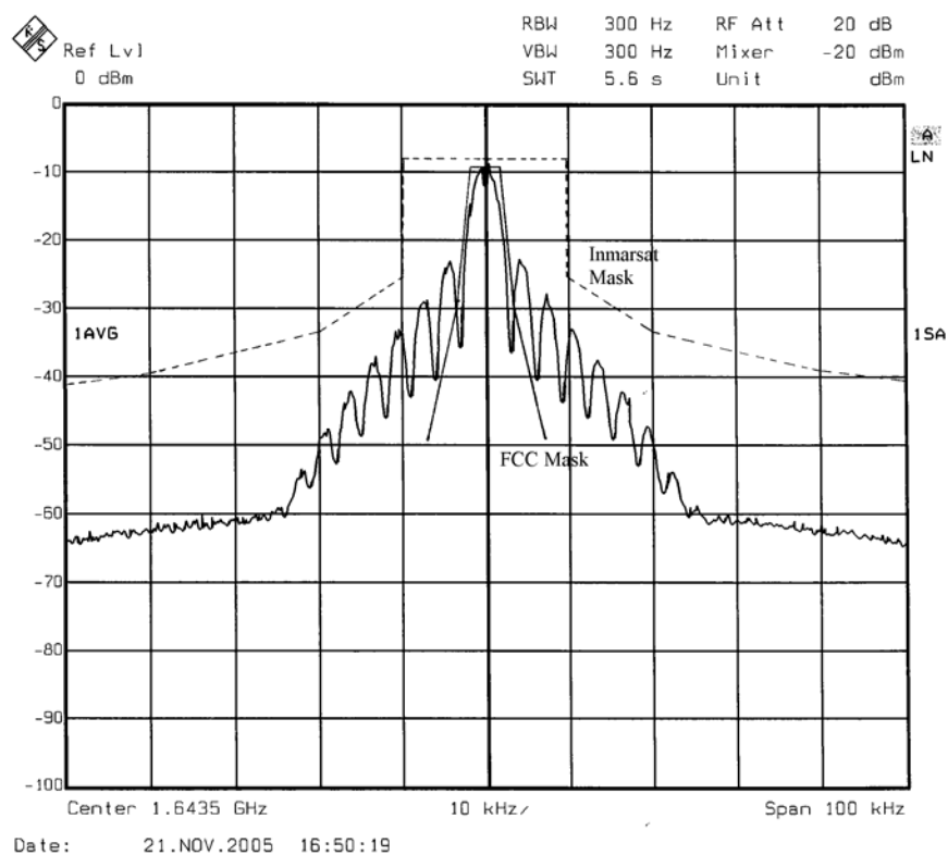
Figure 10 – 3000bps BPSK Transmitter Spectrum
