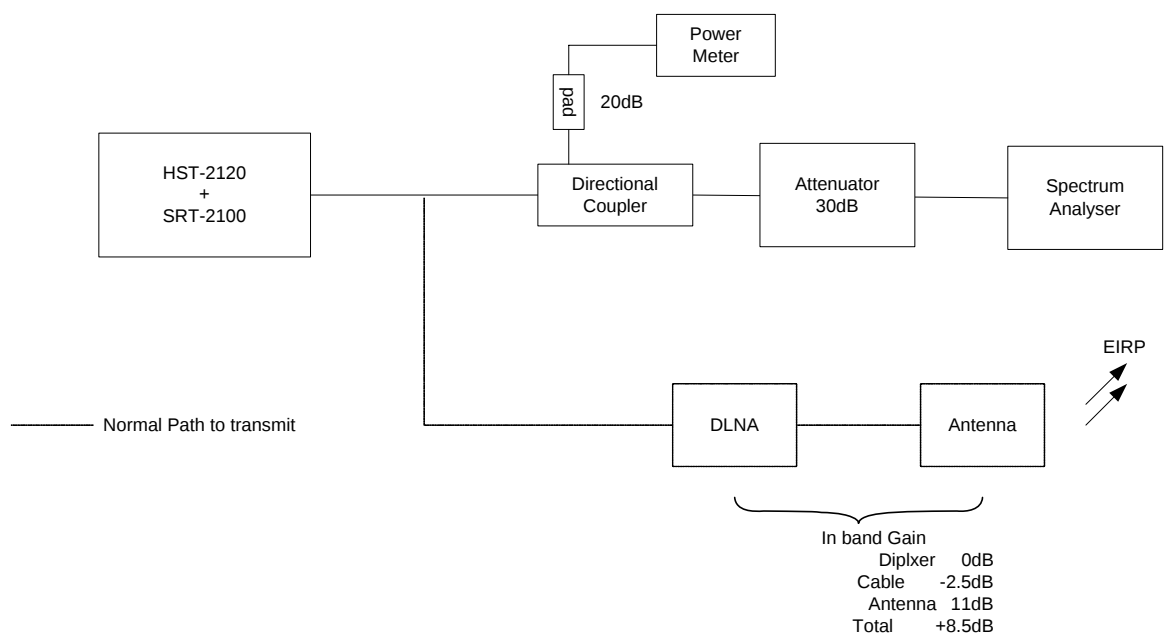
Figure 9 - Frequency Spectrum Test Setup
