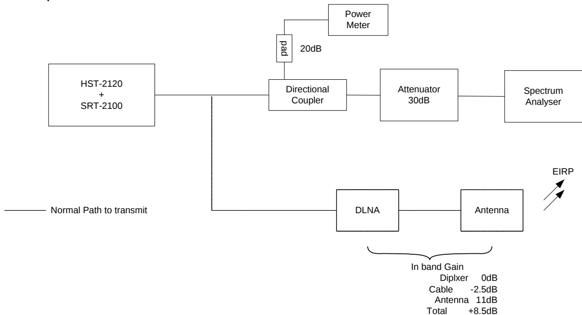
Figure 2 - Modulation Characteristics Test Setup
