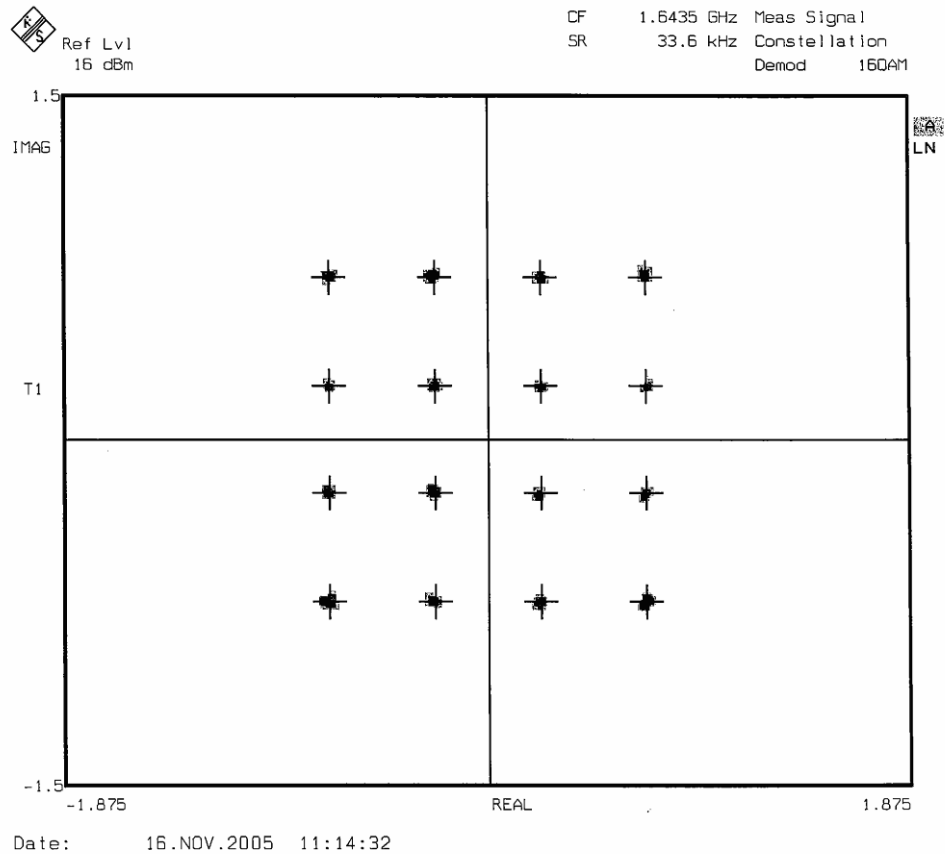
Figure 4 – 134400 bps 16-QAM I/Q Diagram
