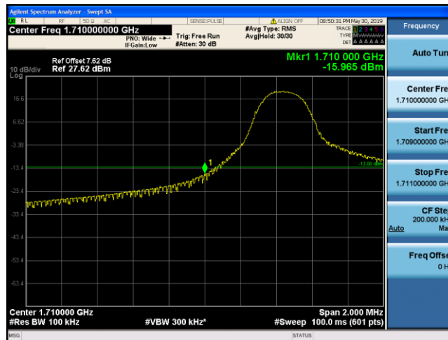
Band4_5MHz_QPSK_19975_1RB#0
