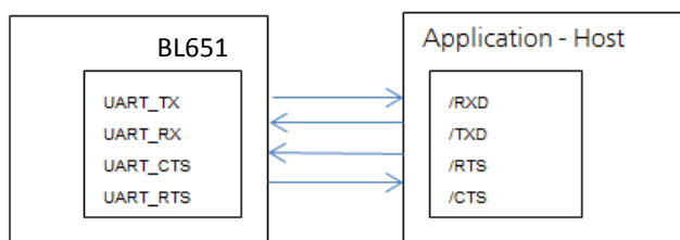
Figure 3: UART signals
