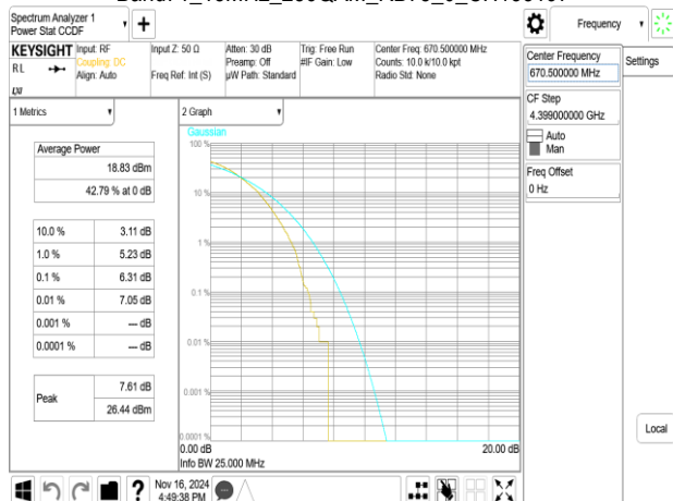
Band71_15MHz_256QAM_RB75_0_CH133297
