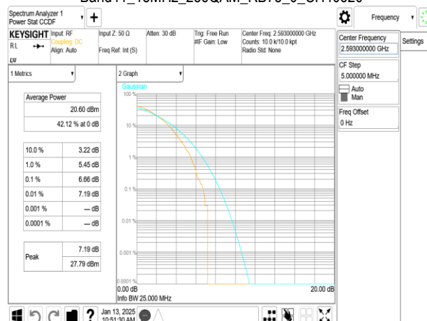
Band41_15MHz_256QAM_RB75_0_CH40620
