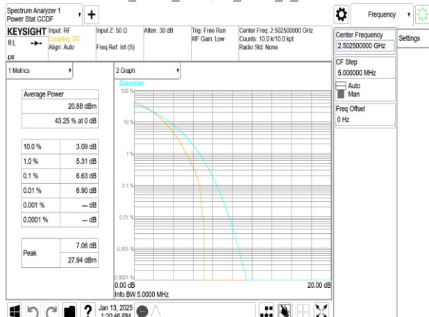
Band41_5MHz_256QAM_RB25_0_CH39715
