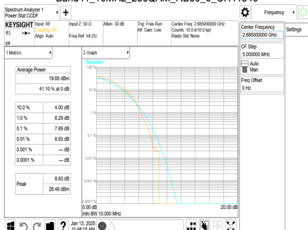
Band41_10MHz_256QAM_RB50_0_CH41540
