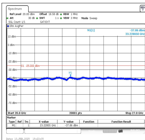
Band41_10MHz_QPSK_40620_1RB#0_20000~27000
