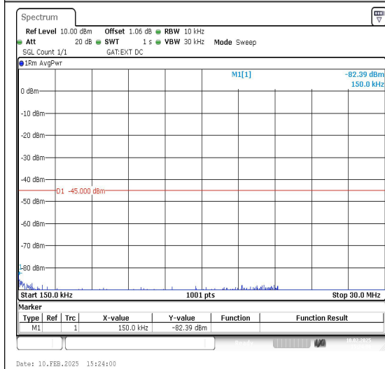
Band41_10MHz_QPSK_40620_1RB#0_0.15~3
