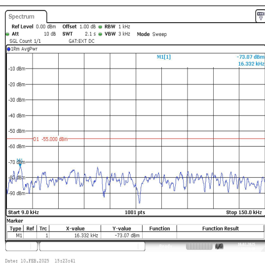
Band41_10MHz_16QAM_40620_1RB#0_0.009~0.15
