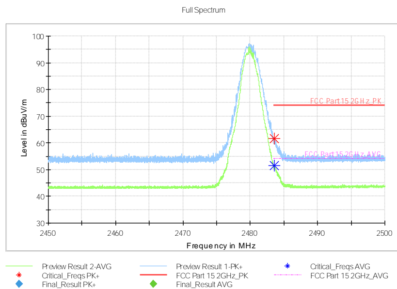
Fig.63. Frequency Band Edges: 8DPSK, Channel 78, 2.45 GHz - 2.50GHz
