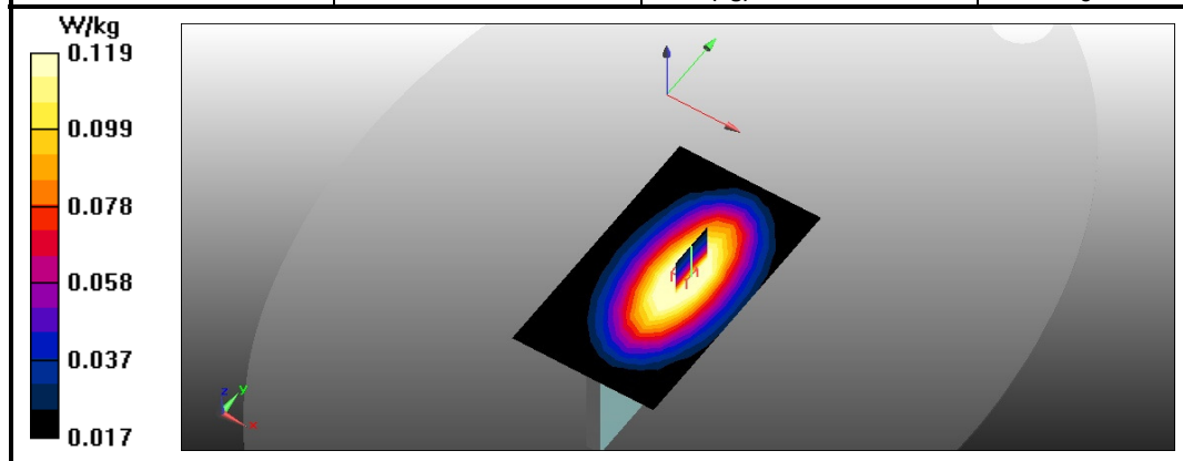
Figure 39: SAR Head Testing Results for the Sharp Smart phone at 709.0 MHz.
