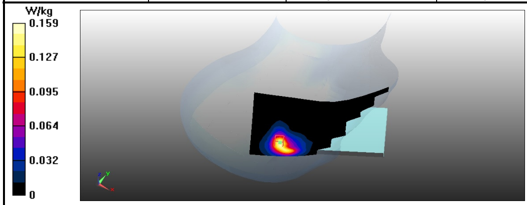
Figure 61: SAR Head Testing Results for the Sharp Smart phone at 2437 MHz.
