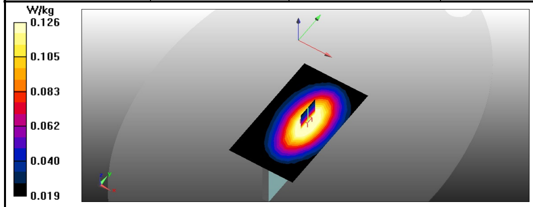
Figure 38: SAR Head Testing Results for the Sharp Smart phone at 709.0 MHz.
