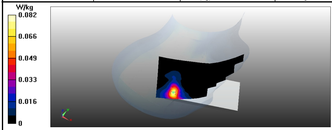
Figure 62: SAR Head Testing Results for the Sharp Smart phone at 2437 MHz.
