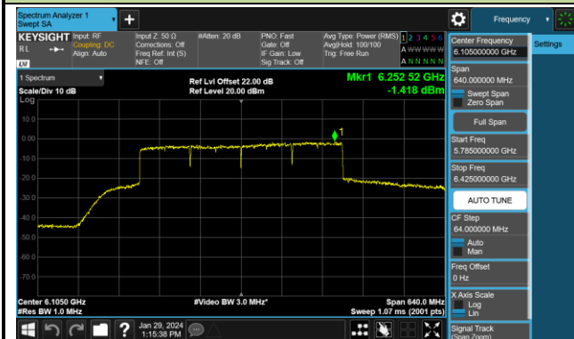
Channel 95 (6425MHz)
