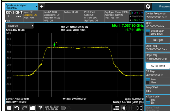
Channel 229 (7095MHz)
