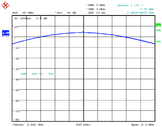
3DH1_Middle 3.79dBm
