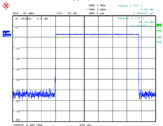
DH5_Hopping 2.956ms
