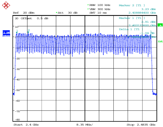
DH1_Hopping 79
