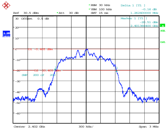
3DH1_Low 1.262MHz
