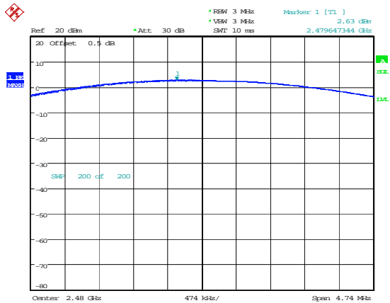
DH1_High 2.63dBm
