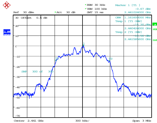
3DH1_Middle 1.162MHz
