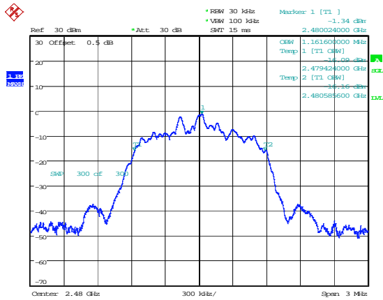
3DH1_High 1.162MHz
