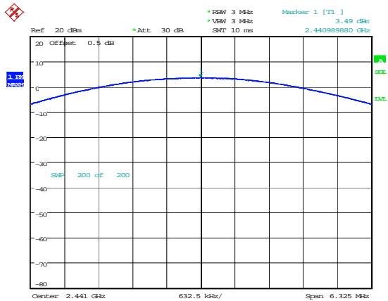
2DH1_Middle 3.49dBm
