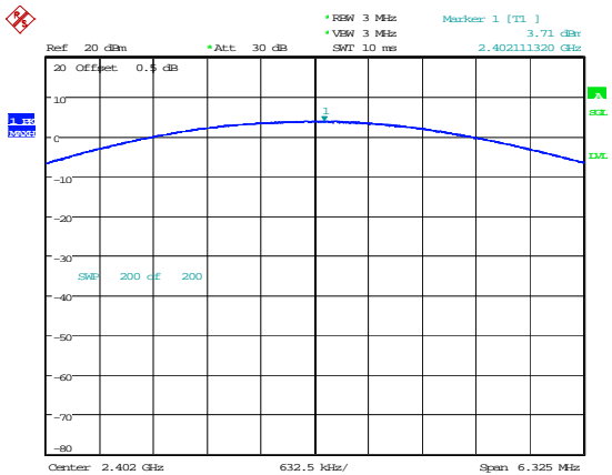
2DH1_Low 3.71dBm
