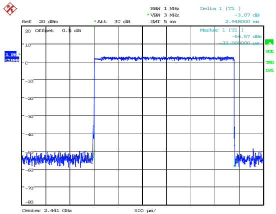
2DH5_Hopping 2.948ms
