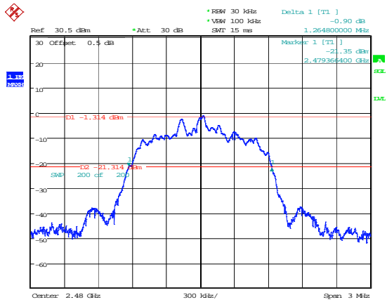
3DH1_High 1.265MHz
