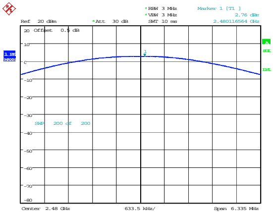
2DH1_High 2.76dBm
