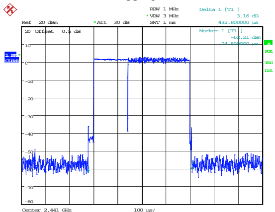
2DH1_Hopping 0.433ms
