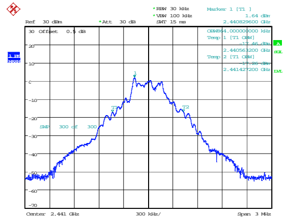
DH1_Middle 0.864MHz
