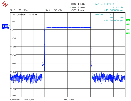
DH1_Hopping 0.440ms
