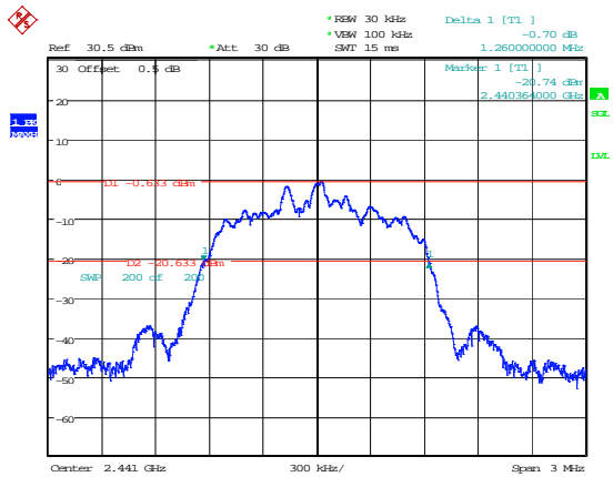
3DH1_Middle 1.260MHz
