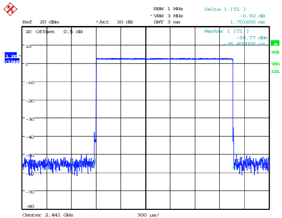
DH3_Hopping 1.702ms
