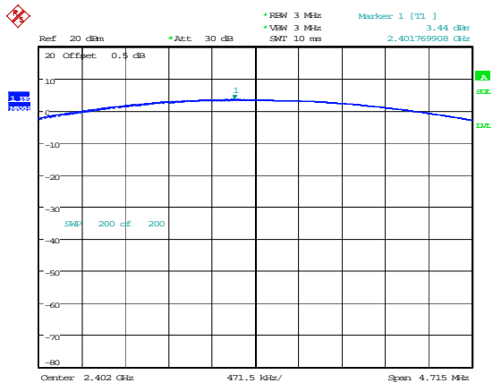
DH1_Low 3.44dBm
