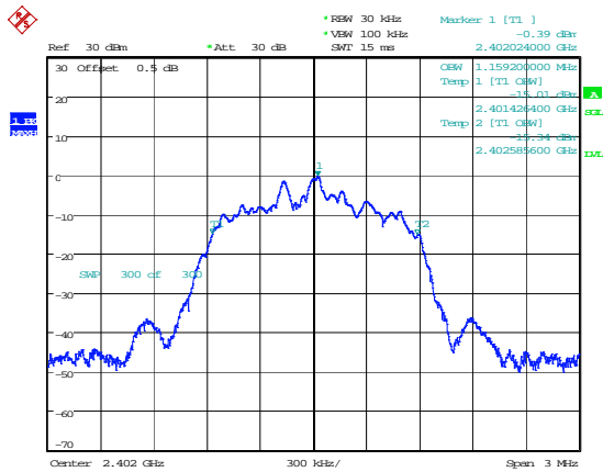
3DH1_Low 1.159MHz
