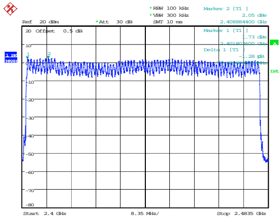
3DH1_Hopping 79
