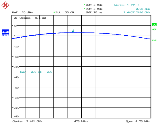
DH1_Middle 2.98dBm
