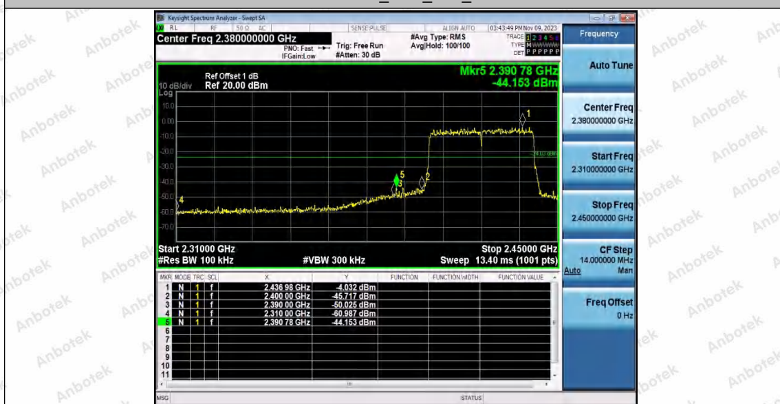
11AX40SISO_Ant1_High_2452
