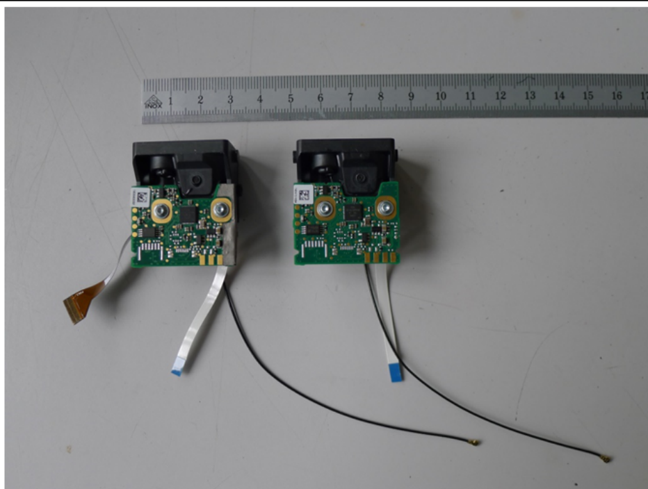
EUT INTERNAL DETAIL (E)
