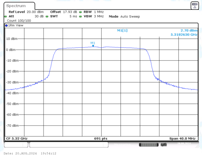
11AX20SISO-Ant3-5320-PASS
