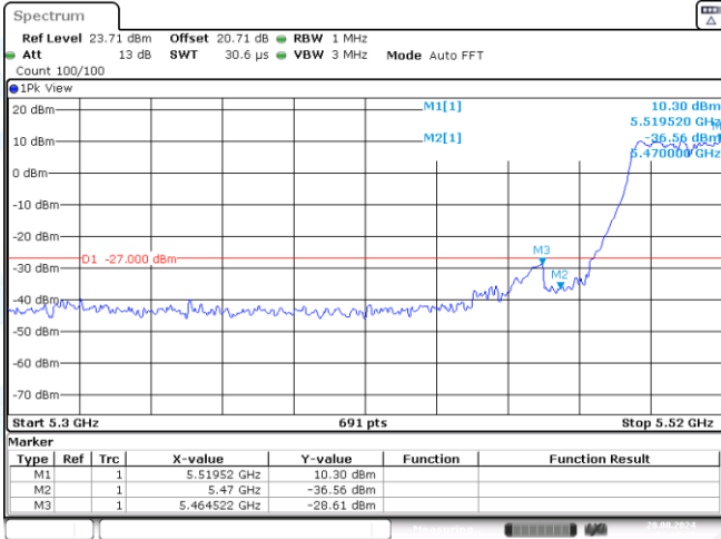
11AC40SISO-Ant3-5510-PASS
