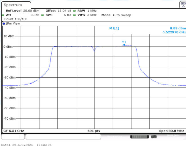
11N40SISO-Ant3-5510-PASS
