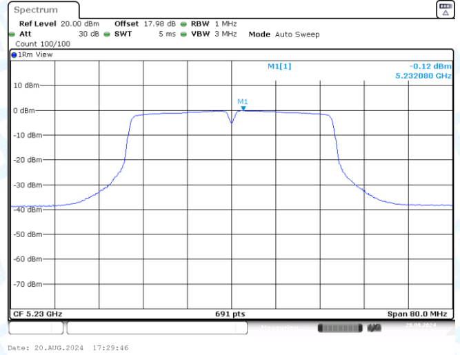
11N40SISO-Ant3-5230-PASS
