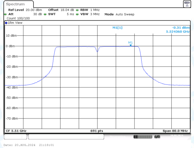
11AC40SISO-Ant3-5510-PASS
