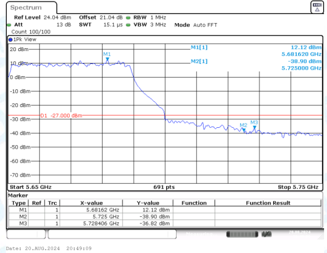
11AX40SISO-Ant3-5670-PASS
