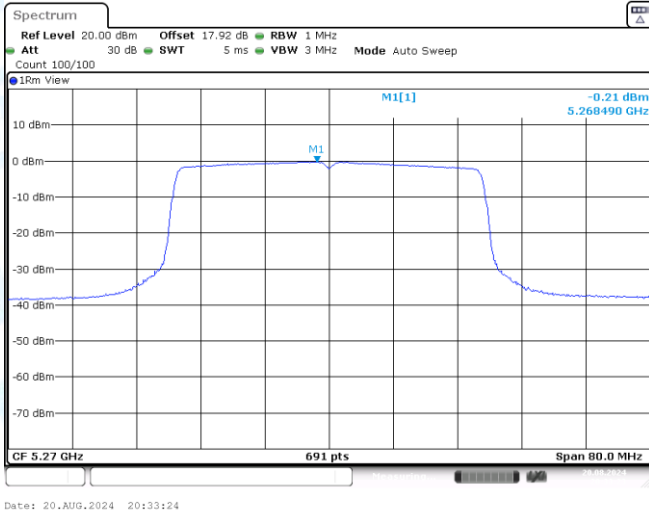
11AX40SISO-Ant3-5270-PASS
