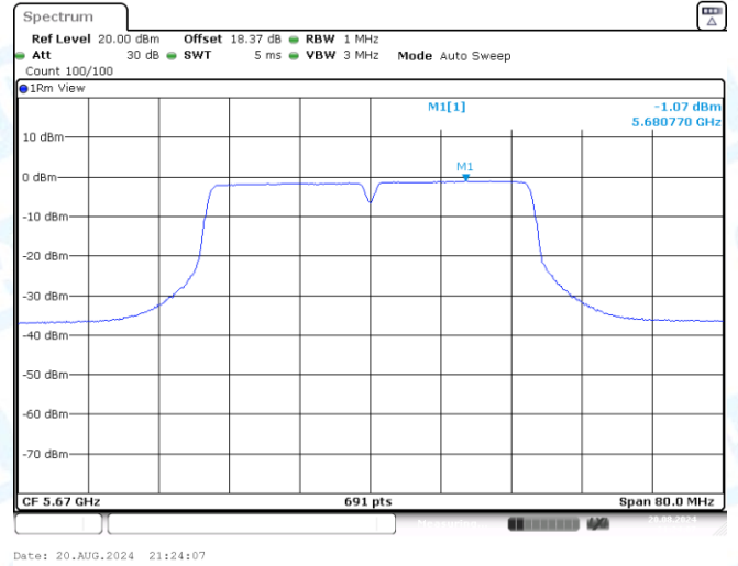
11AC40SISO-Ant3-5670-PASS
