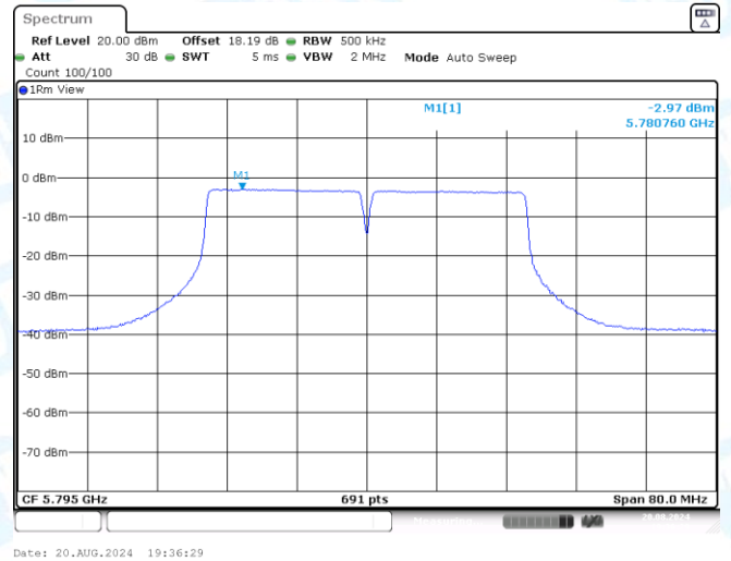
11AC40SISO-Ant3-5795-PASS
