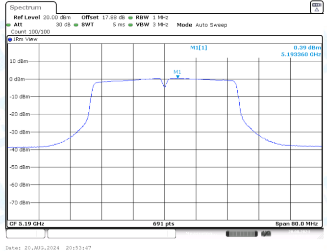
11AC40SISO-Ant3-5190-PASS
