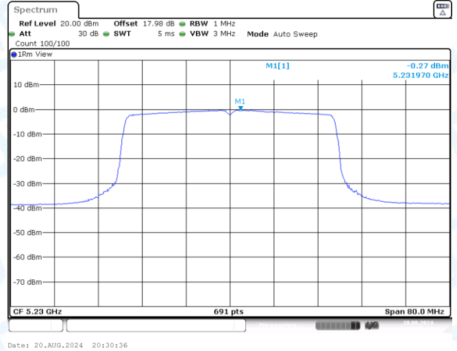
11AX40SISO-Ant3-5230-PASS
