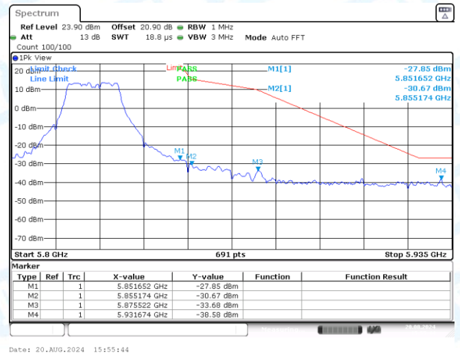
11A-Ant3-5825-PASS
