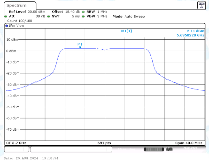
11AC20SISO-Ant3-5700-PASS
