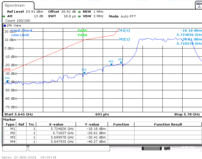
11N40SISO-Ant3-5755-PASS
