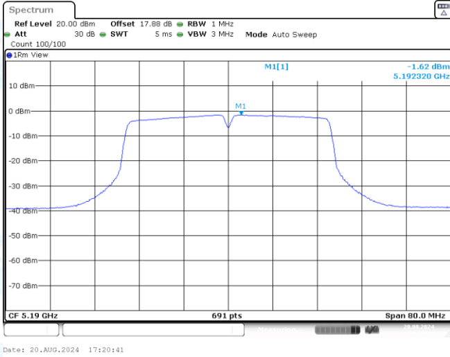
11N40SISO-Ant3-5190-PASS
