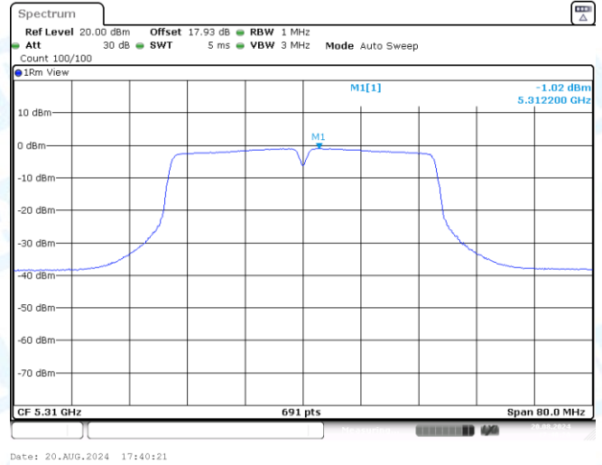
11N40SISO-Ant3-5310-PASS
