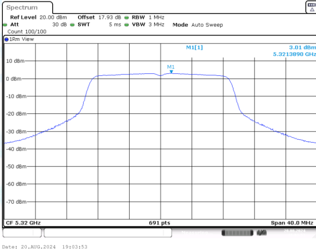
11AC20SISO-Ant3-5320-PASS
