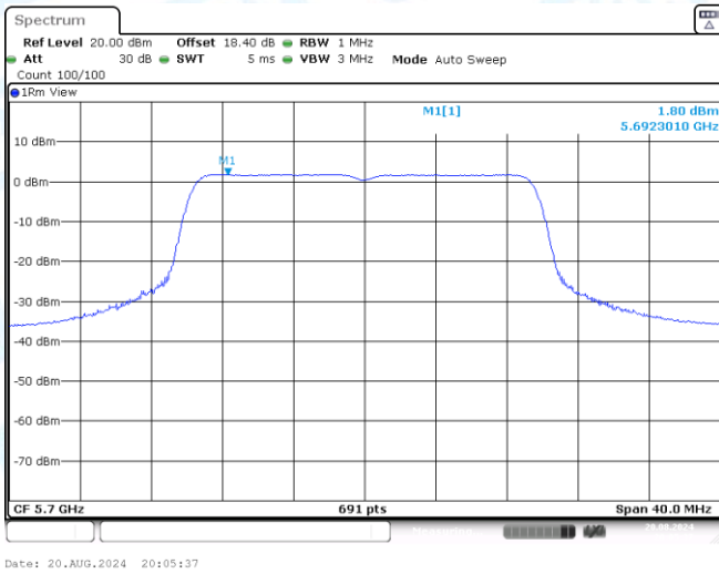
11AX20SISO-Ant3-5700-PASS
