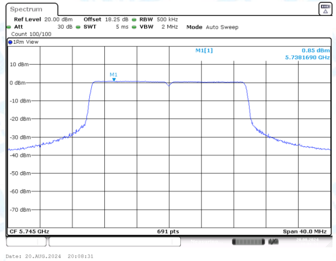
11AX20SISO-Ant3-5745-PASS
