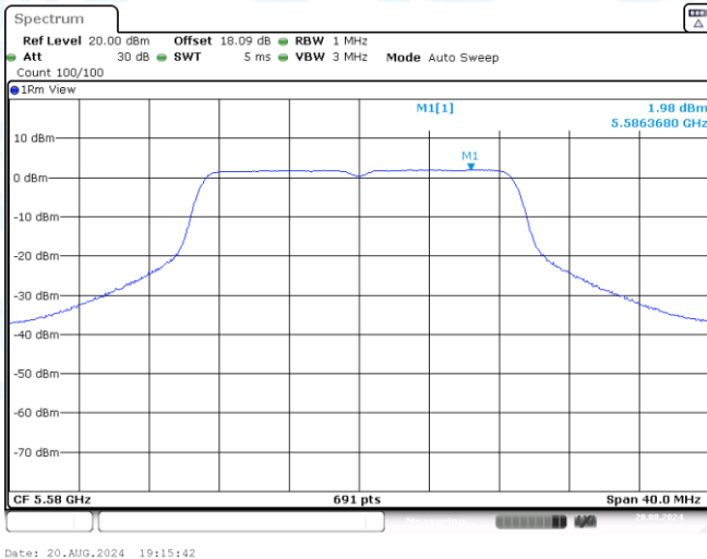
11AC20SISO-Ant3-5580-PASS
