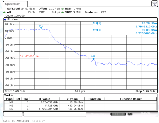
11A-Ant3-5700-PASS
