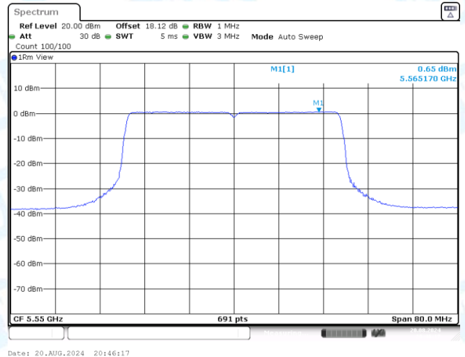
11AX40SISO-Ant3-5550-PASS
