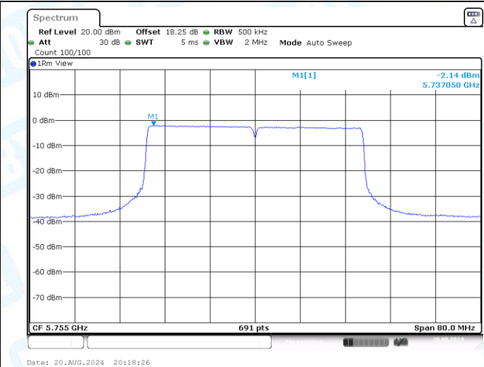
11AX40SISO-Ant3-5755-PASS
