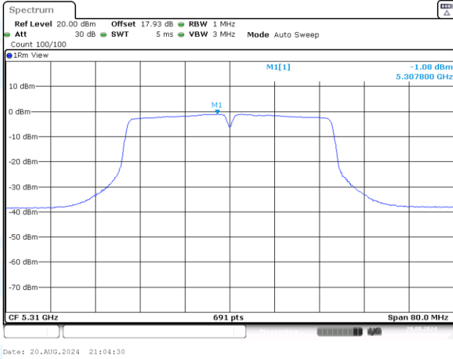
11AC40SISO-Ant3-5310-PASS
