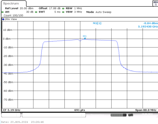
11AX40SISO-Ant3-5190-PASS
