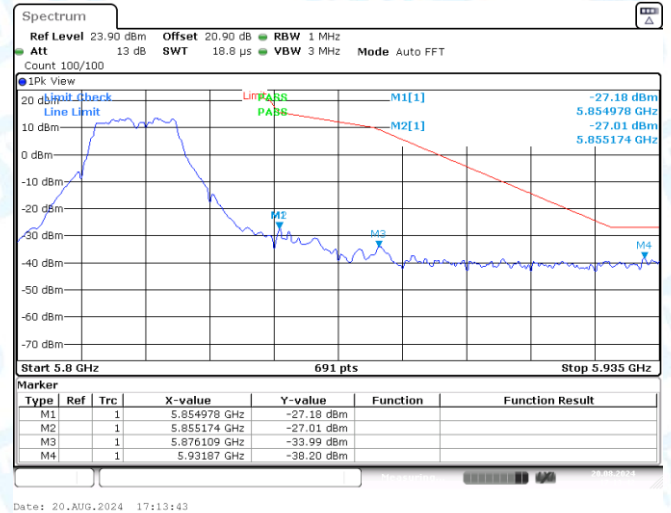
11N20SISO-Ant3-5825-PASS
