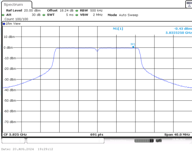
11AC20SISO-Ant3-5825-PASS
