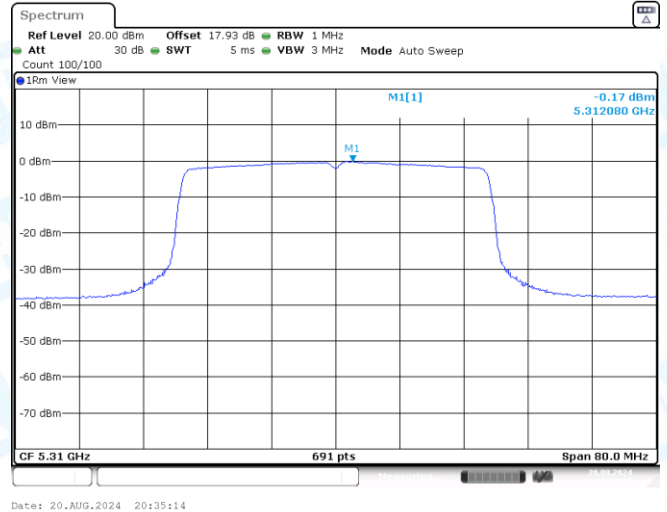
11AX40SISO-Ant3-5310-PASS
