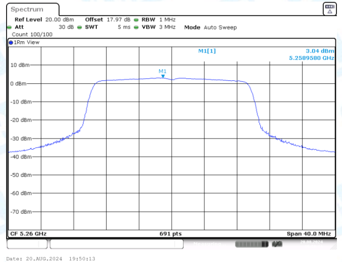
11AX20SISO-Ant3-5260-PASS
