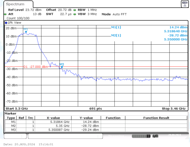
11A-Ant3-5320-PASS
