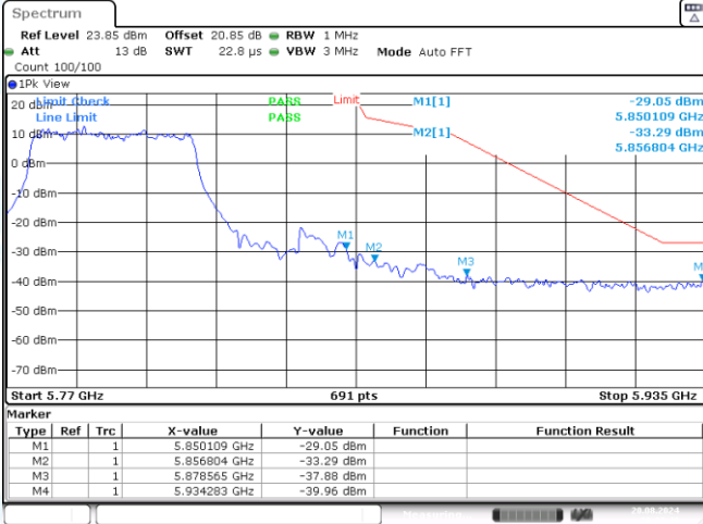
11AX40SISO-Ant3-5795-PASS
