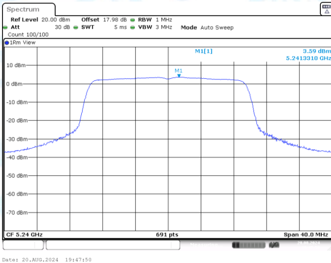
11AX20SISO-Ant3-5240-PASS
