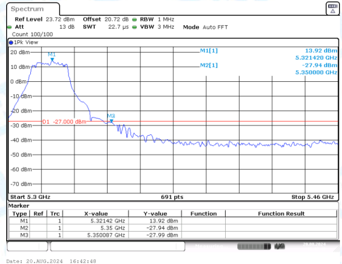
11N20SISO-Ant3-5320-PASS
