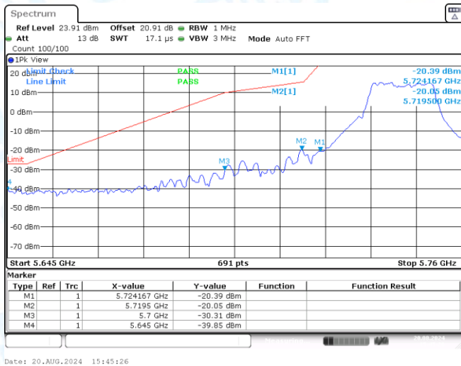
11A-Ant3-5745-PASS
