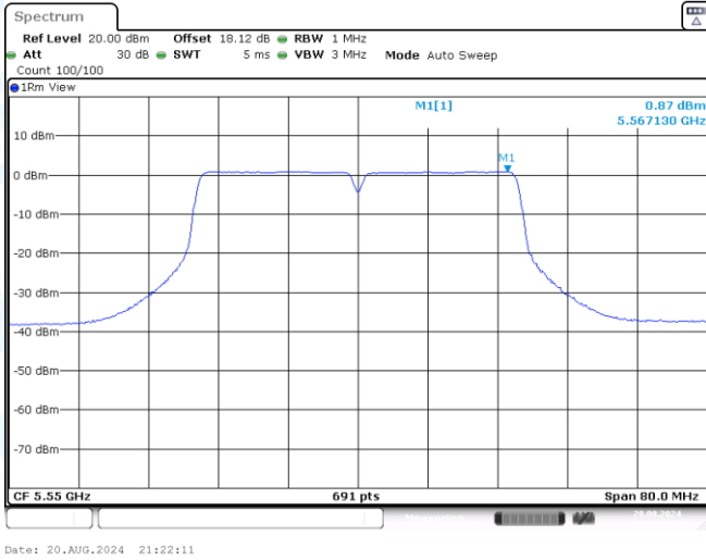
11AC40SISO-Ant3-5550-PASS
