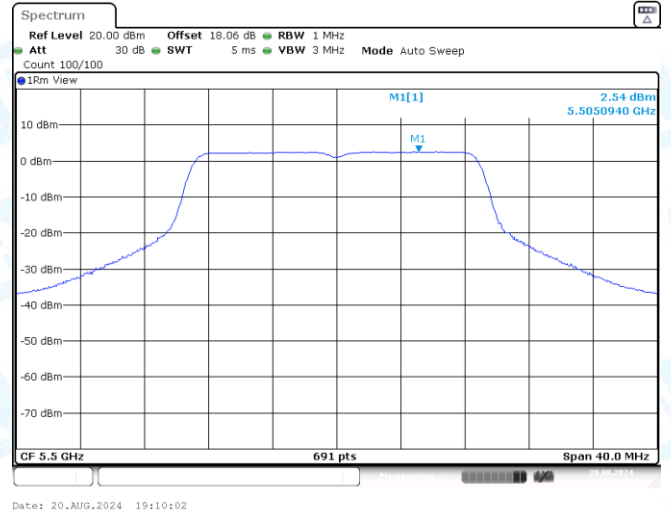
11AC20SISO-Ant3-5500-PASS
