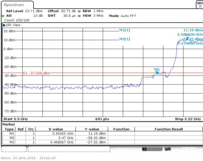
11AX40SISO-Ant3-5510-PASS
