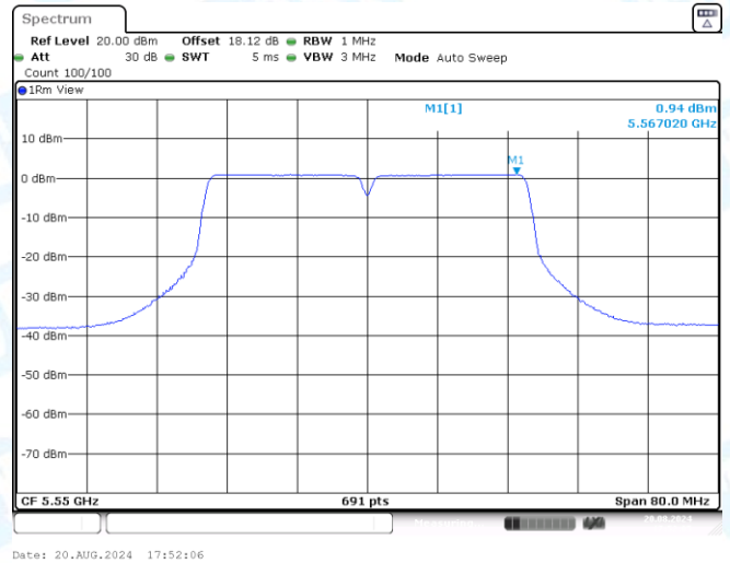
11N40SISO-Ant3-5550-PASS
