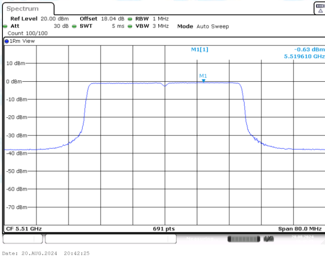
11AX40SISO-Ant3-5510-PASS
