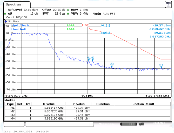
11N40SISO-Ant3-5795-PASS
