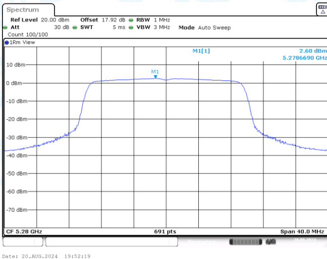
11AX20SISO-Ant3-5280-PASS
