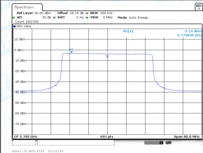
11AX40SISO-Ant3-5795-PASS
