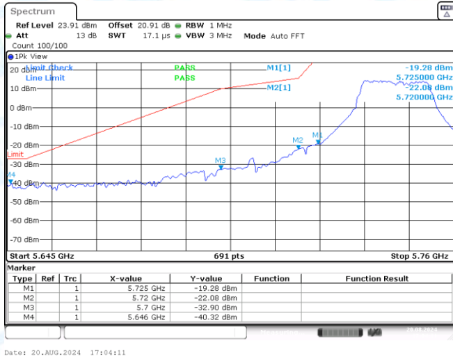
11N20SISO-Ant3-5745-PASS
