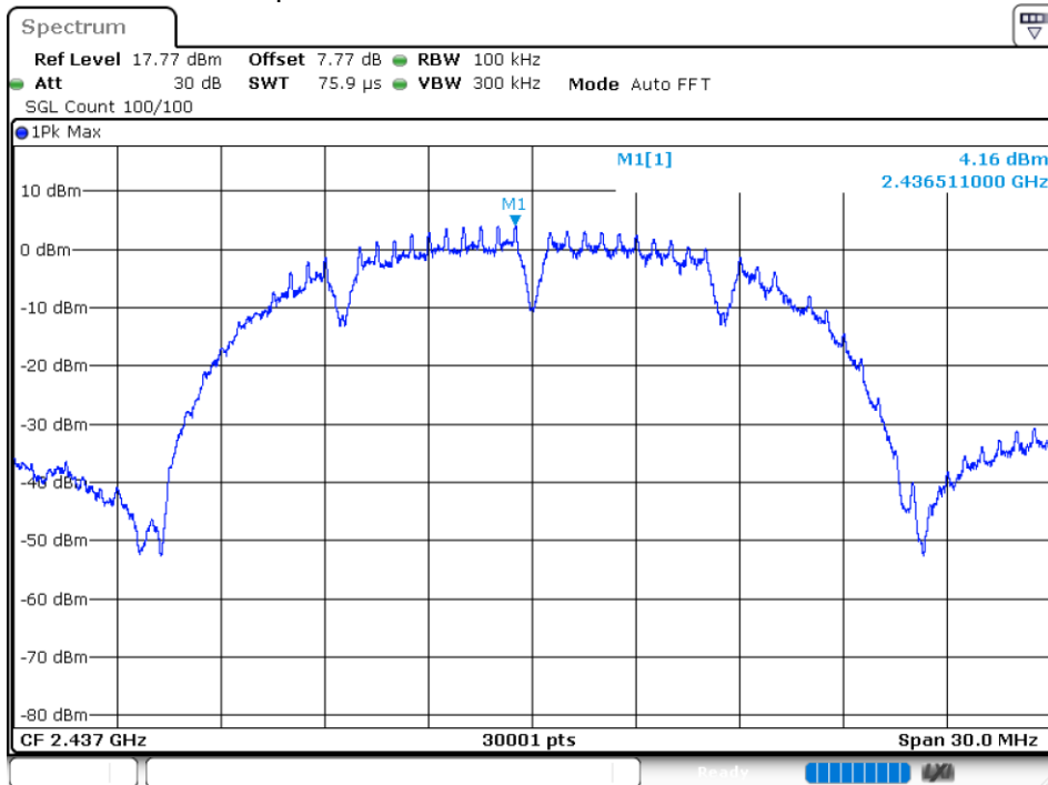
Tx. Spurious NVNT 802.11b 2437MHz Ant1 Emission
