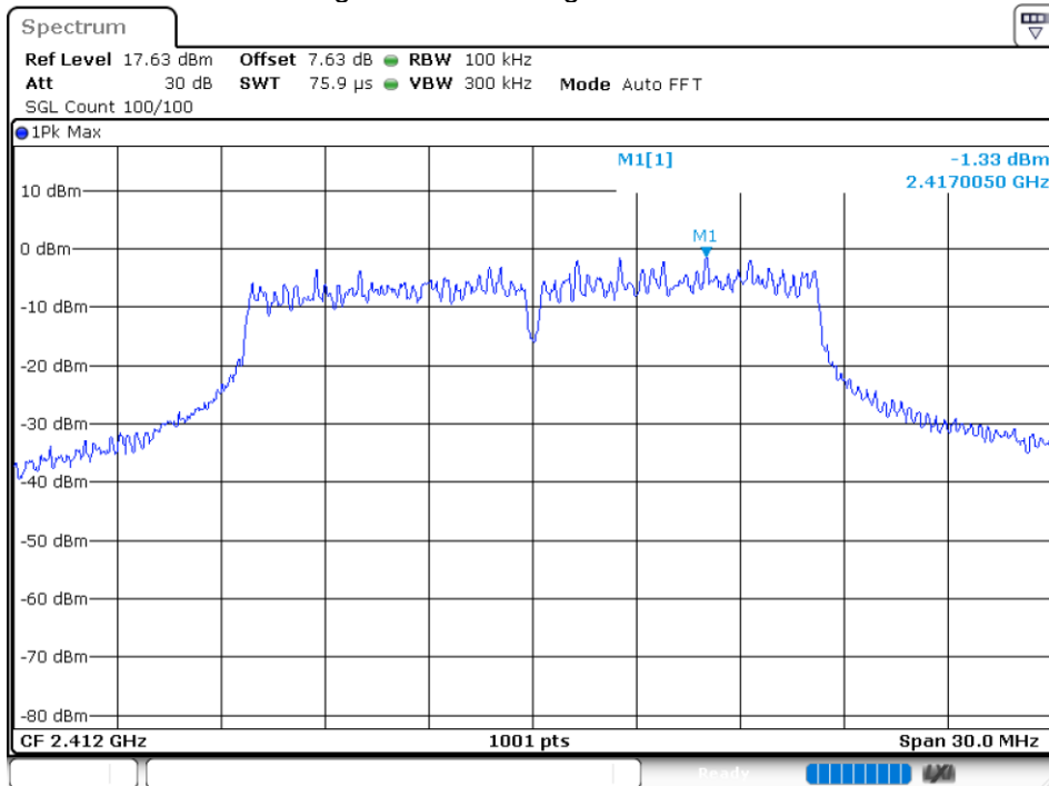
Band Edge NVNT 802.11g 2412MHz Ant1 Emission
