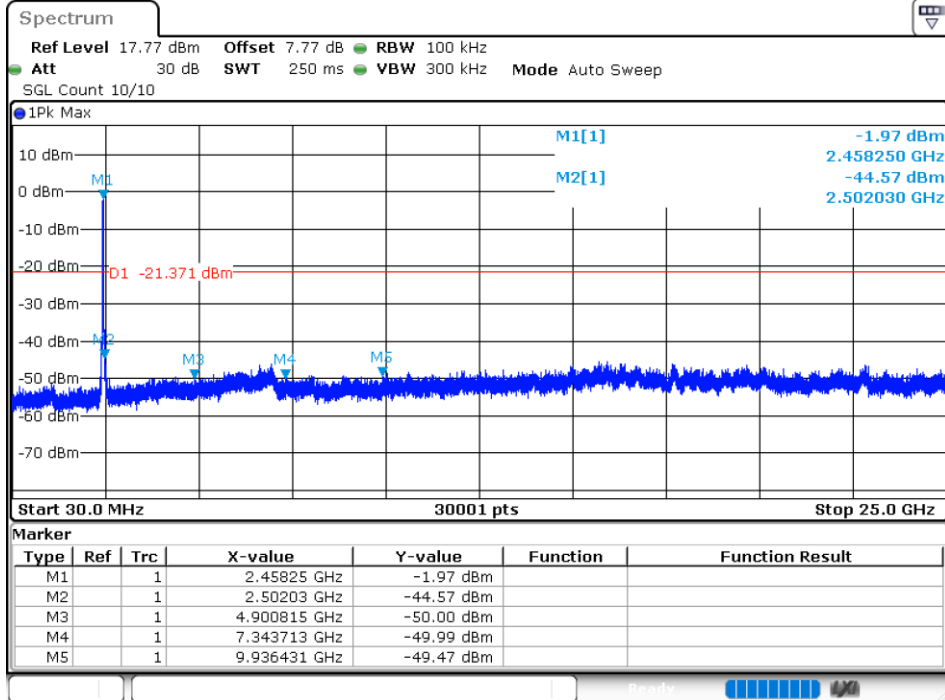
Tx. Spurious NVNT 802.11n(HT40) 2452MHz Ant1 Ref
