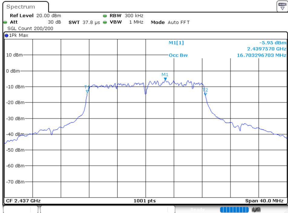
-6 dB BW NVNT 802.11g 2437MHz Ant1
