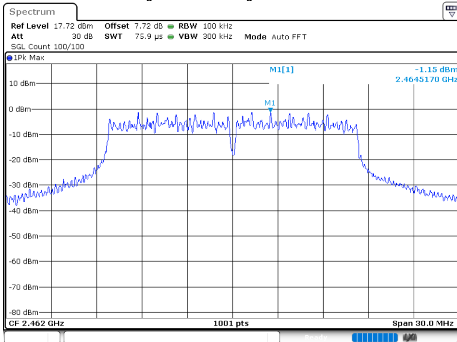
Band Edge NVNT 802.11g 2462MHz Ant1 Emission
