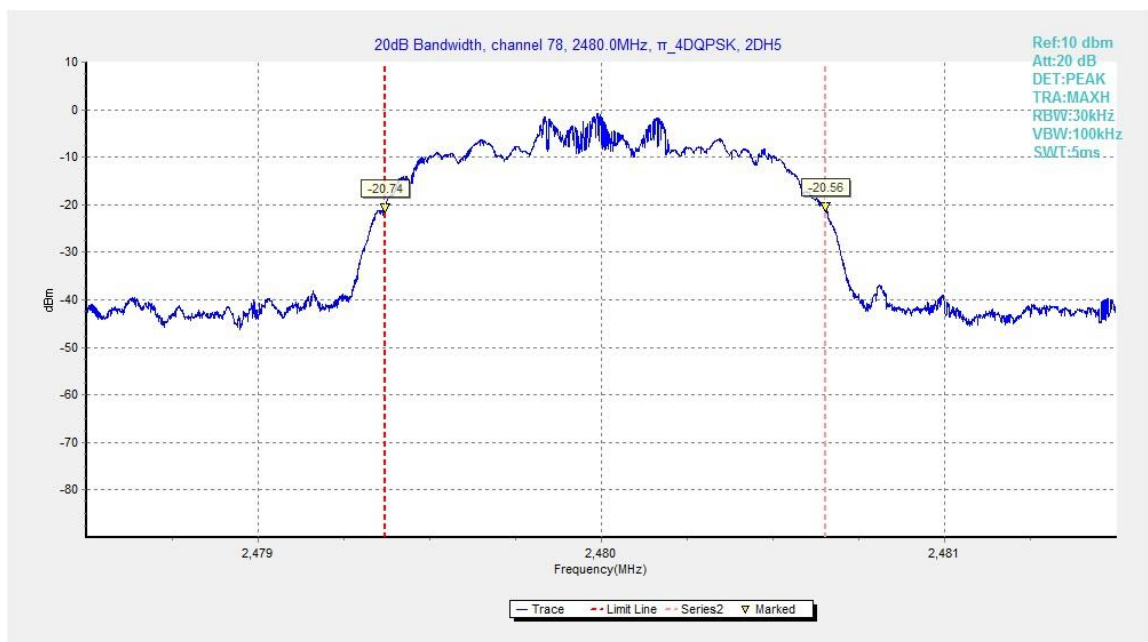
Fig.86. 20dB Bandwidth: \pi/4 DQPSK, Channel 78
