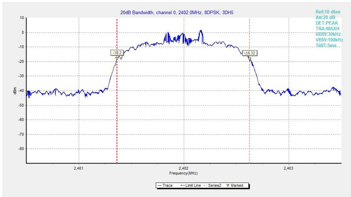
Fig.87. 20dB Bandwidth: 8DPSK, Channel 0
