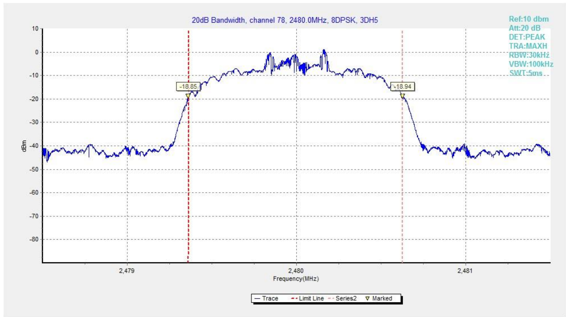
Fig.89. 20dB Bandwidth: 8DPSK, Channel 78
