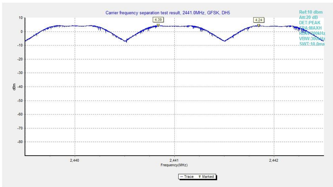
Fig.90. Carrier frequency separation measurement: GFSK, Channel 39
