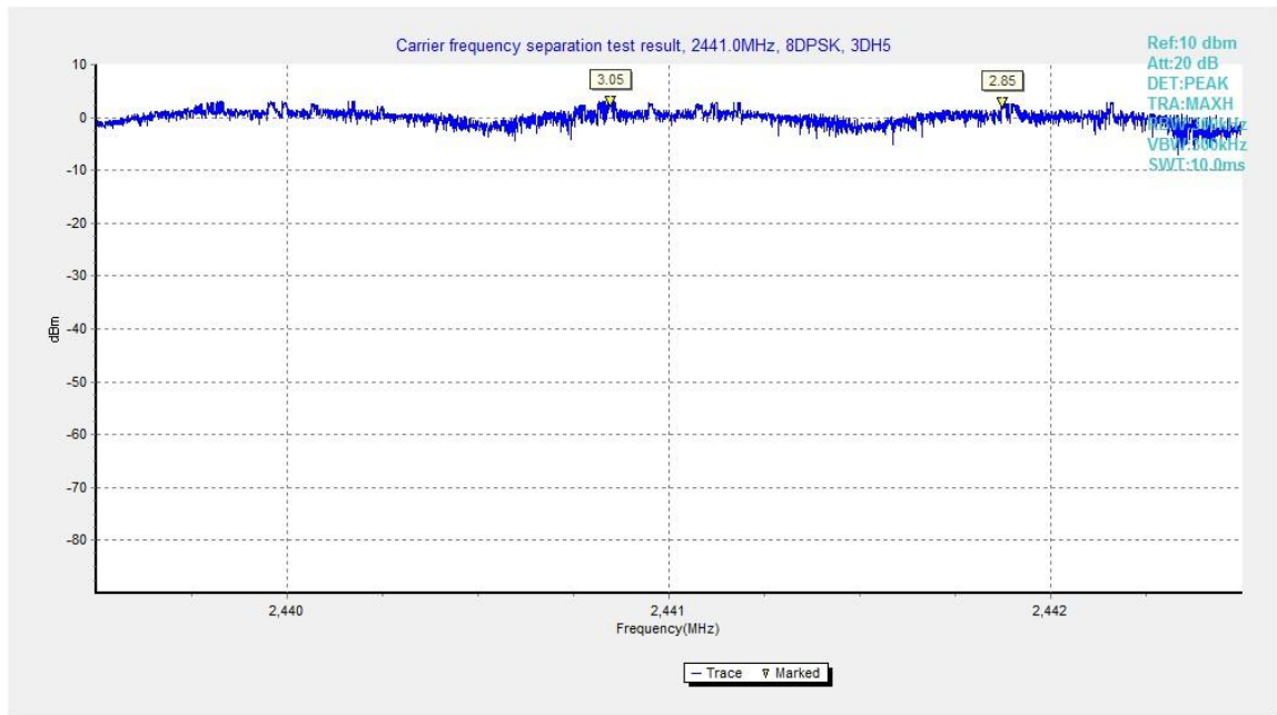
Fig.92. Carrier frequency separation measurement: 8DPSK, Channel 39
