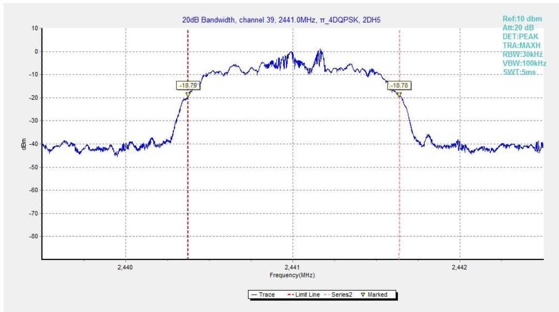
Fig.85. 20dB Bandwidth: \pi/4 DQPSK, Channel 39
