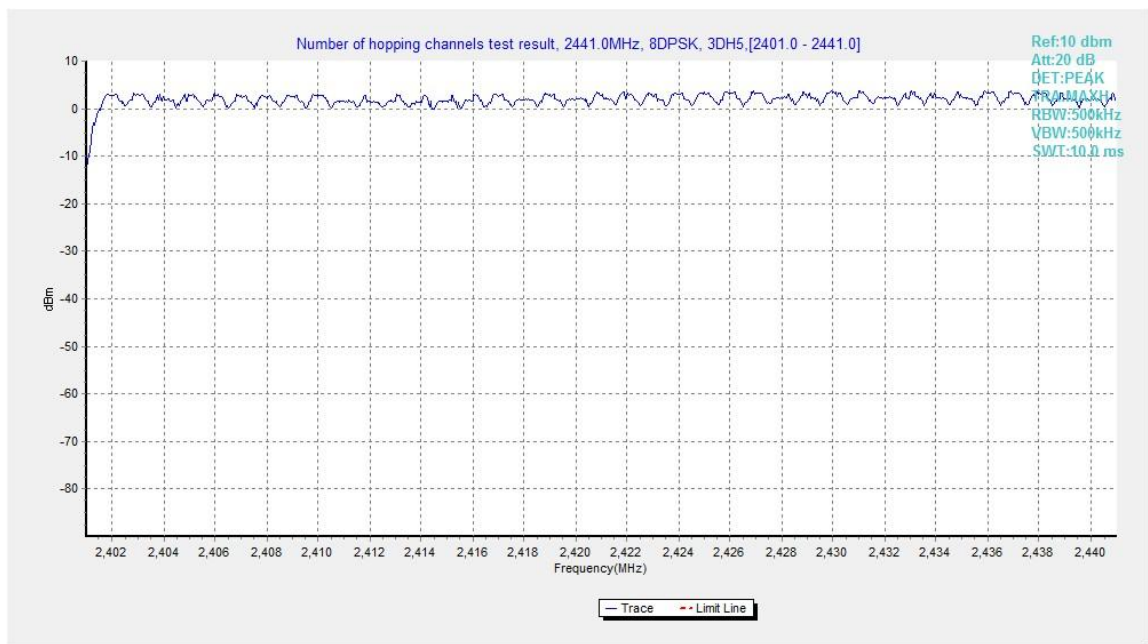
Fig.97. Number of hopping frequencies: 8DPSK, Channel 0 - 39
