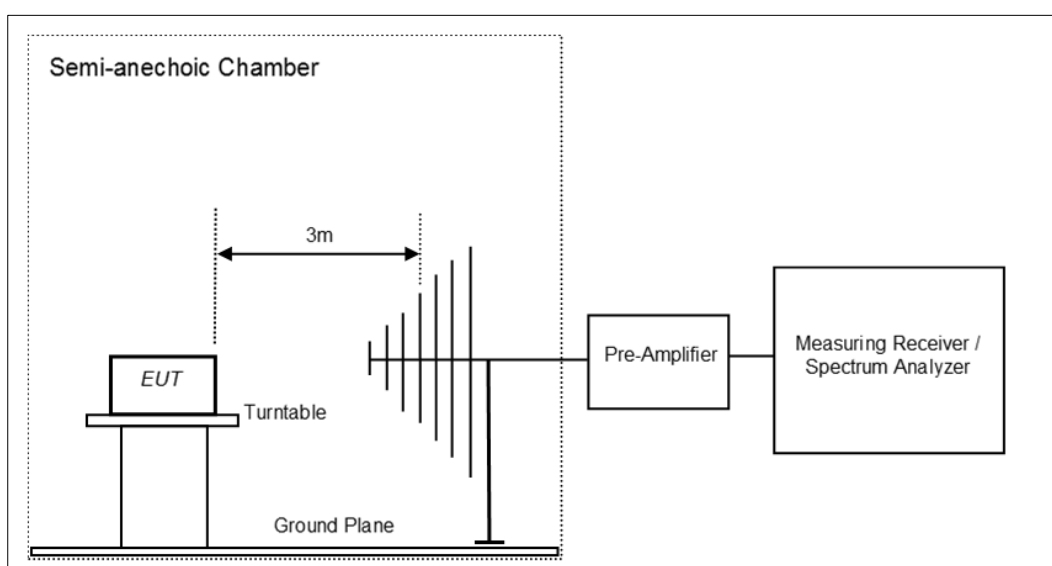
Figure 5: Frequency Range 200 MHz - 1GHz
