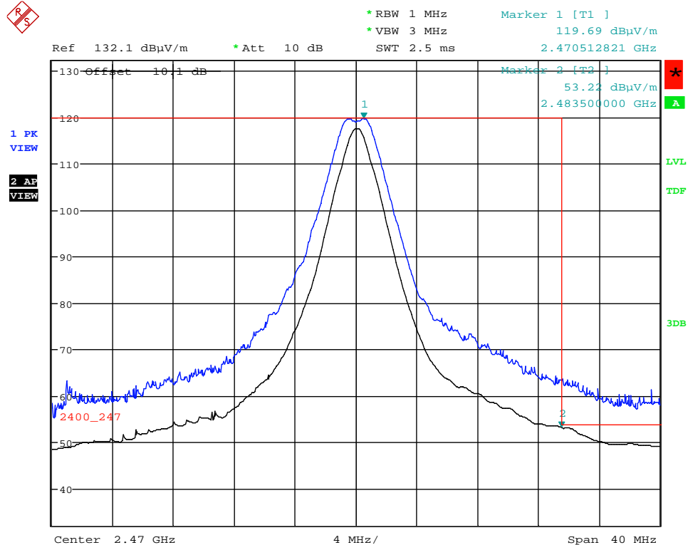
Plot 5.2.4.2.2.5. Band-Edge RF Radiated Emissions at 3 m, Horizontal Polarization Highest End of Frequency Band, Ch24- 2470 MHz, QPSK Modulation, Power -7 Mode 3 @ 66% Duty Cycle
