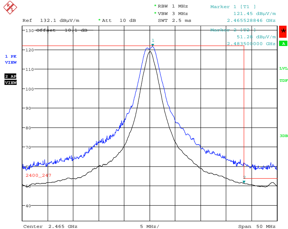
Plot 5.2.4.2.2.4. Band-Edge RF Radiated Emissions at 3 m, Vertical Polarization High End of Frequency Band, Ch23- 2465 MHz, QPSK Modulation, Power -7 Mode 3@ 66% Duty Cycle
