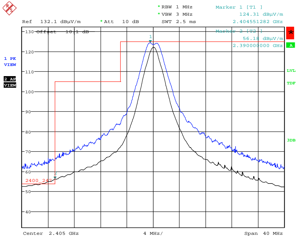
Plot 5.2.4.3.2.2. Band-Edge RF Radiated Emissions at 3 m, Vertical Polarization Low End of Frequency Band, Ch11- 2405 MHz, QPSK Modulation, Power -7 Mode 3 @ 66% Duty Cycle
