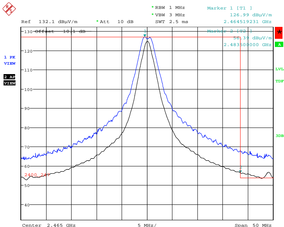
Plot 5.2.4.5.2.3. Band-Edge RF Radiated Emissions at 3 m, Horizontal Polarization Higher End of Frequency Band, Ch23- 2465 MHz, QPSK Modulation, Power -7 Mode 3 @ 66% Duty Cycle
