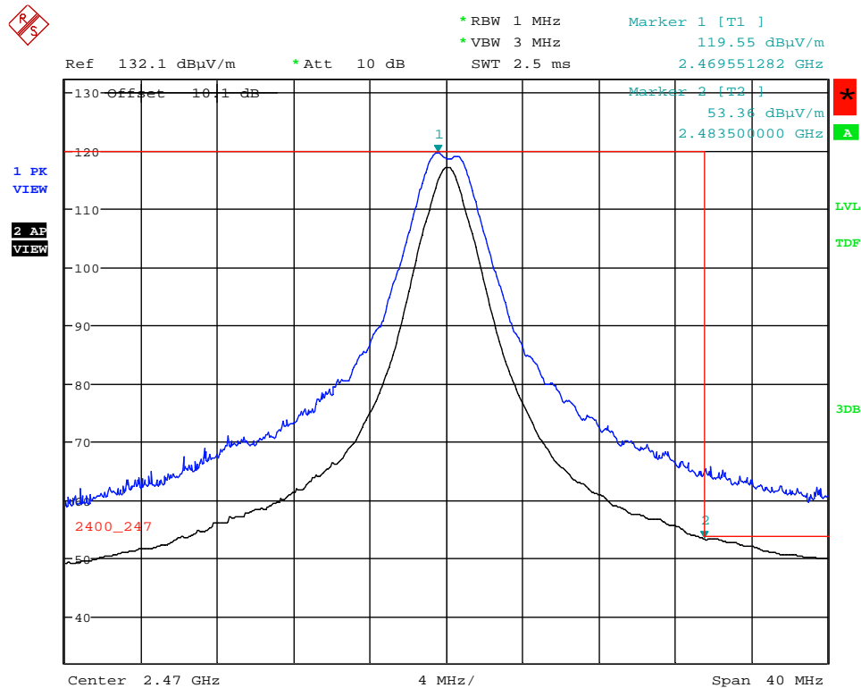
Plot 5.2.4.1.2.5. Band-Edge RF Radiated Emissions at 3 m, Horizontal Polarization Highest End of Frequency Band, Ch24- 2470 MHz, QPSK Modulation, Power -7 Mode 3@ 66% Duty Cycle
