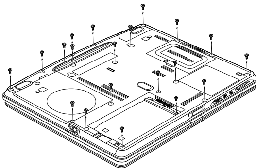
Figure 1 Removing twenty screws
