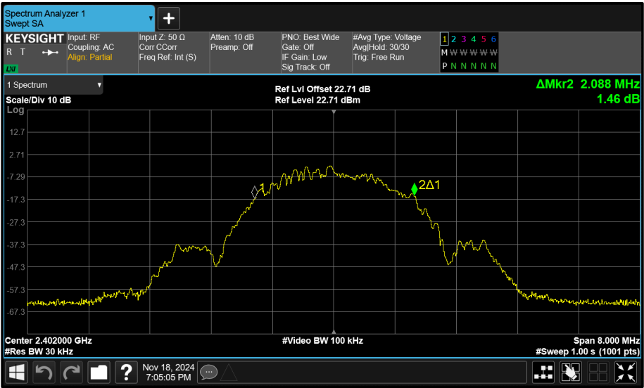
Figure 85 - Core 0 (A) 2402 MHz (CH37) 99% Bandwidth
