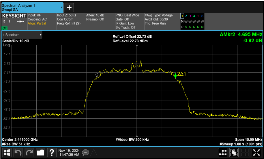
Figure 137 - Core 0 (A) 2441 MHz (CH39) 99% Bandwidth
