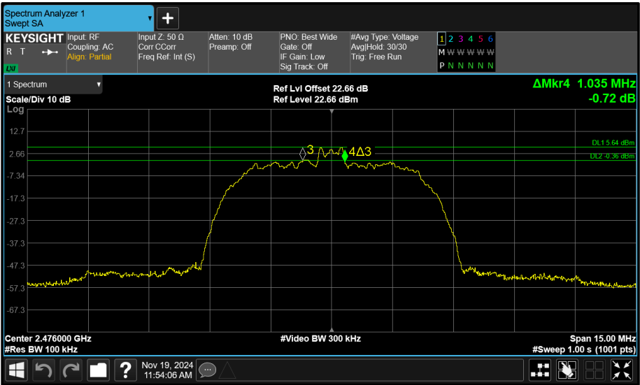
Figure 144 - Core 1 (B) 2476 MHz (CH74) 6 dB Bandwidth
