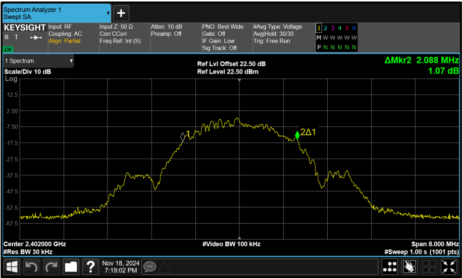
Figure 91 - Core 1 (B) 2402 MHz (CH37) 99% Bandwidth
