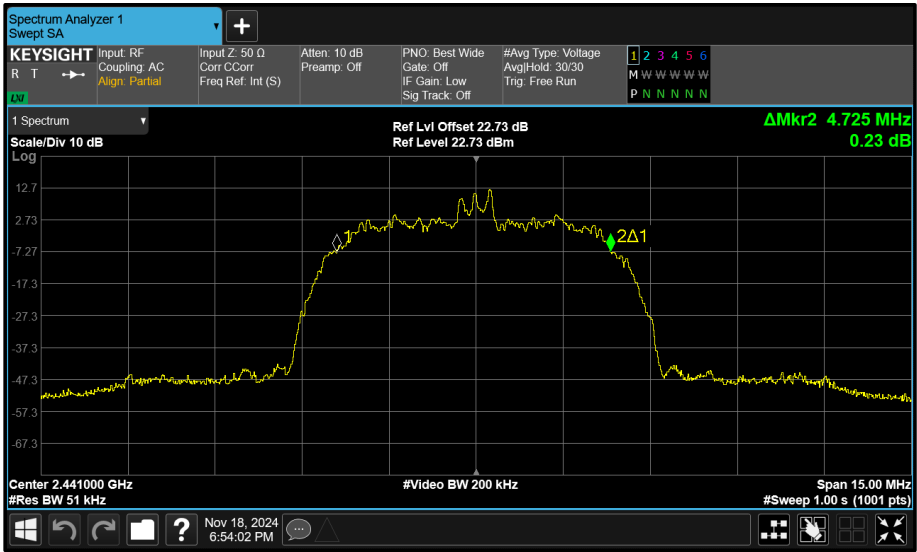
Figure 105 - Core 0 (A) 2441 MHz (CH39) 99% Bandwidth
