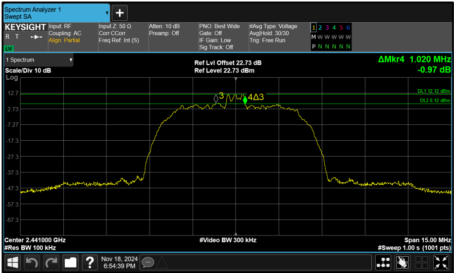
Figure 106 - Core 0 (A) 2441 MHz (CH39) 6 dB Bandwidth
