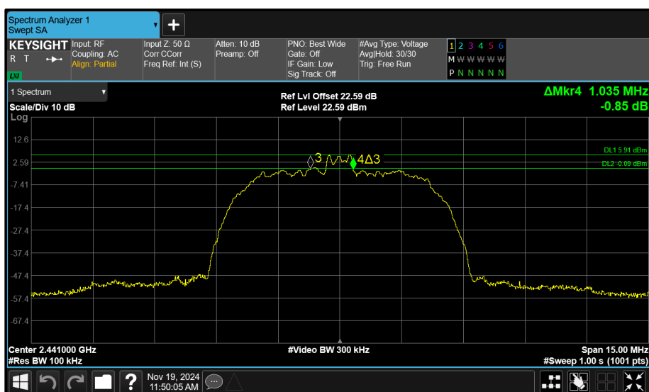
Figure 140 - Core 1 (B) 2441 MHz (CH39) 6 dB Bandwidth
