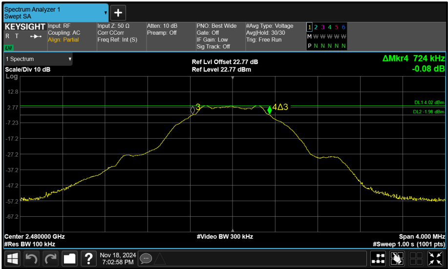
Figure 78 - Core 0 (A) 2480 MHz (CH39) 6 dB Bandwidth
