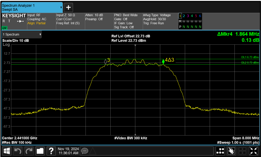
Figure 126 - Core 0 (A) 2441 MHz (CH39) 6 dB Bandwidth
