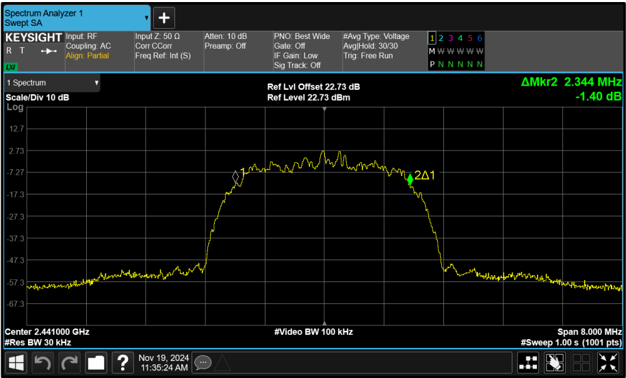
Figure 125 - Core 0 (A) 2441 MHz (CH39) 99% Bandwidth
