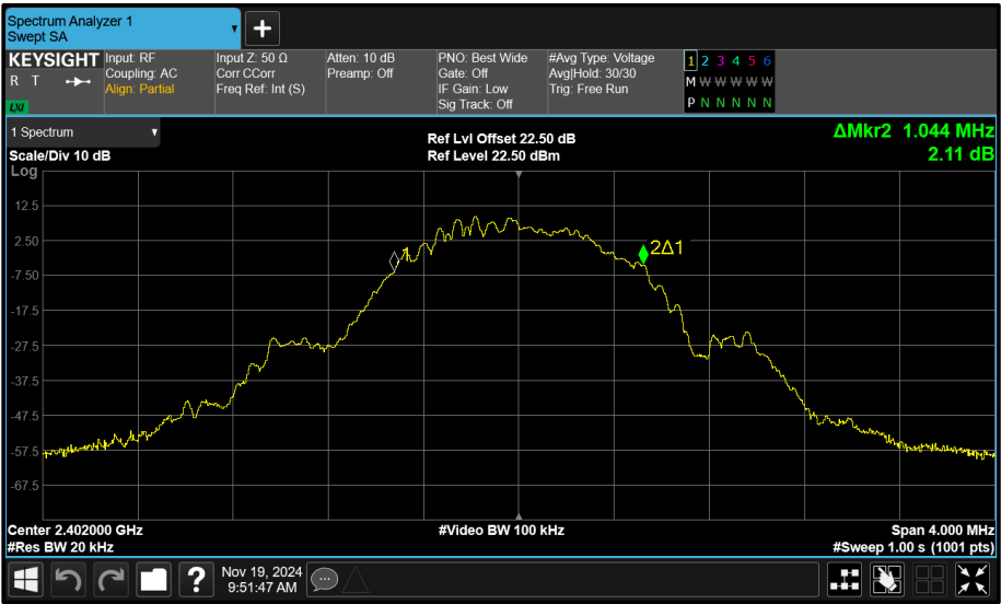
Figure 109 - Core 1 (B) 2402 MHz (CH37) 99% Bandwidth
