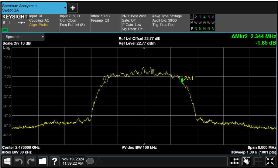
Figure 129 - Core 0 (A) 2476 MHz (CH74) 99% Bandwidth
