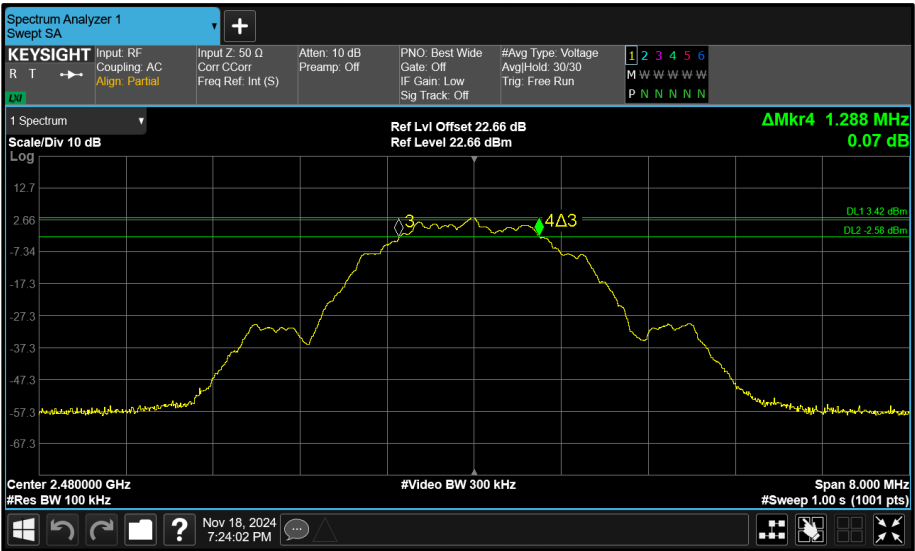
Figure 96 - Core 1 (B) 2480 MHz (CH39) 6 dB Bandwidth
