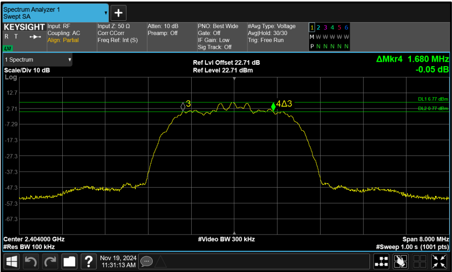
Figure 122 - Core 0 (A) 2404 MHz (CH2) 6 dB Bandwidth
