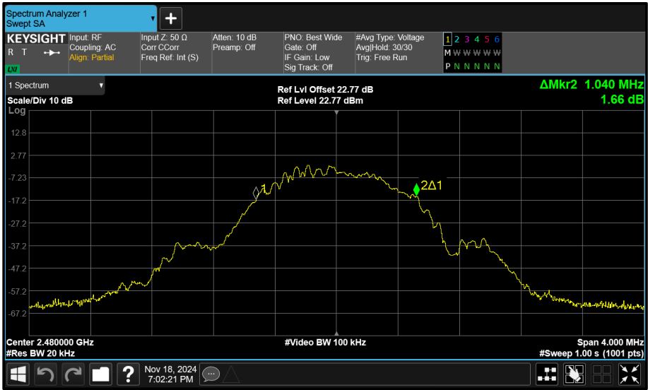
Figure 77 - Core 0 (A) 2480 MHz (CH39) 99% Bandwidth
