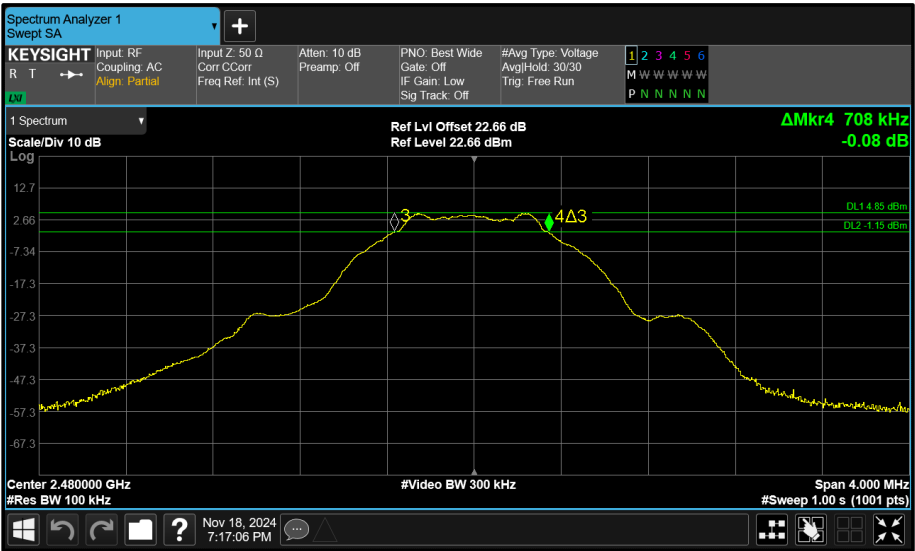
Figure 84 - Core 1 (B) 2480 MHz (CH39) 6 dB Bandwidth
