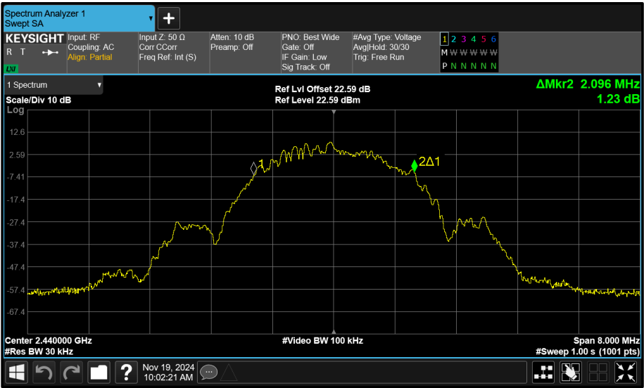
Figure 117 - Core 1 (B) 2440 MHz (CH17) 99% Bandwidth
