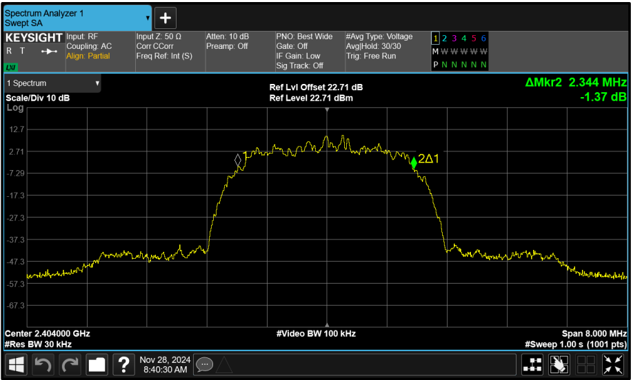
Figure 97 - Core 0 (A) 2404 MHz (CH2) 99% Bandwidth
