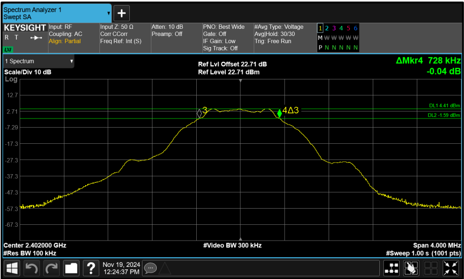
Figure 146 - Core 0 (A) 2402 MHz (CH37) 6 dB Bandwidth
