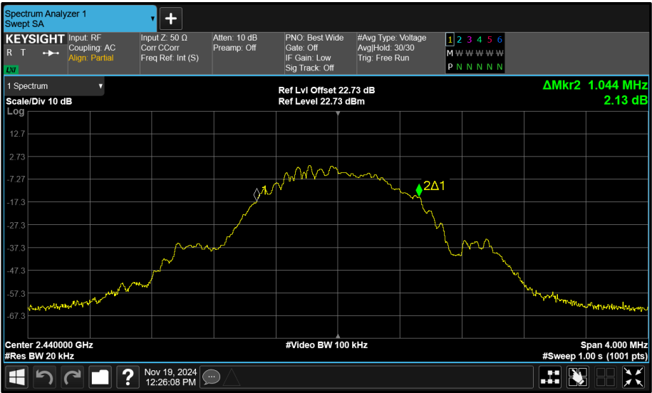
Figure 149 - Core 0 (A) 2440 MHz (CH17) 99% Bandwidth
