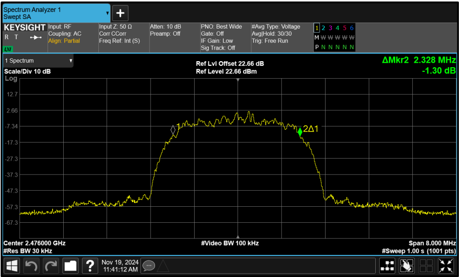
Figure 131 - Core 1 (B) 2476 MHz (CH74) 99% Bandwidth
