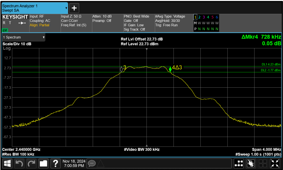
Figure 76 - Core 0 (A) 2440 MHz (CH17) 6 dB Bandwidth
