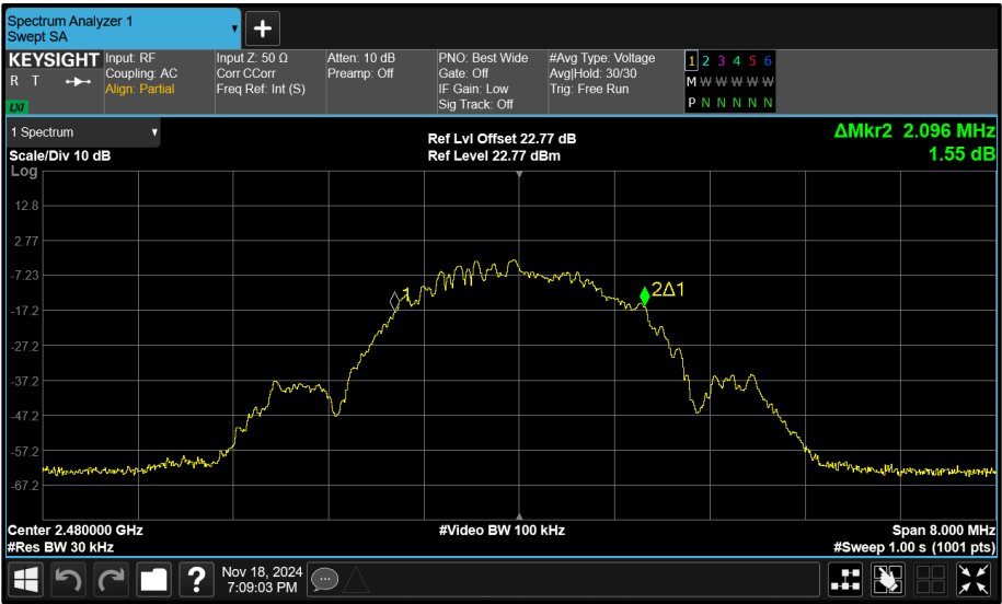
Figure 89 - Core 0 (A) 2480 MHz (CH39) 99% Bandwidth
