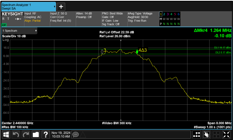
Figure 118 - Core 1 (B) 2440 MHz (CH17) 6 dB Bandwidth
