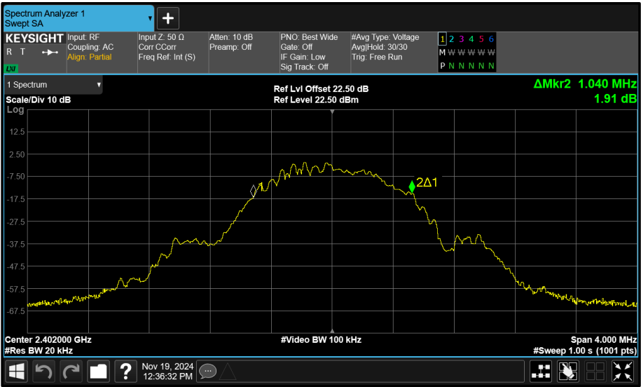
Figure 147 - Core 1 (B) 2402 MHz (CH37) 99% Bandwidth
