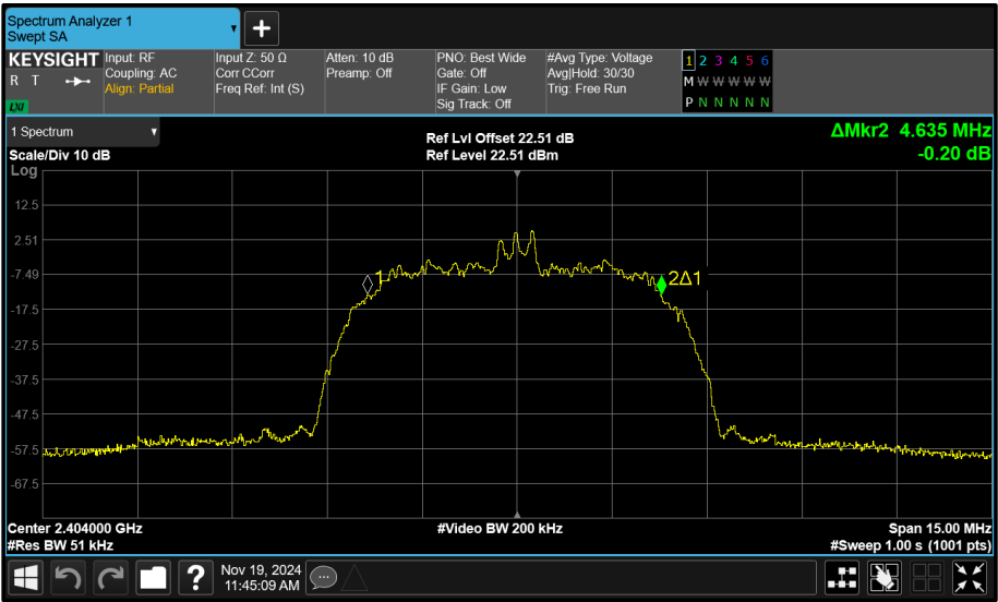
Figure 135 - Core 1 (B) 2404 MHz (CH2) 99% Bandwidth
