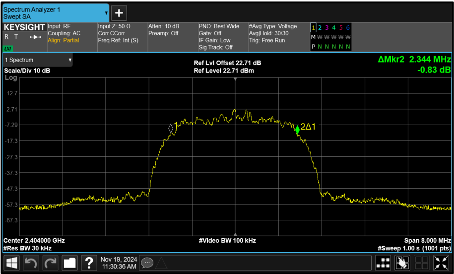
Figure 121 - Core 0 (A) 2404 MHz (CH2) 99% Bandwidth
