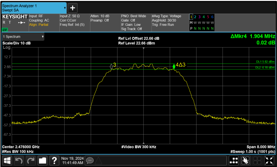
Figure 132 - Core 1 (B) 2476 MHz (CH74) 6 dB Bandwidth
