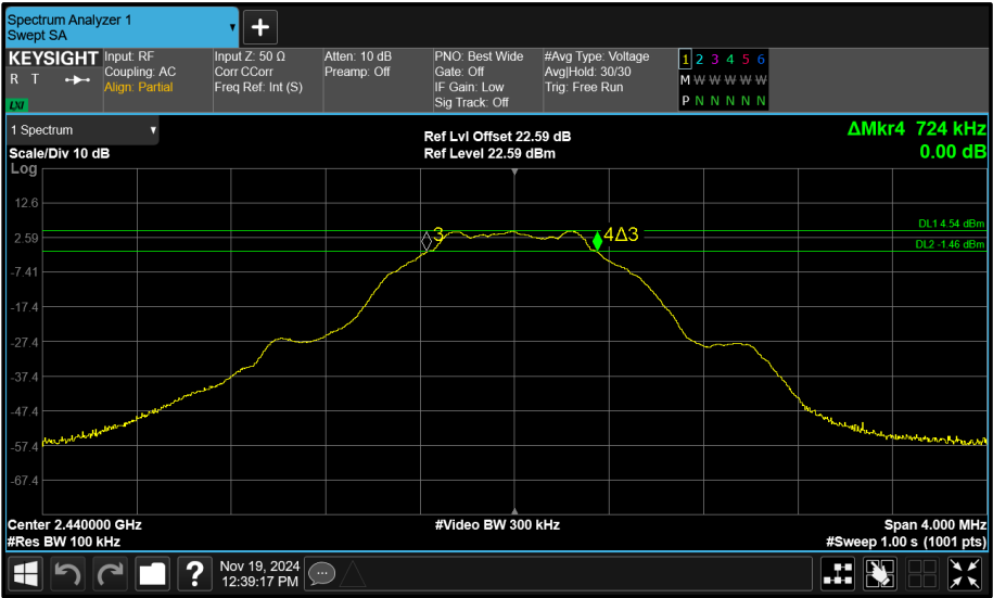
Figure 152 - Core 1 (B) 2440 MHz (CH17) 6 dB Bandwidth
