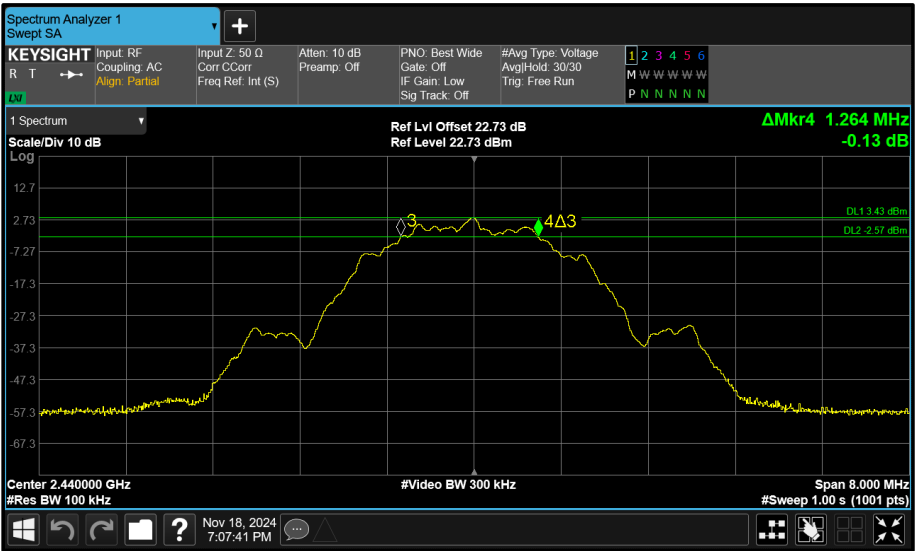
Figure 88 - Core 0 (A) 2440 MHz (CH17) 6 dB Bandwidth
