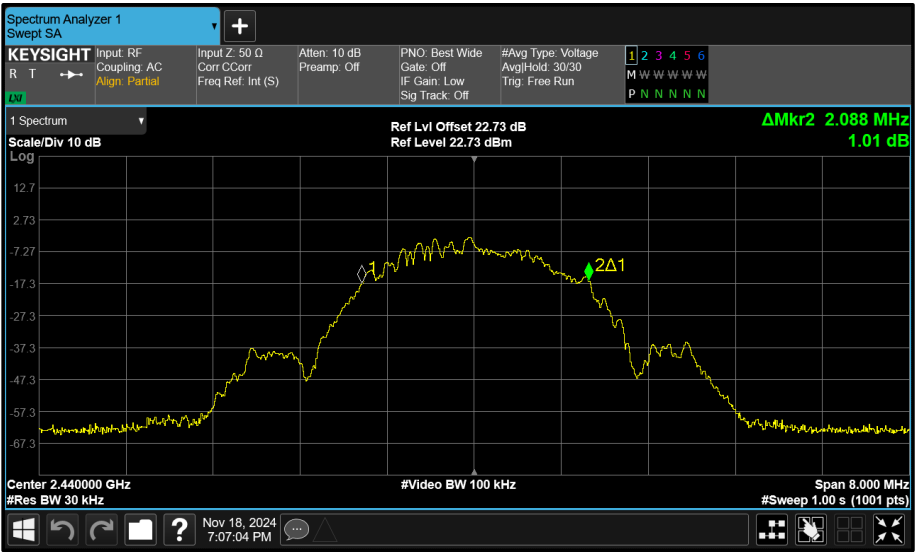
Figure 87 - Core 0 (A) 2440 MHz (CH17) 99% Bandwidth
