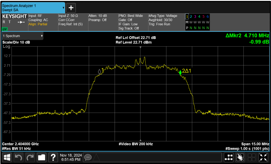
Figure 103 - Core 0 (A) 2404 MHz (CH2) 99% Bandwidth
