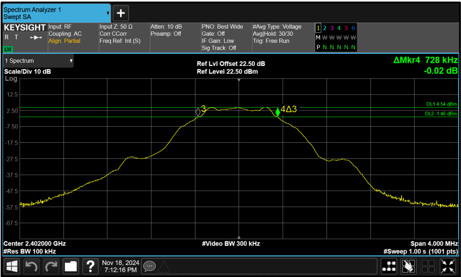
Figure 80 - Core 1 (B) 2402 MHz (CH37) 6 dB Bandwidth
