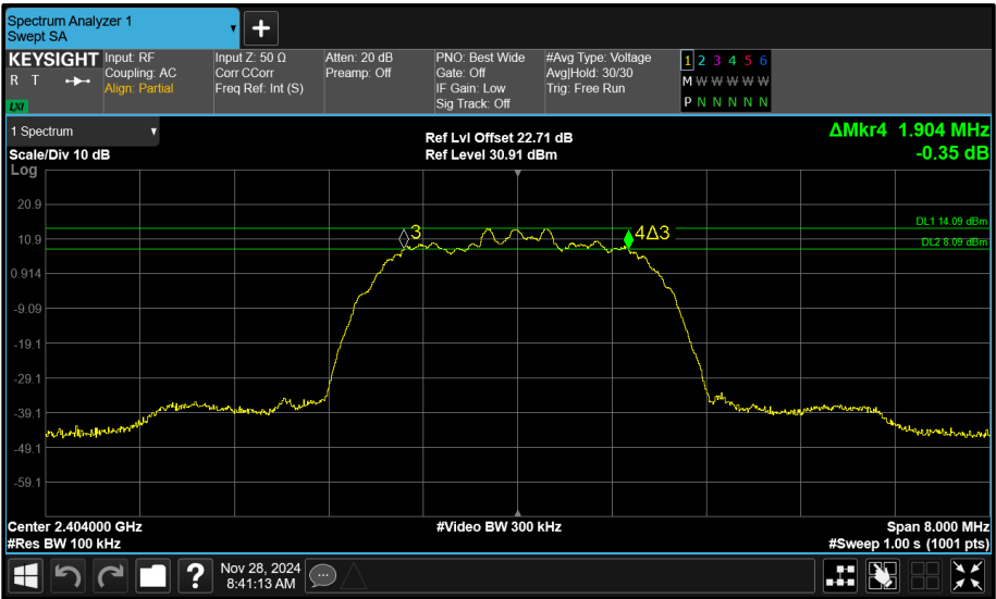
Figure 98 - Core 0 (A) 2404 MHz (CH2) 6 dB Bandwidth
