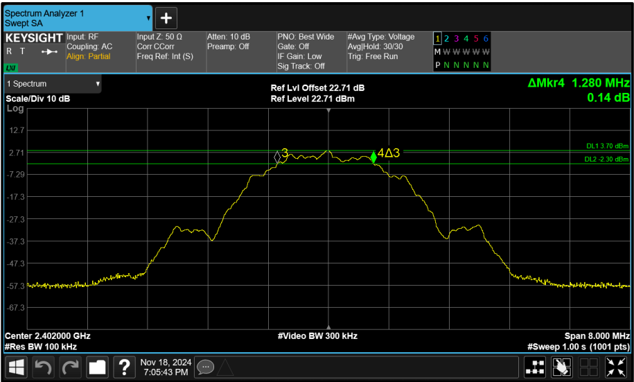
Figure 86 - Core 0 (A) 2402 MHz (CH37) 6 dB Bandwidth
