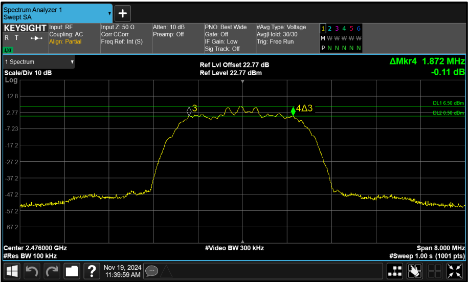
Figure 130 - Core 0 (A) 2476 MHz (CH74) 6 dB Bandwidth
