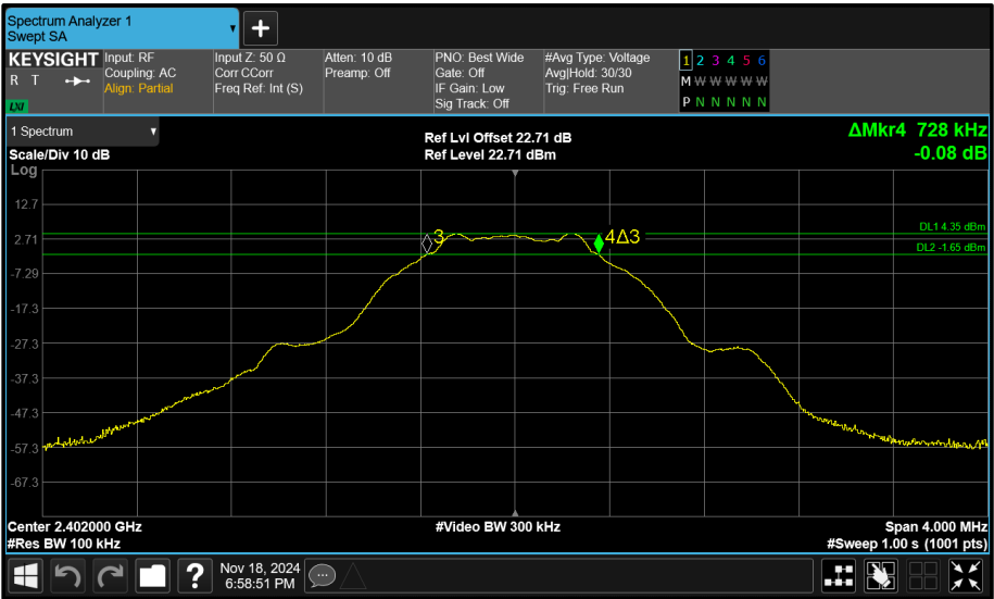
Figure 74 - Core 0 (A) 2402 MHz (CH37) 6 dB Bandwidth
