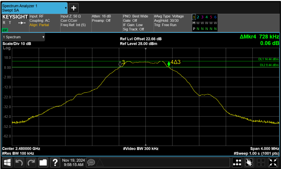
Figure 114 - Core 1 (B) 2480 MHz (CH39) 6 dB Bandwidth
