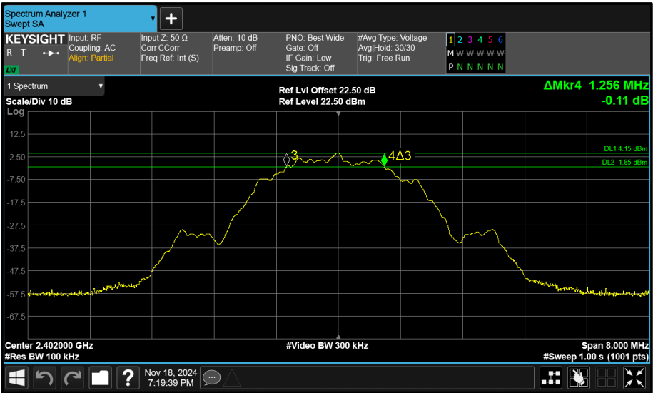
Figure 92 - Core 1 (B) 2402 MHz (CH37) 6 dB Bandwidth
