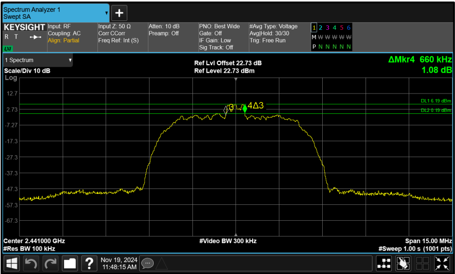
Figure 138 - Core 0 (A) 2441 MHz (CH39) 6 dB Bandwidth
