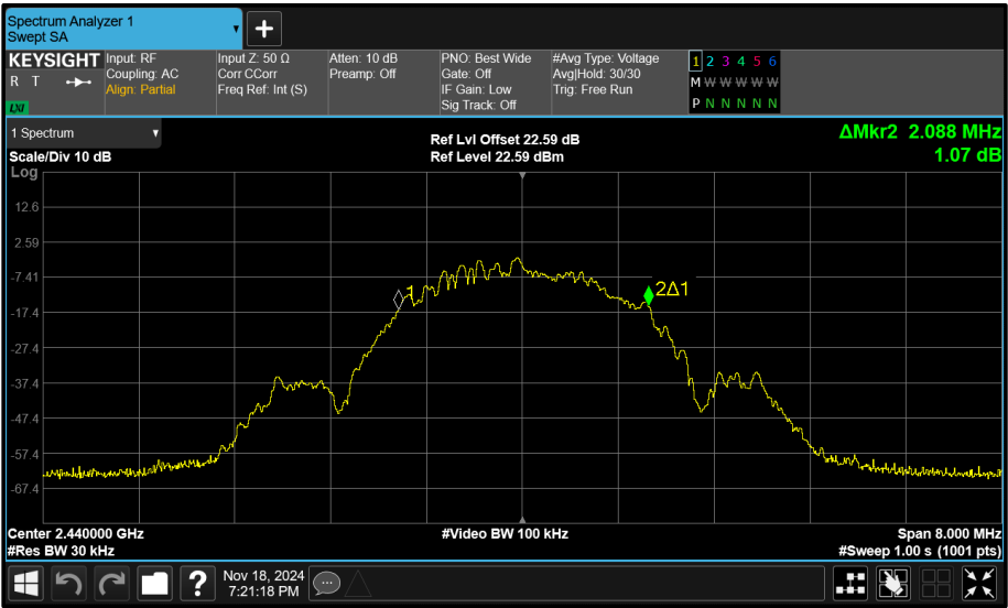
Figure 93 - Core 1 (B) 2440 MHz (CH17) 99% Bandwidth
