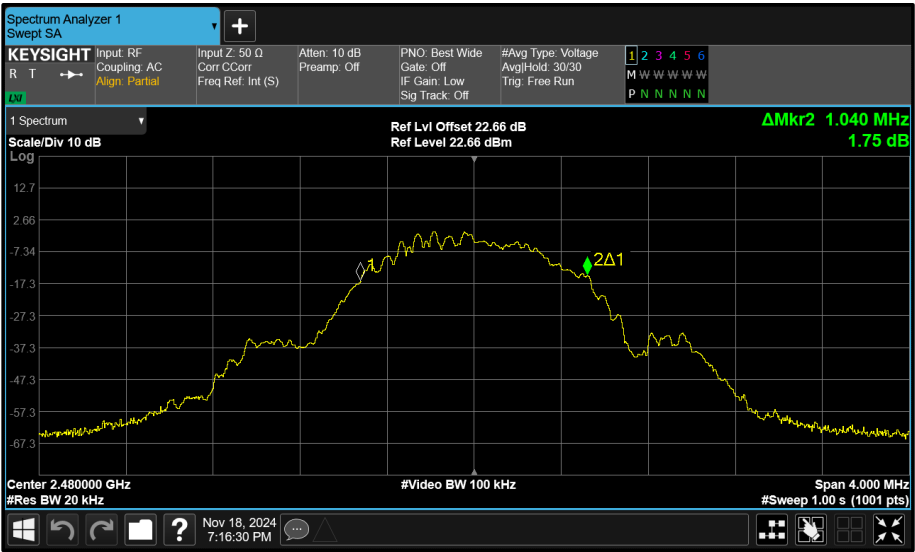
Figure 83 - Core 1 (B) 2480 MHz (CH39) 99% Bandwidth
