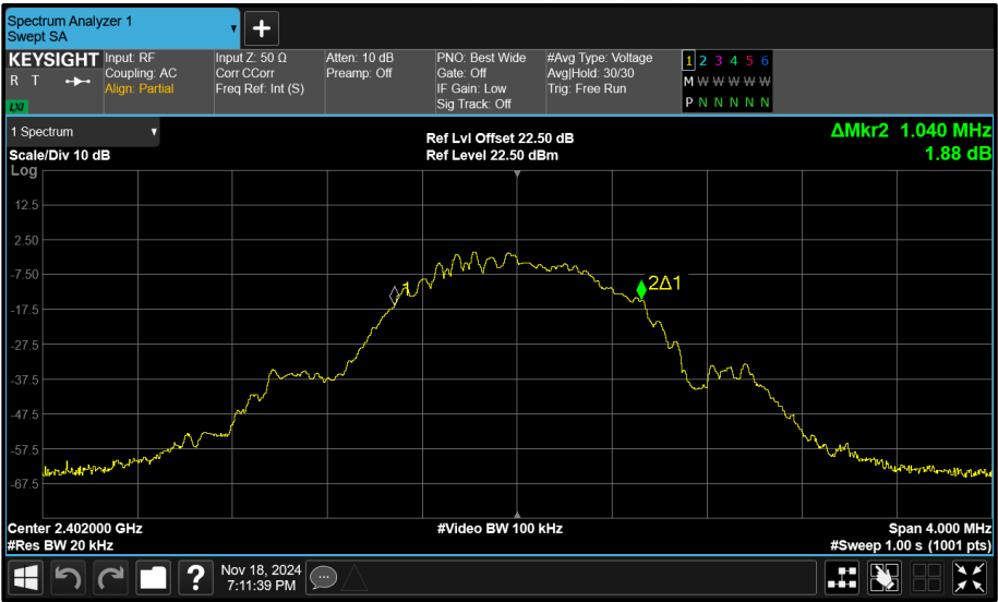
Figure 79 - Core 1 (B) 2402 MHz (CH37) 99% Bandwidth
