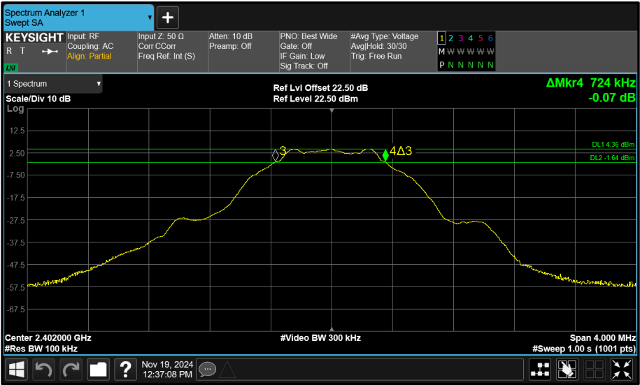
Figure 148 - Core 1 (B) 2402 MHz (CH37) 6 dB Bandwidth
