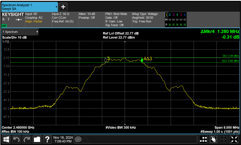
Figure 90 - Core 0 (A) 2480 MHz (CH39) 6 dB Bandwidth
