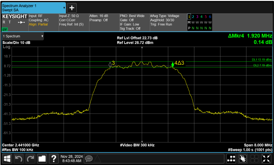
Figure 100 - Core 0 (A) 2441 MHz (CH39) 6 dB Bandwidth
