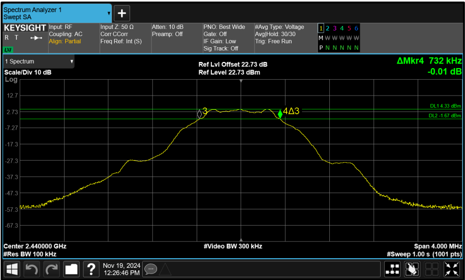
Figure 150 - Core 0 (A) 2440 MHz (CH17) 6 dB Bandwidth
