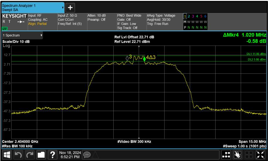
Figure 104 - Core 0 (A) 2404 MHz (CH2) 6 dB Bandwidth
