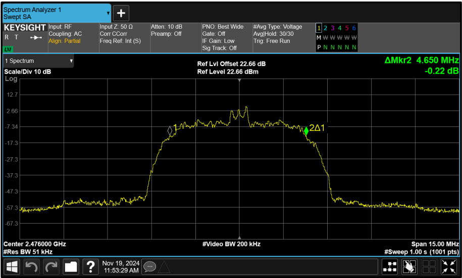
Figure 143 - Core 1 (B) 2476 MHz (CH74) 99% Bandwidth
