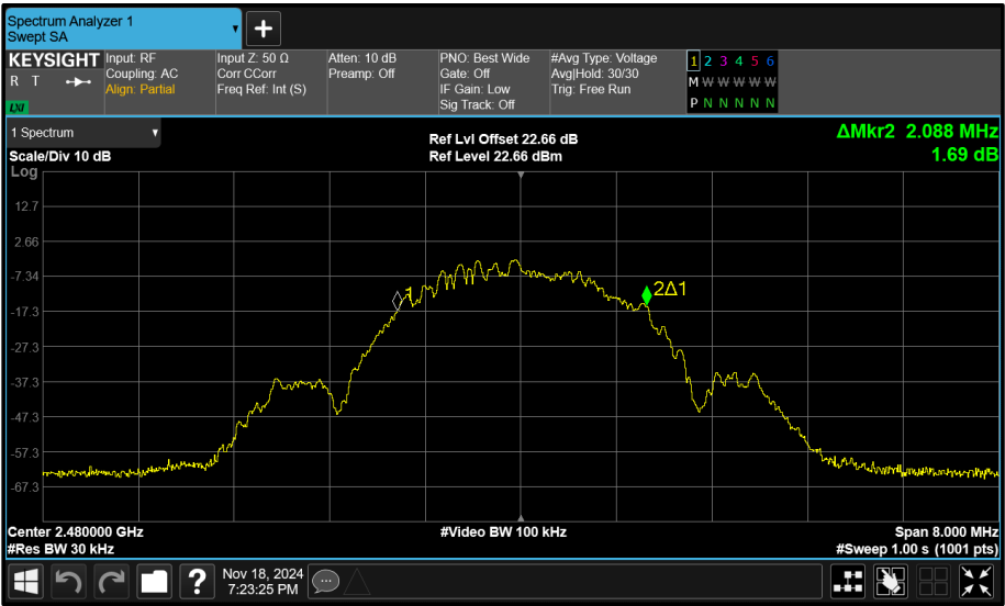
Figure 95 - Core 1 (B) 2480 MHz (CH39) 99% Bandwidth
