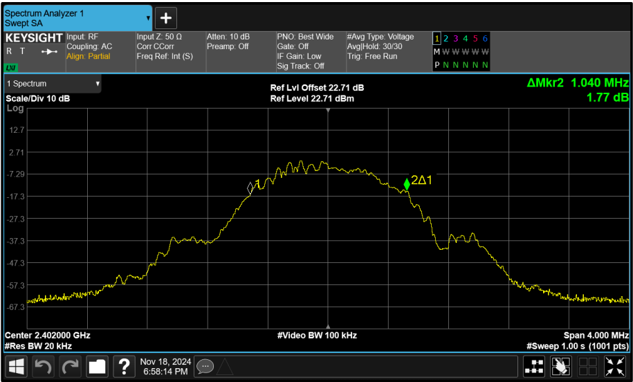
Figure 73 - Core 0 (A) 2402 MHz (CH37) 99% Bandwidth
