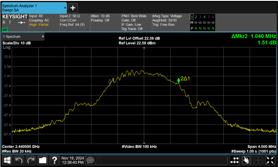
Figure 151 - Core 1 (B) 2440 MHz (CH17) 99% Bandwidth
