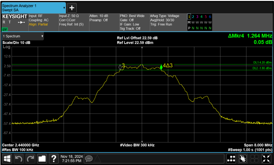
Figure 94 - Core 1 (B) 2440 MHz (CH17) 6 dB Bandwidth
