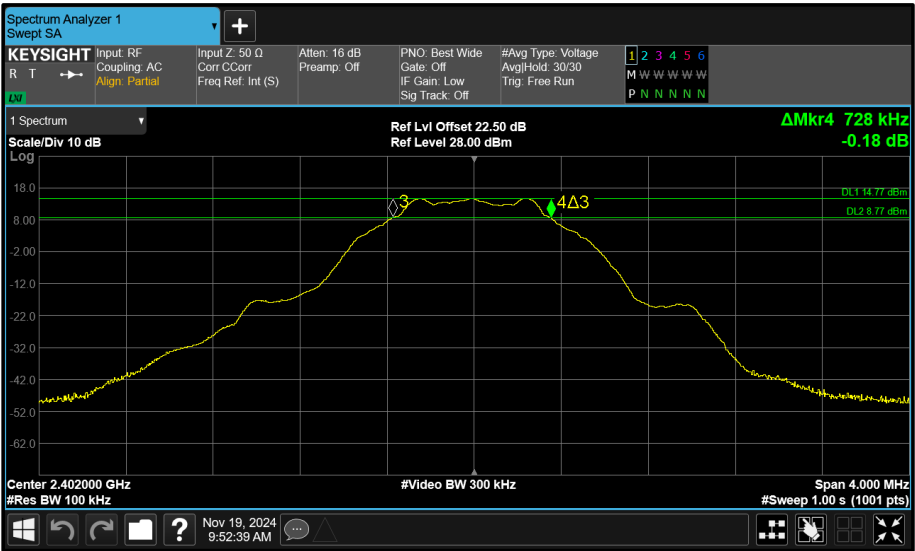
Figure 110 - Core 1 (B) 2402 MHz (CH37) 6 dB Bandwidth
