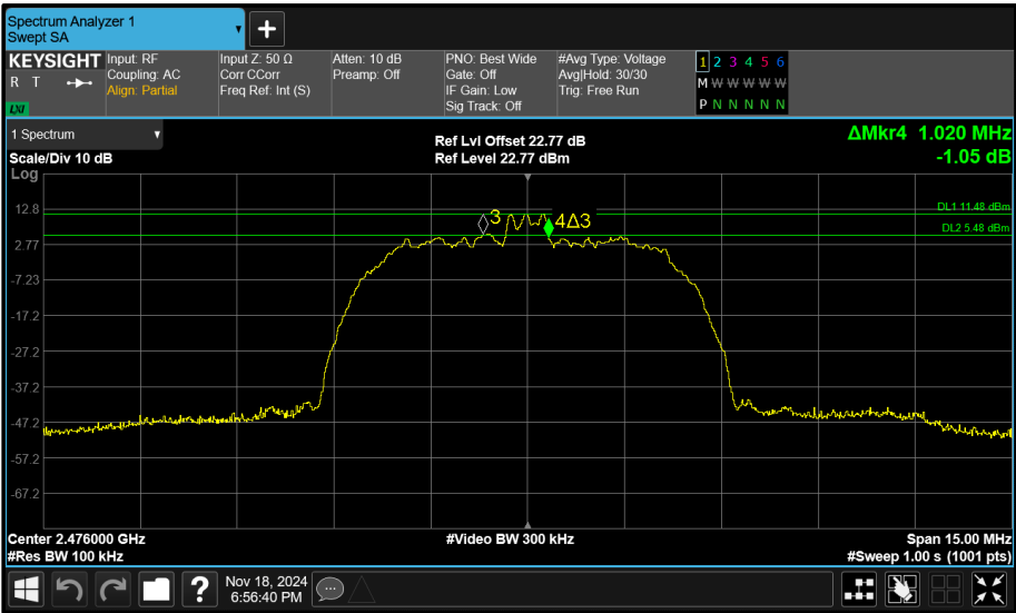
Figure 108 - Core 0 (A) 2476 MHz (CH74) 6 dB Bandwidth
