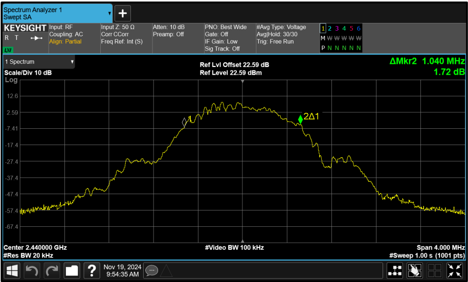
Figure 111 - Core 1 (B) 2440 MHz (CH17) 99% Bandwidth
