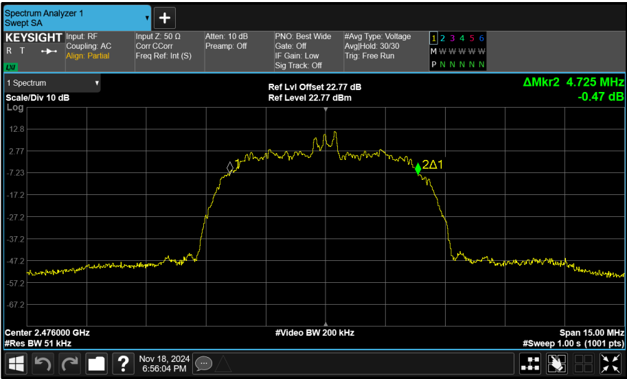
Figure 107 - Core 0 (A) 2476 MHz (CH74) 99% Bandwidth
