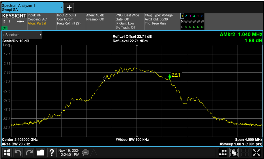
Figure 145 - Core 0 (A) 2402 MHz (CH37) 99% Bandwidth
