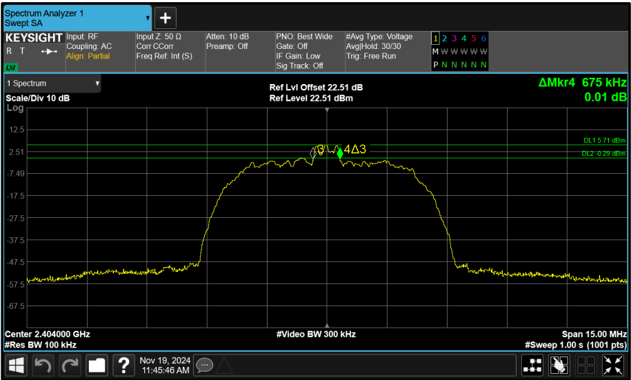
Figure 136 - Core 1 (B) 2404 MHz (CH2) 6 dB Bandwidth
