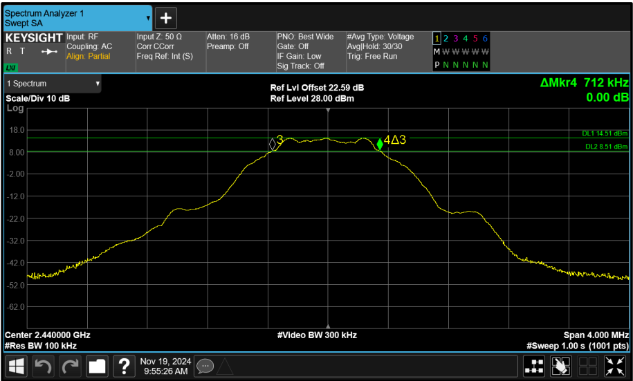
Figure 112 - Core 1 (B) 2440 MHz (CH17) 6 dB Bandwidth
