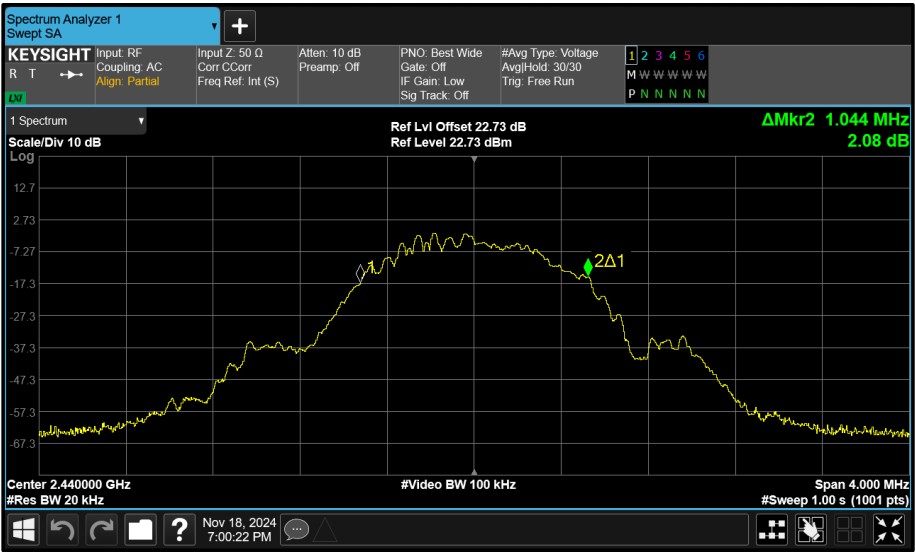
Figure 75 - Core 0 (A) 2440 MHz (CH17) 99% Bandwidth
