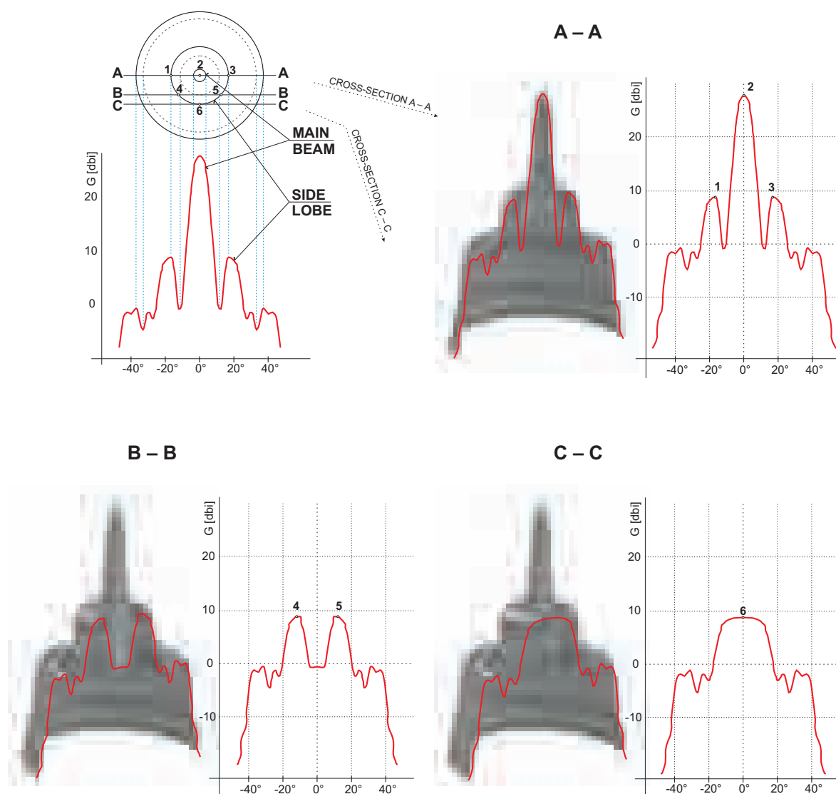
Fig. 6.43: Radiation diagrams
