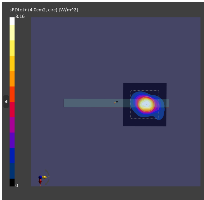
Figure D-2 4cm 2 -averaged power density distribution measured at input.power.limit of 8.6 dBm on the Right Surface n261 beam ID 12.
