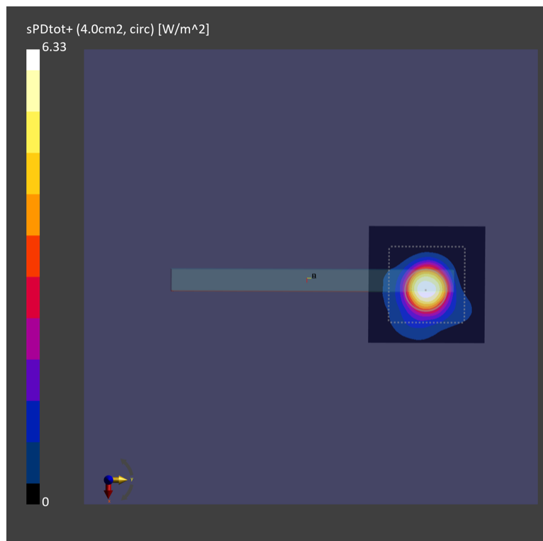
Figure D-3 4cm 2 -averaged power density distribution measured at input.power.limit of 13.2 dBm on the Right Surface n261 beam ID 4.
